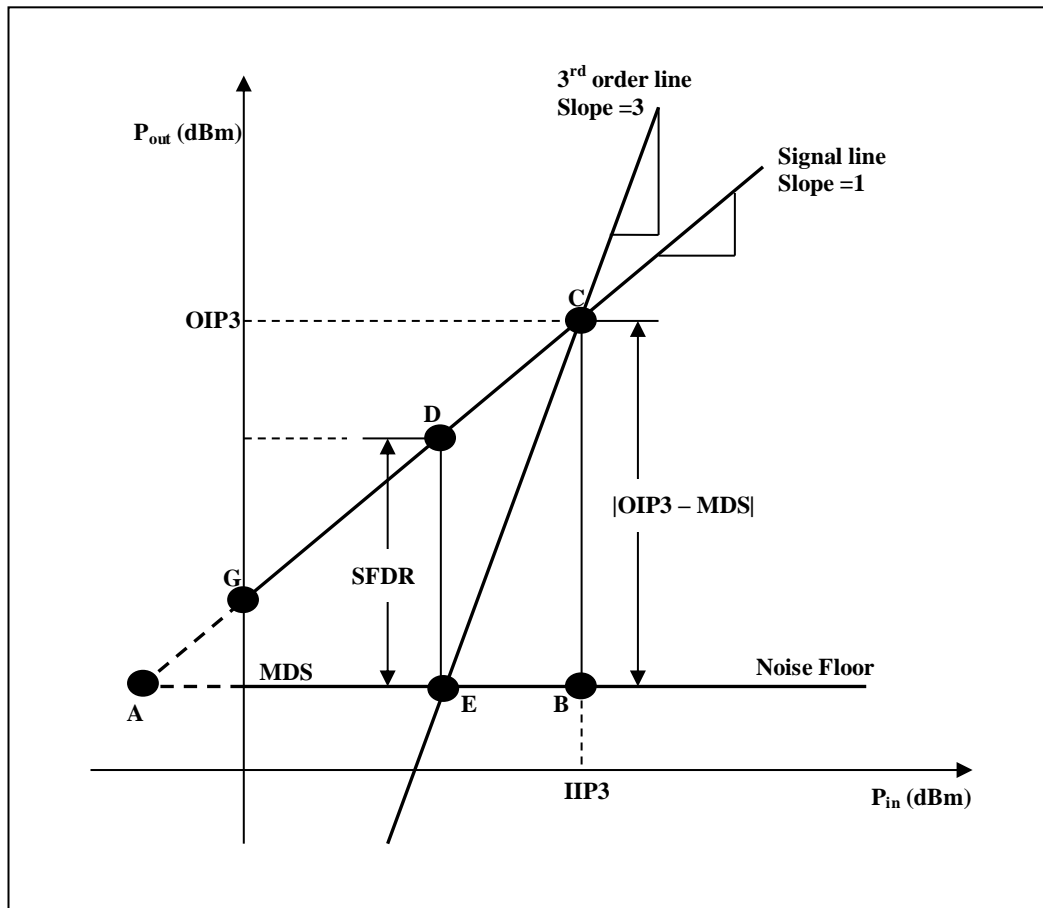
Figure-5 Graphical Representation of SFDR
