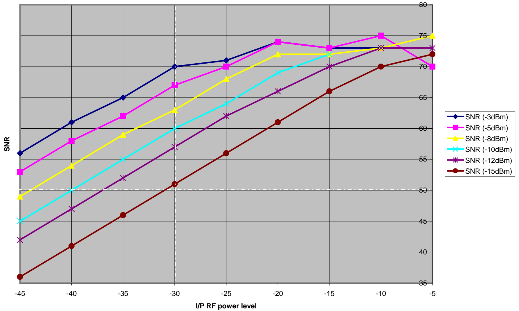
RF input level Vs SNR
