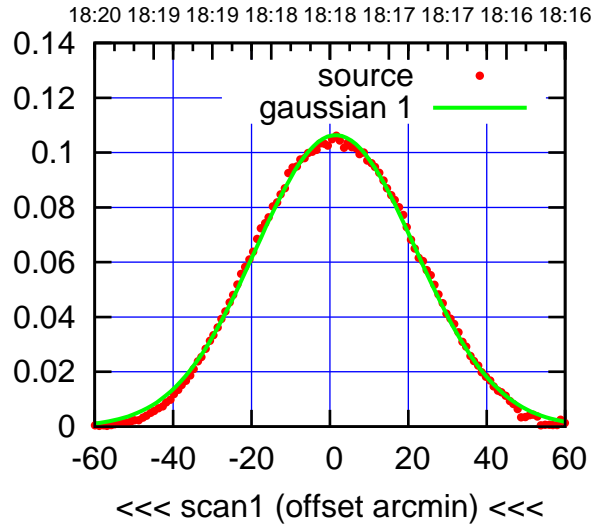
C13-175-AZ OFF= 2.7'
