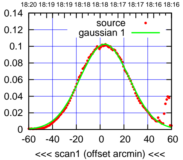
C12-175-AZ OFF= 4.3'
