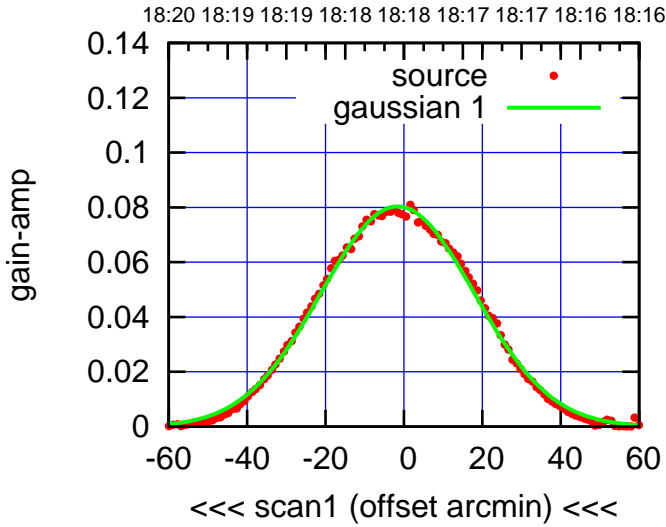
E05-130-AZ OFF= -0.8'
