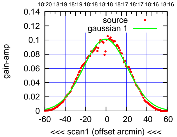
S03-175-AZ OFF= -4.4'
