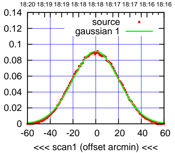
S06-175-AZ OFF= 0.8'
