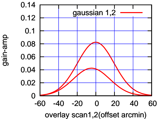
BACKLASH ERROR= 4.8'
