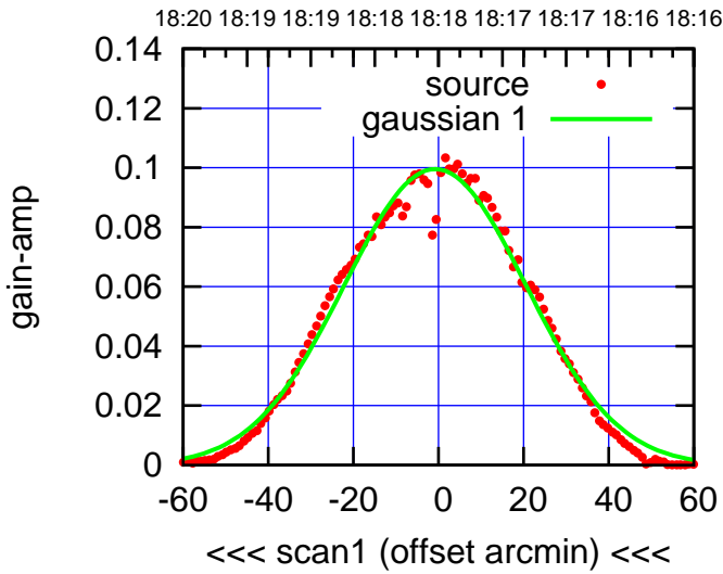
S03-130-AZ OFF= -4.5'
