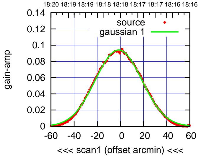
S04-175-AZ OFF= -0.9'
