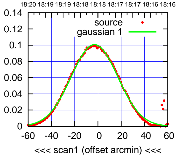
C02-175-AZ OFF= -2.6'
