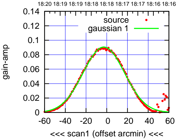
C02-130-AZ OFF= -2.5'
