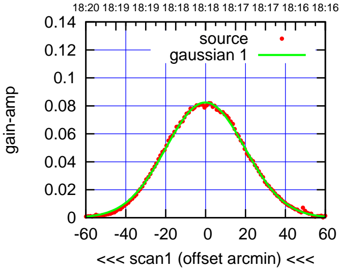
W01-130-AZ OFF= -4.6'
