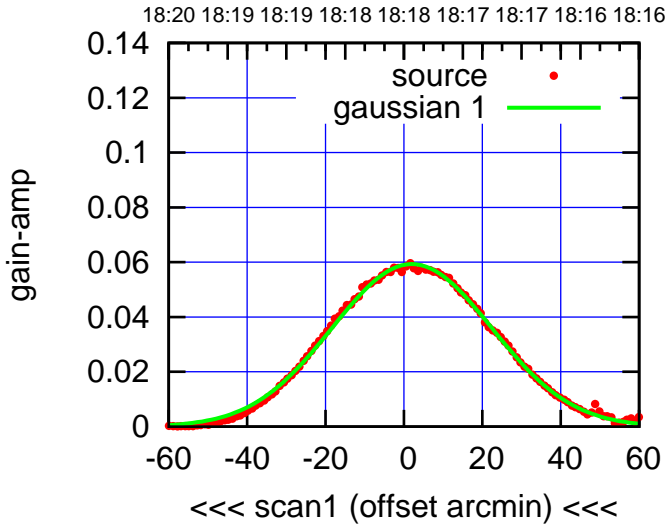
C11-130-AZ OFF= 2.5'
