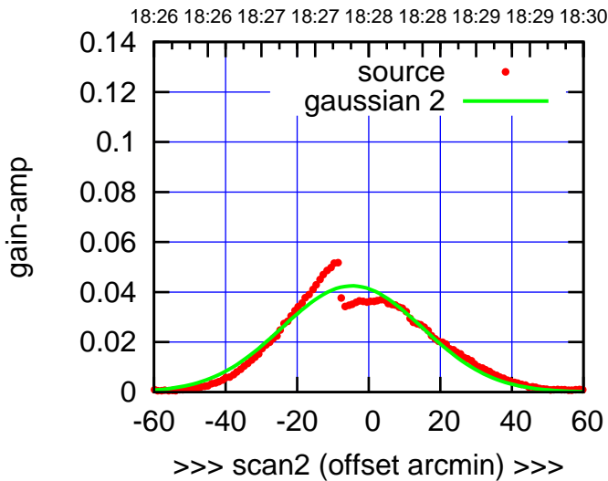
BACKLASH ERROR= 4.8'
