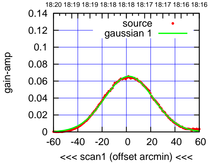
C11-175-AZ OFF= 2.6'
