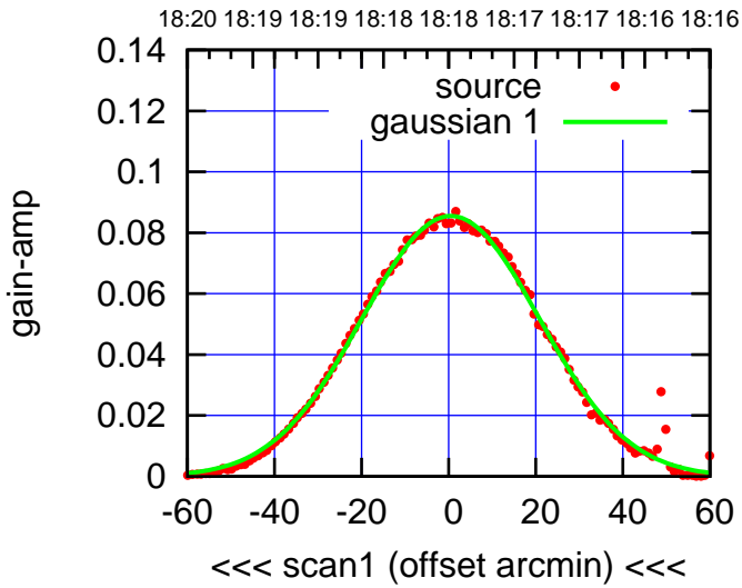
W02-130-AZ OFF= 0.4'
