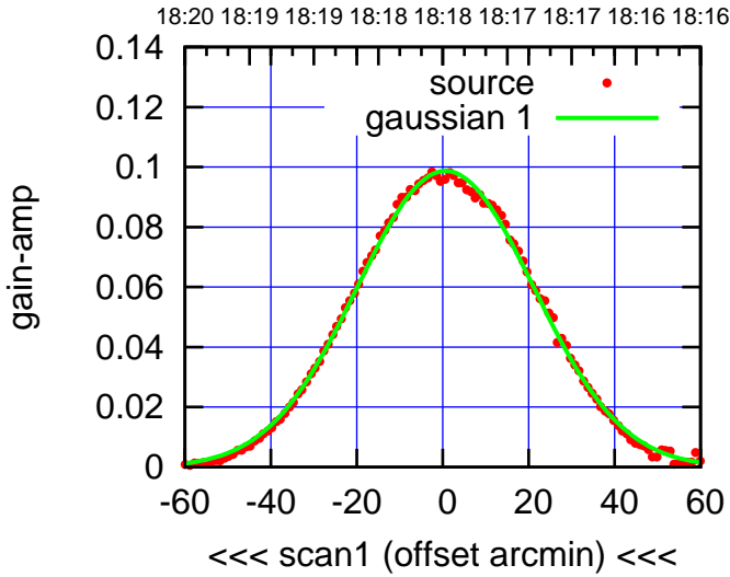
C00-130-AZ OFF= 1.9'
