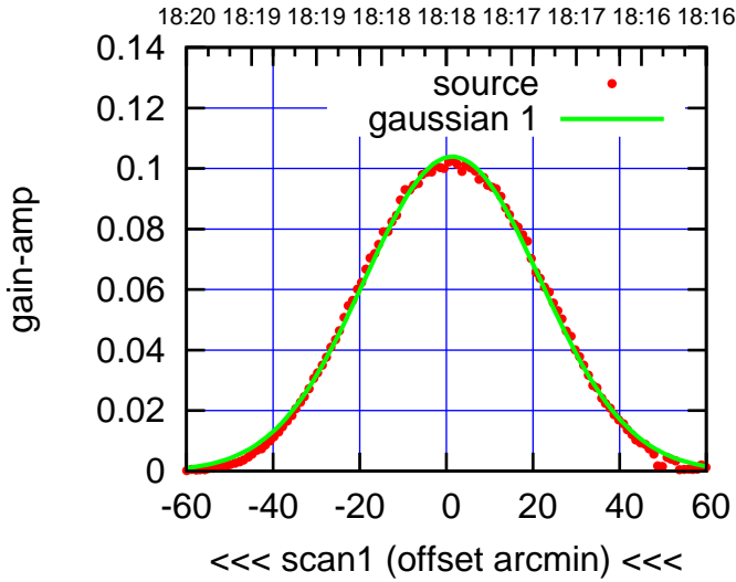
C13-130-AZ OFF= 2.5'
