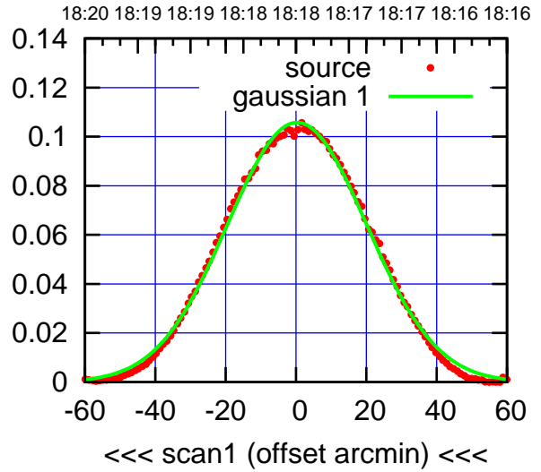
W06-175-AZ OFF= 0.9'
