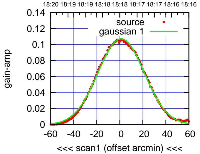
C00-175-AZ OFF= 2.3'
