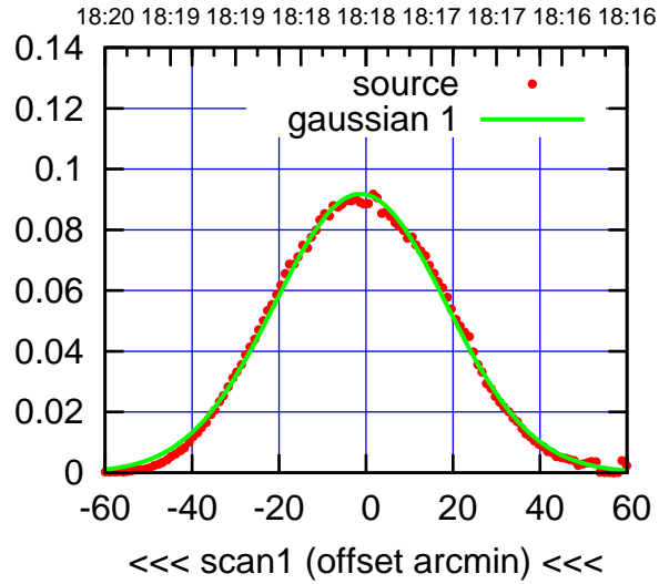
E05-175-AZ OFF= -0.4'
