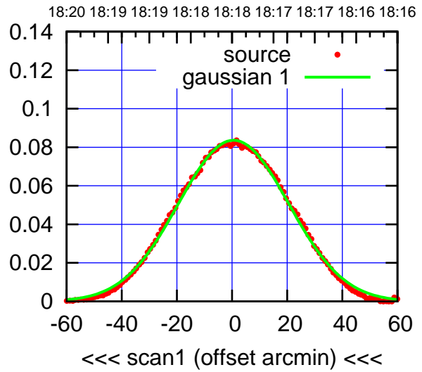
W05-175-AZ OFF= -0.7'
