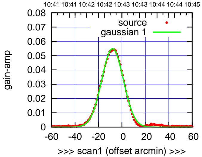
W05-175-EL OFF= -2.3' ( 21.5')
