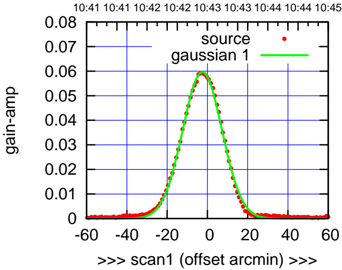
E06-130-EL OFF= -2.4' ( 22.7')
