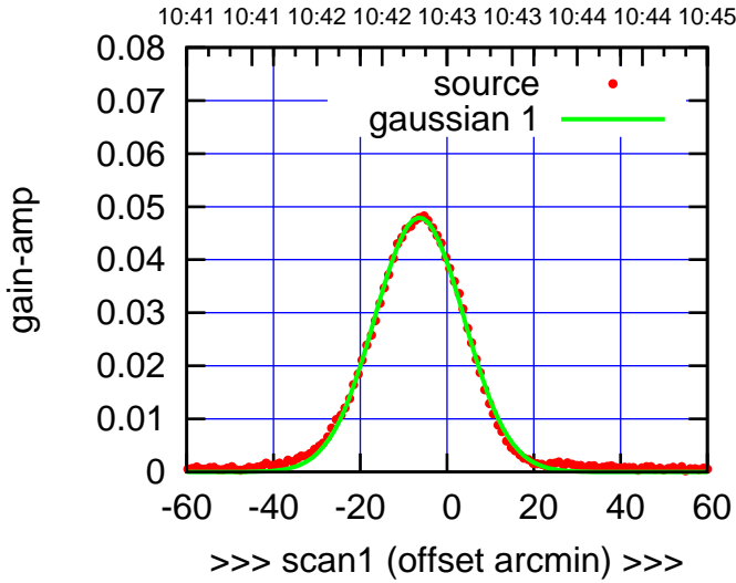
C11-130-EL OFF= -5.6' ( 24.0')
