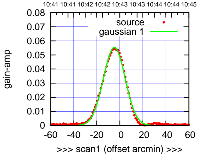
C10-175-EL OFF= -4.5' ( 22.0')
