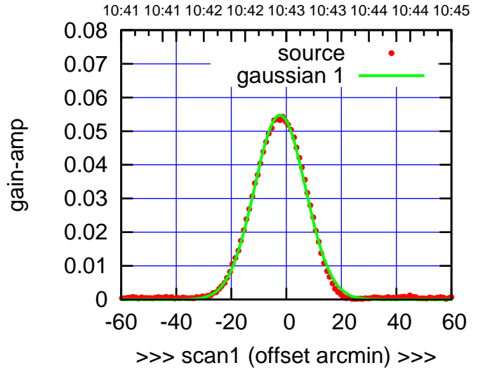
E06-175-EL OFF= -2.1' ( 21.8')
