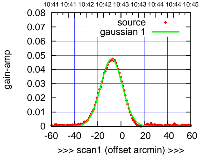
C09-175-EL OFF= -7.5' ( 21.7')
