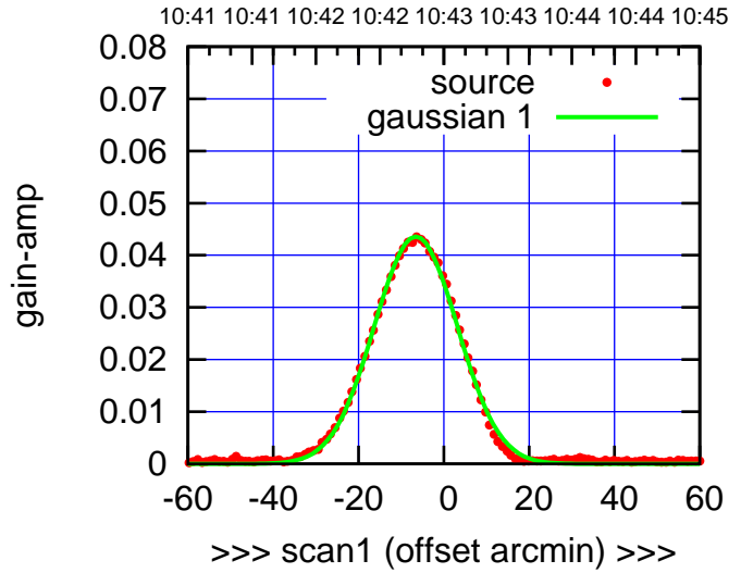
C11-175-EL OFF= -5.8' ( 22.6')
