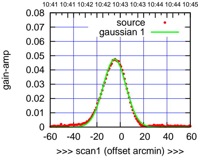
C10-130-EL OFF= -4.5' ( 22.8')
