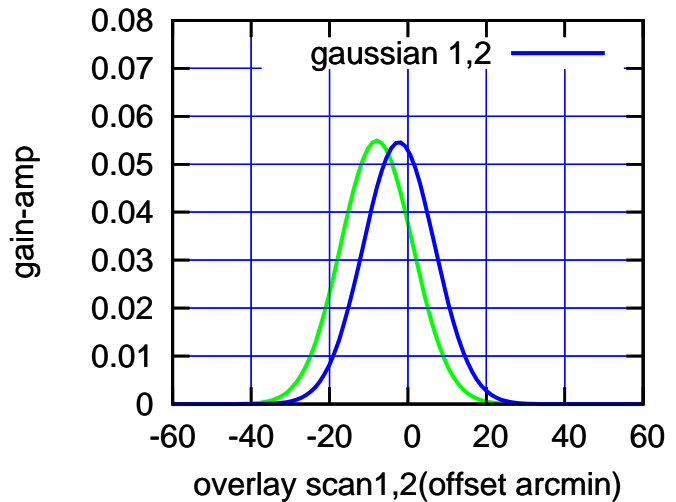
BACKLASH ERROR= 5.7'
