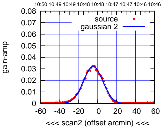
BACKLASH ERROR= 4.1'
