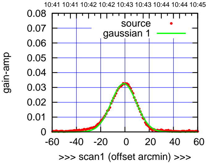
S06-130-EL OFF= 2.2' ( 24.4')
