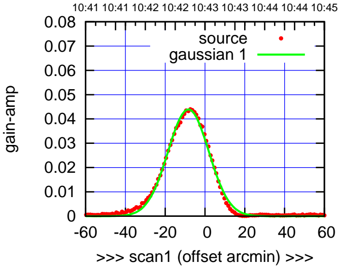
W06-130-EL OFF= -8.4' ( 23.9')
