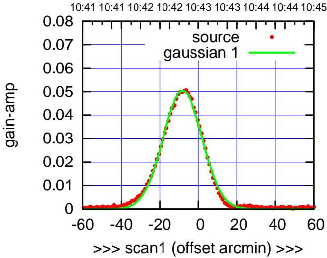
C09-130-EL OFF= -7.5' ( 23.4')
