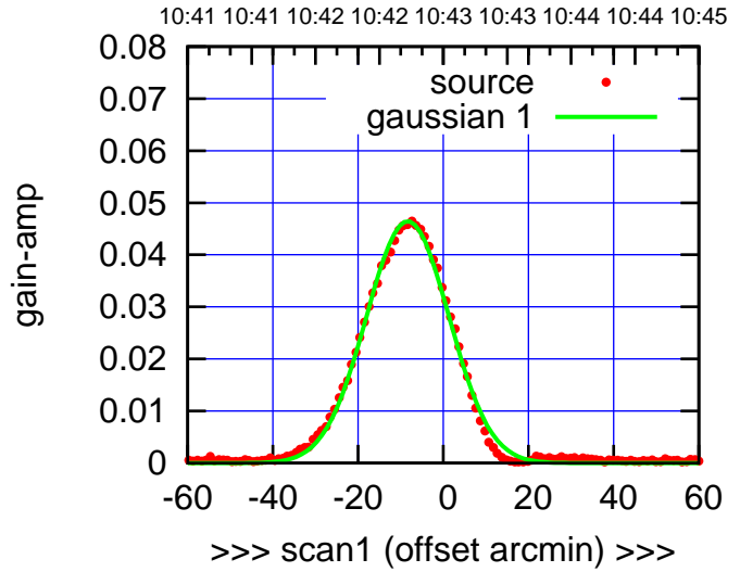
W06-175-EL OFF= -8.5' ( 22.6')
