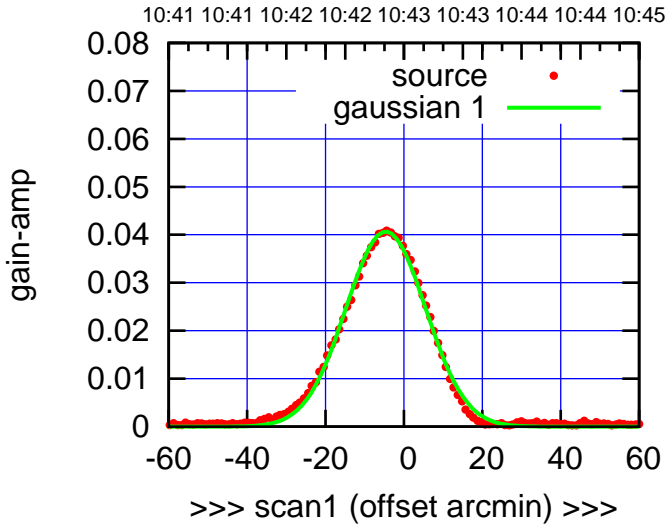
E03-130-EL OFF= -3.8' ( 24.1')
