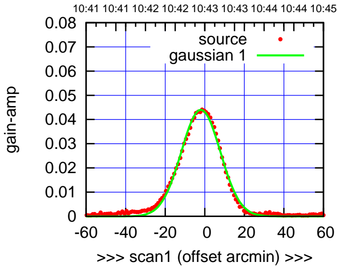
C06-130-EL OFF= -2.0' ( 23.1')
