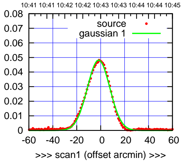
C06-175-EL OFF= -1.8' ( 21.8')
