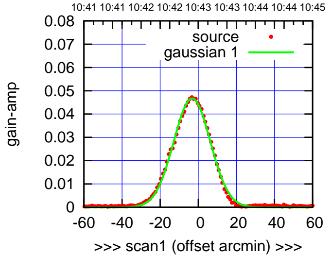
W02-175-EL OFF= -2.2' ( 22.2')
