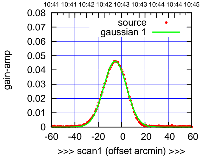
W04-175-EL OFF= -5.3' ( 22.8')
