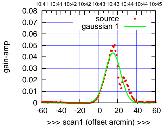
C08-175-EL OFF= 15.4' ( 18.3')
