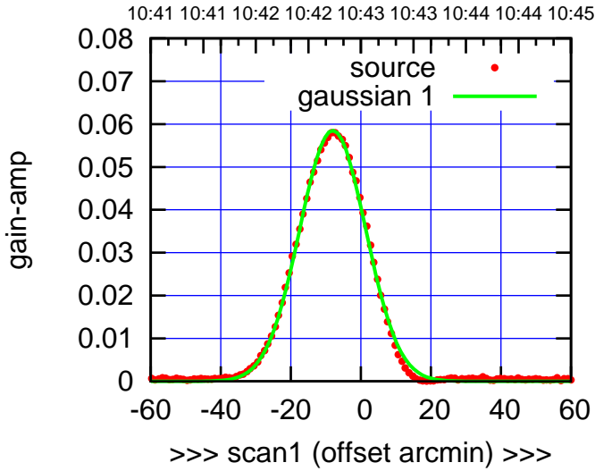
W05-130-EL OFF= -2.3' ( 22.1')
