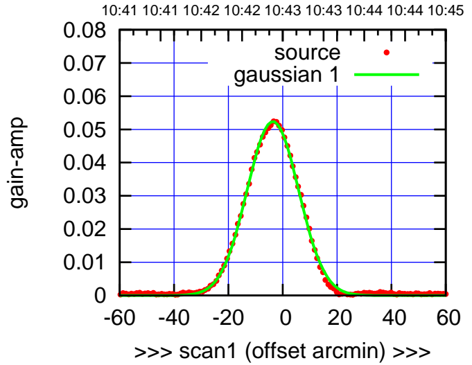
S01-175-EL OFF= -2.9' ( 22.3')
