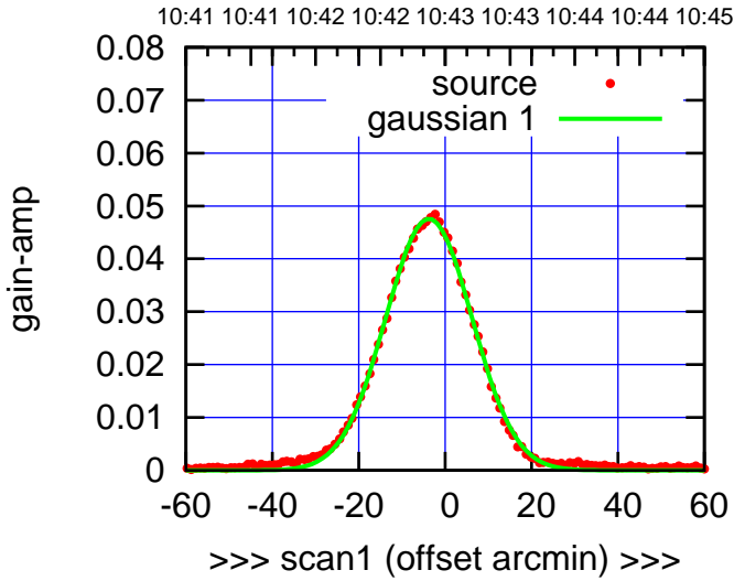
S01-130-EL OFF= -3.1' ( 23.4')
