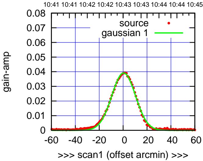
C12-130-EL OFF= 1.0' ( 22.9')
