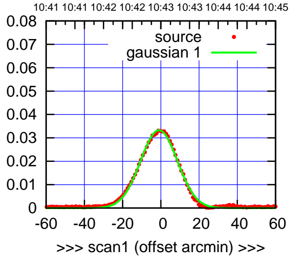
S06-175-EL OFF= 1.9' ( 22.5')
