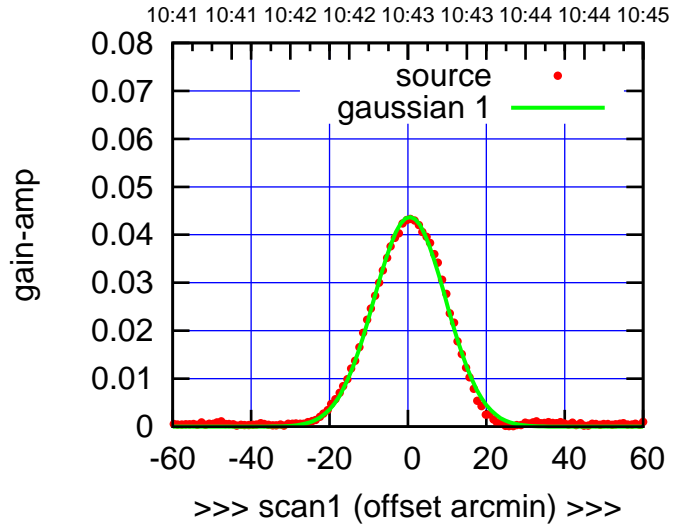
C12-175-EL OFF= 1.0' ( 21.1')
