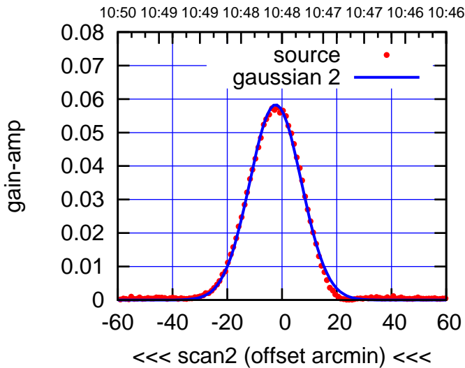
BACKLASH ERROR= 5.7'
