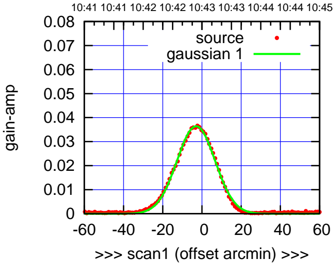
W02-130-EL OFF= -2.1' ( 22.7')
