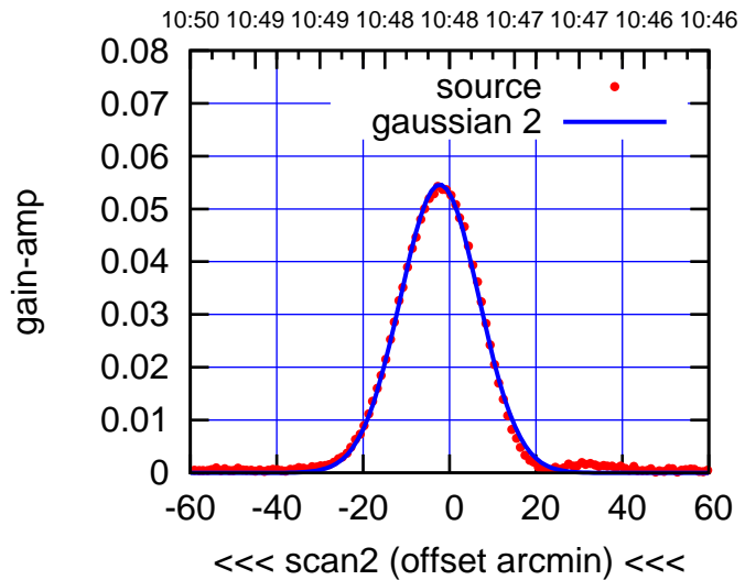
BACKLASH ERROR= 5.7'
