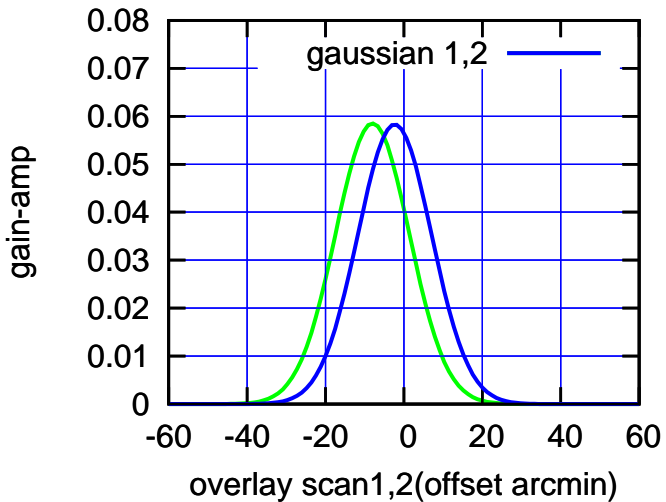
BACKLASH ERROR= 5.7'
