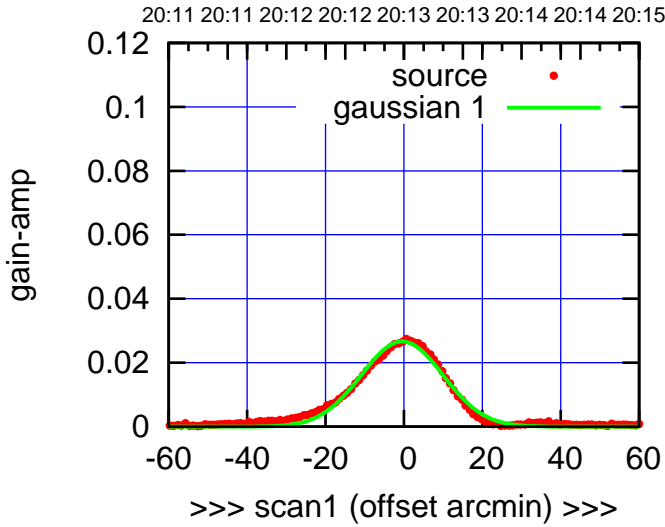
C13-130-EL OFF= -0.4' ( 24.4')
