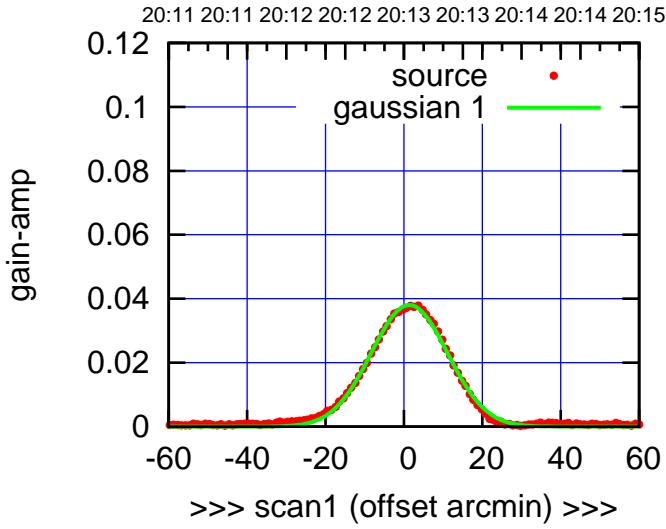
C04-130-EL OFF= 1.9' ( 23.0')
