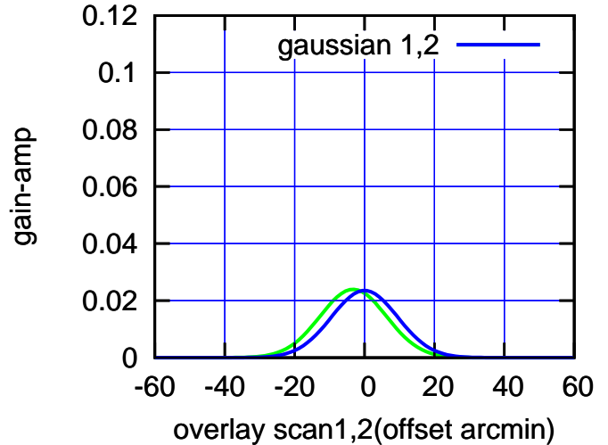
BACKLASH ERROR= 3.2'
