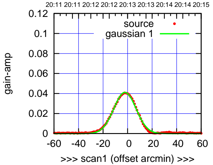
W05-175-EL OFF= 0.8' ( 21.0')
