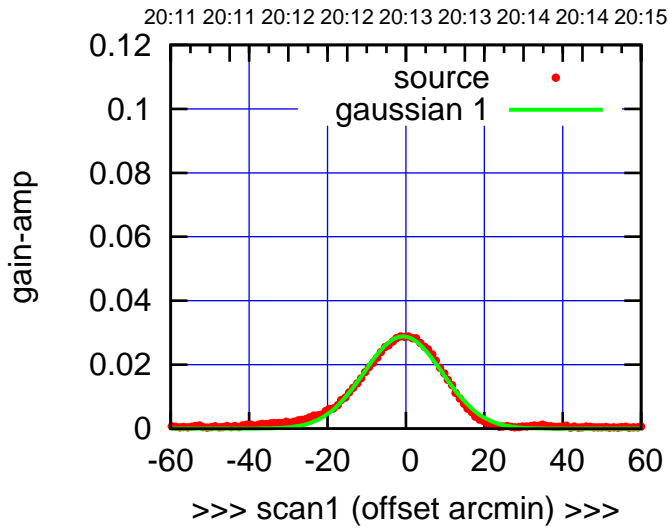
E02-130-EL OFF= -0.2' ( 23.3')
