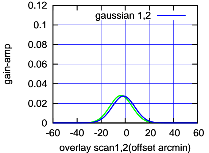
BACKLASH ERROR= 2.0'
