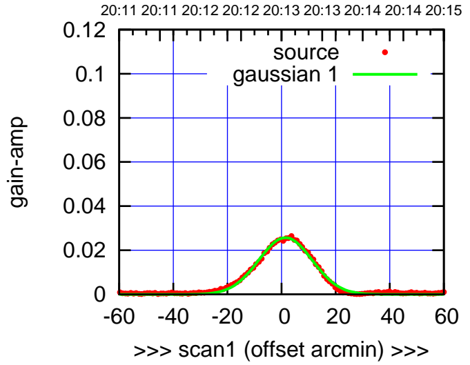
E03-175-EL OFF= 1.8' (23.3')
