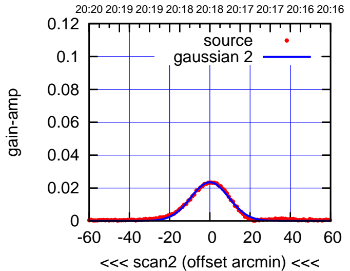
BACKLASH ERROR= 3.2'
