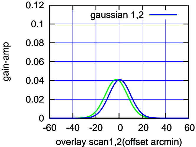
BACKLASH ERROR= 3.1'
