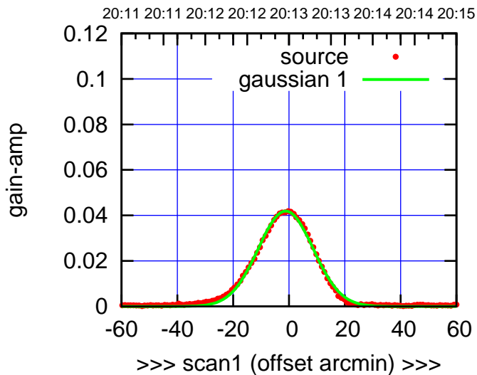
W03-130-EL OFF= -0.1' ( 23.4')
