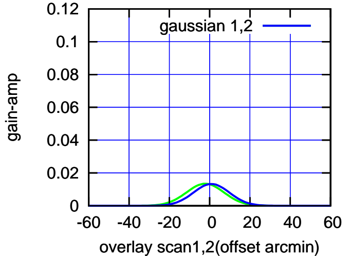
BACKLASH ERROR= 3.1'
