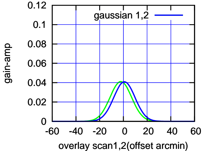
BACKLASH ERROR= 3.0'
