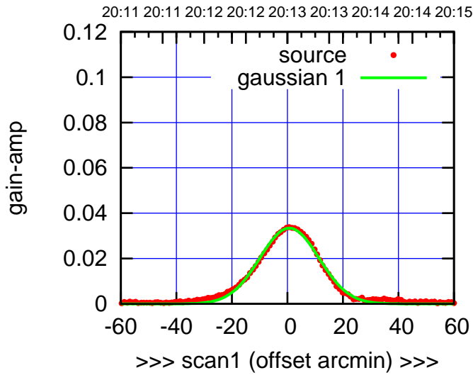
C11-130-EL OFF= 1.4' ( 25.1')
