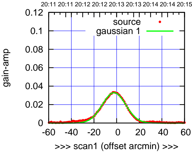
S03-130-EL OFF= -1.9' ( 24.0')
