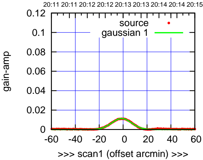
E04-130-EL OFF= 0.3' ( 19.4')
