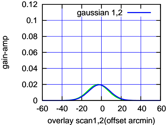
BACKLASH ERROR= 1.3'
