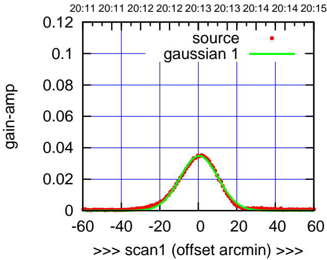
C08-130-EL OFF= 0.3' (22.9')
