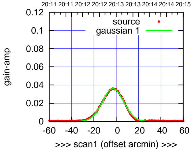
W02-175-EL OFF= -2.4' ( 22.1')
