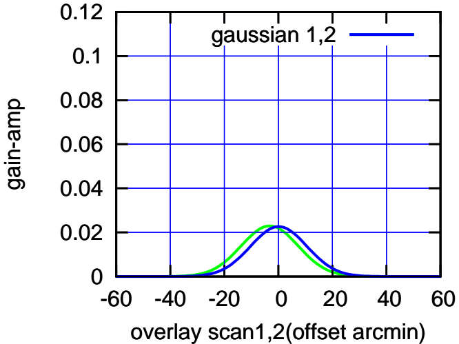
BACKLASH ERROR= 3.3'
