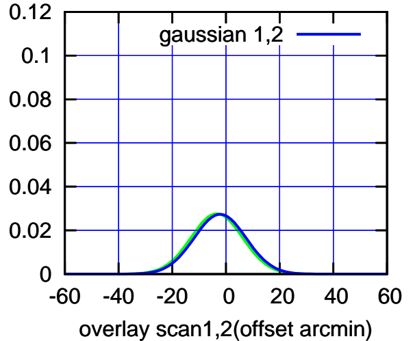
BACKLASH ERROR= 1.2'
