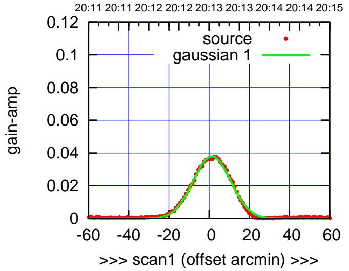
C04-175-EL OFF= 1.8' ( 22.0')
