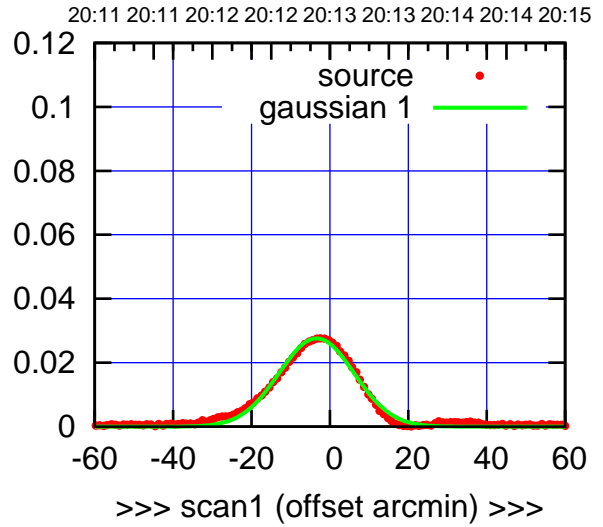
C02-175-EL OFF= -2.2' ( 22.6')
