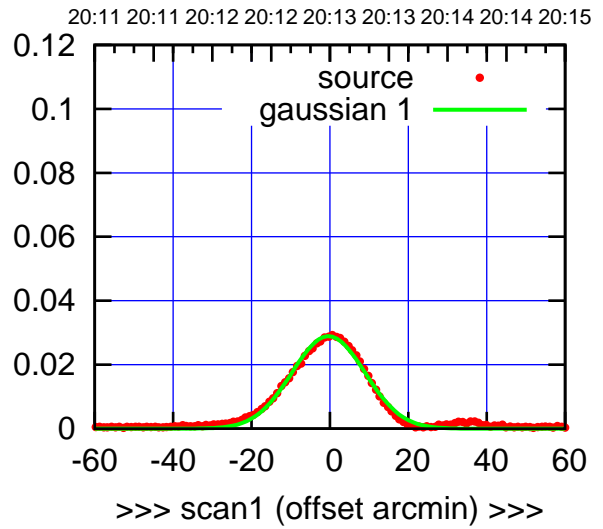
C00-175-EL OFF= 0.6' ( 22.1')
