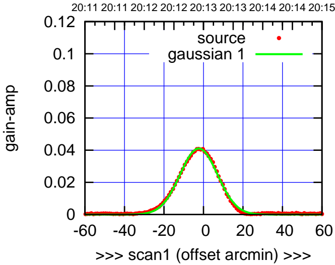
W05-130-EL OFF= 0.7' ( 21.9')
