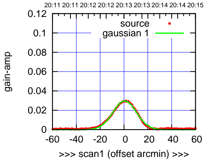
C11-175-EL OFF= 1.3' ( 23.3')
