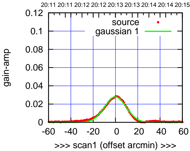
C00-130-EL OFF= 0.8' ( 22.8')
