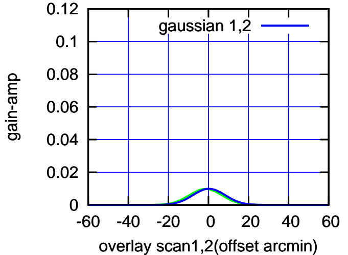
BACKLASH ERROR= 1.7'
