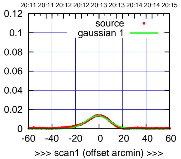
C03-175-EL OFF= -1.5' ( 23.1')
