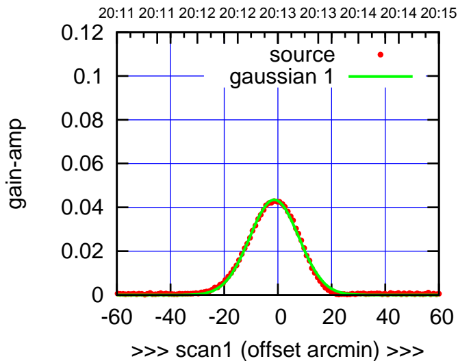
W03-175-EL OFF= -0.2' ( 21.7')
