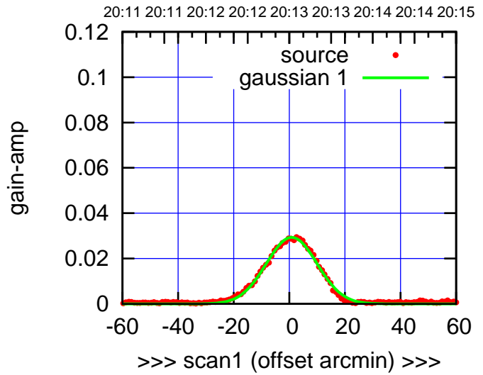
C08-175-EL OFF= 0.2' (21.1')
