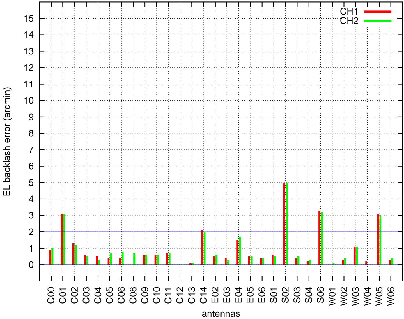
EL backlash test (08Mar2018 20:13:00)
