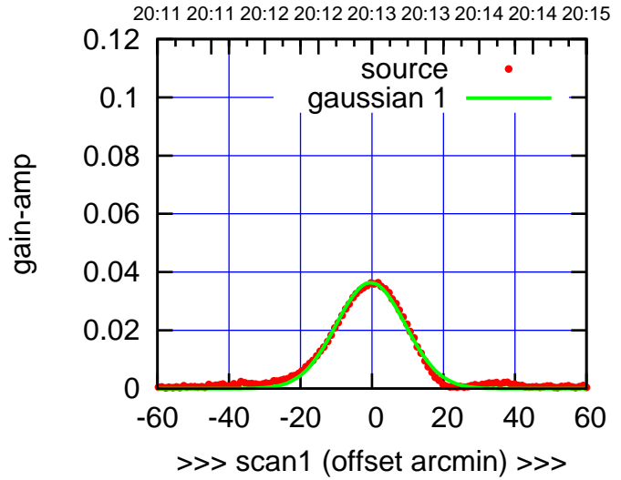
C10-175-EL OFF= -1.0' ( 22.2')
