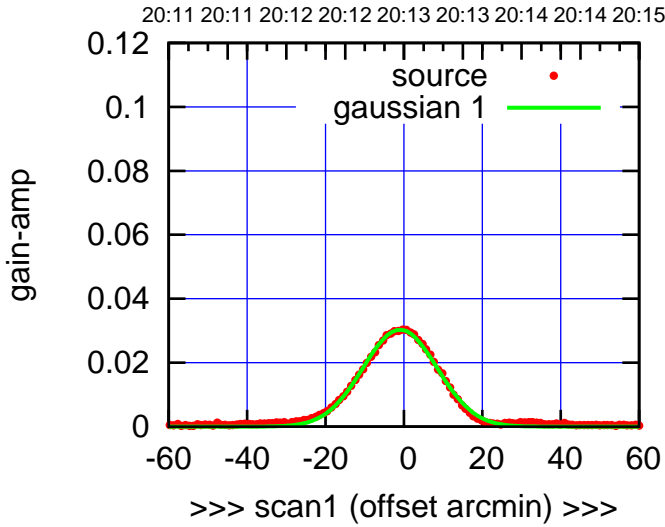
E06-130-EL OFF= -1.4' ( 22.3')
