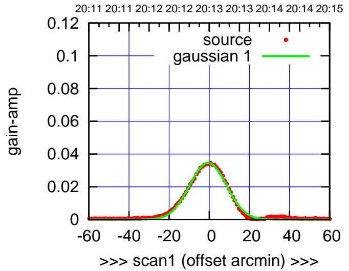
W01-175-EL OFF= -0.5' ( 21.3')
