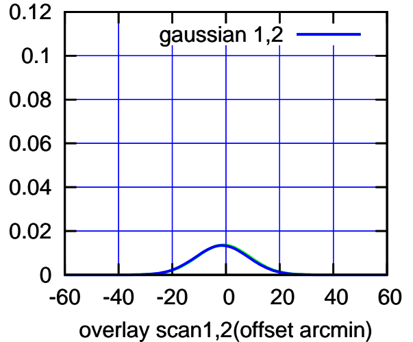
BACKLASH ERROR= 0.5'
