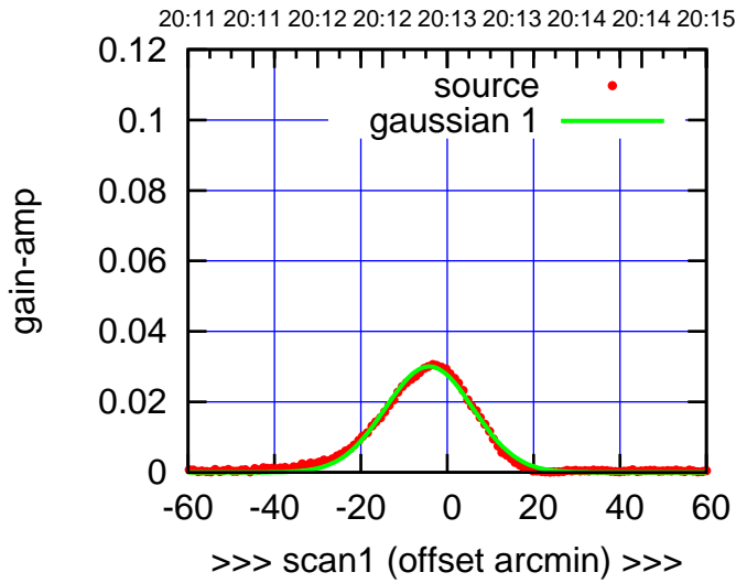
W06-130-EL OFF= -4.5' ( 23.8')
