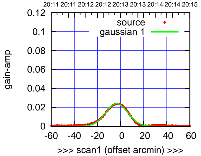
S06-175-EL OFF= -0.0' ( 22.2')
