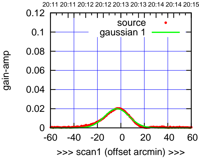
C02-130-EL OFF= -2.1' ( 25.0')
