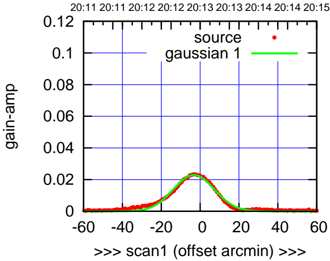
S06-130-EL OFF= 0.1' ( 24.5')
