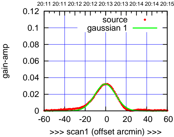
C10-130-EL OFF= -1.1' ( 23.2')
