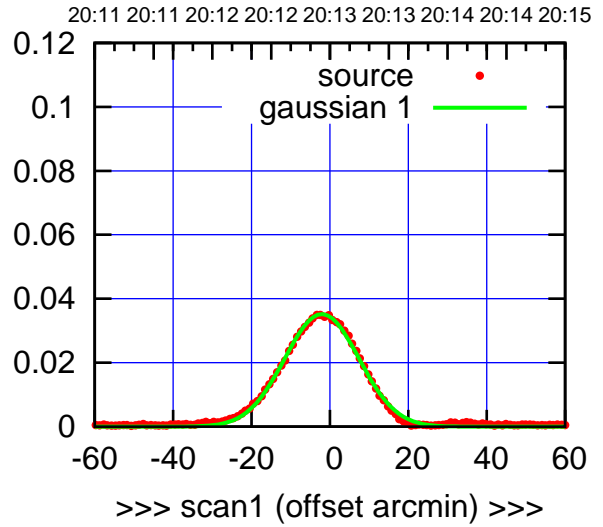
S03-175-EL OFF= -1.6' ( 22.1')
