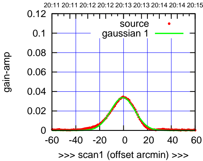
C09-130-EL OFF= -0.0' ( 23.7')
