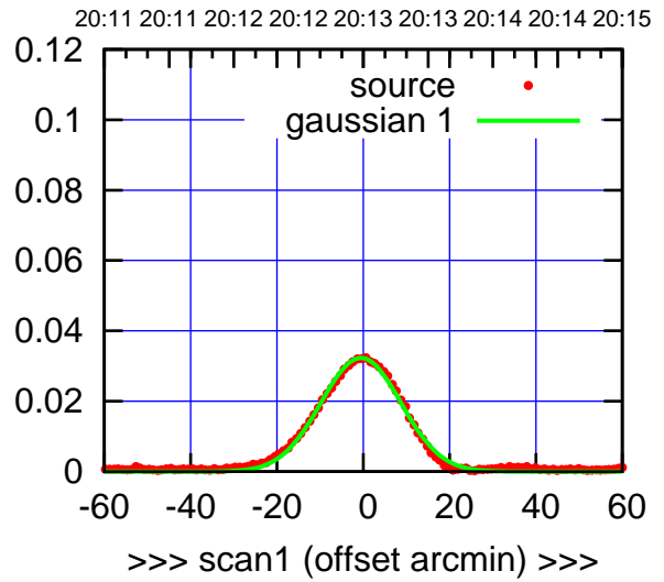
C09-175-EL OFF= 0.0' ( 21.6')
