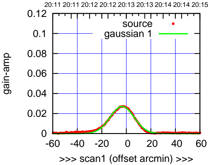
C14-130-EL OFF= -1.3' ( 23.0')
