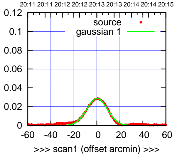
C05-175-EL OFF= -0.5' ( 21.4')
