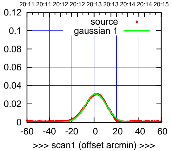
C06-175-EL OFF= 0.8' ( 22.1')
