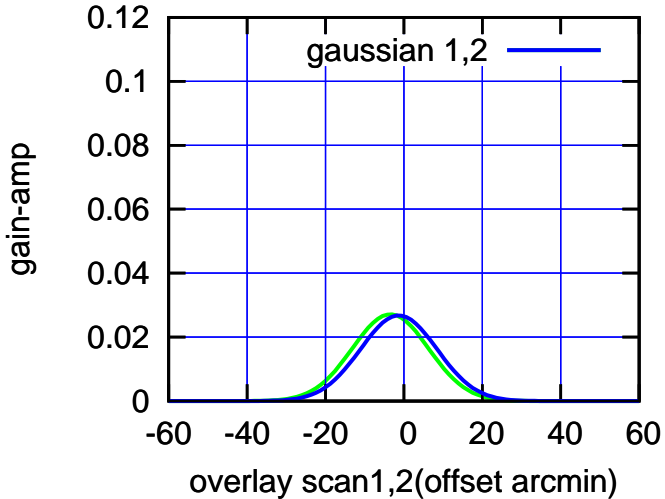
BACKLASH ERROR= 2.1'
