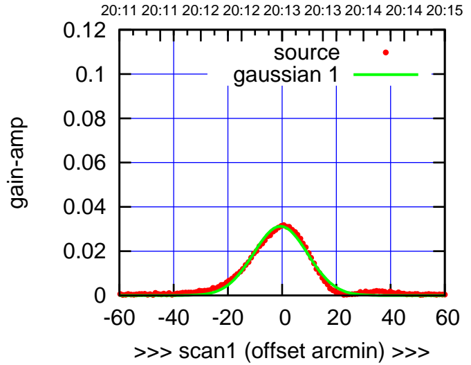
C13-175-EL OFF= -0.5' ( 23.5')
