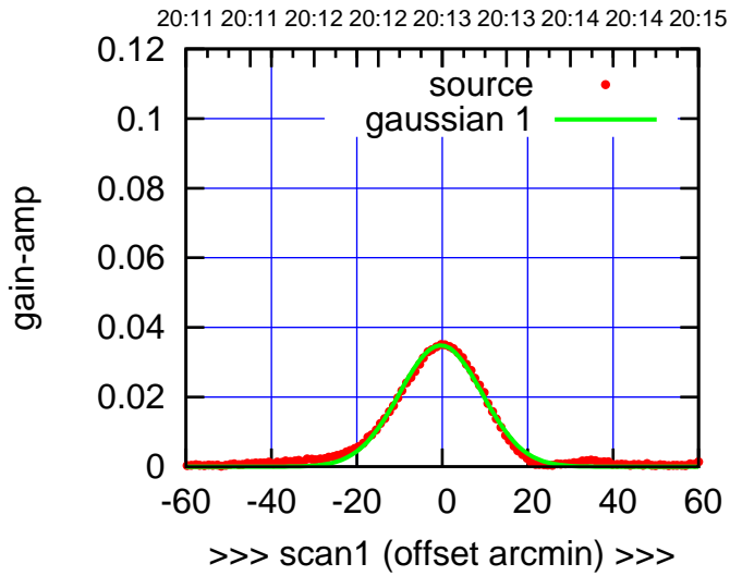
W01-130-EL OFF= -0.4' ( 22.6')
