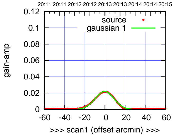
E02-175-EL OFF= 0.1' ( 21.7')
