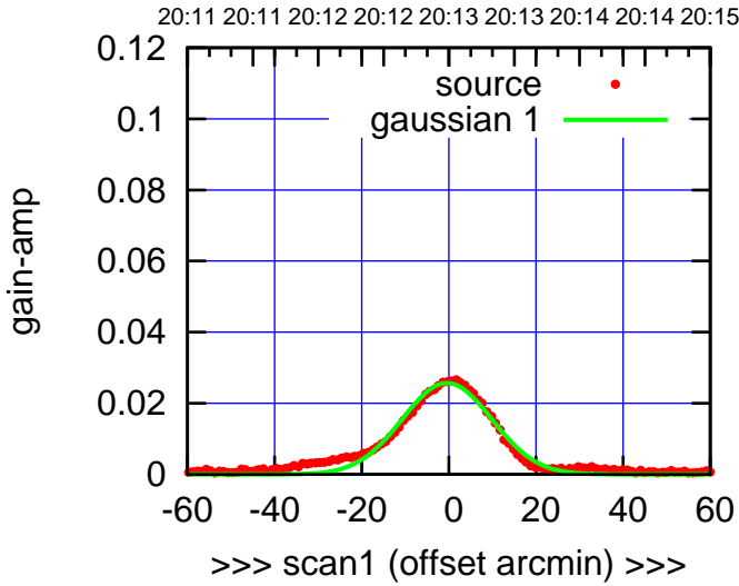
C05-130-EL OFF= -0.8' ( 24.4')
