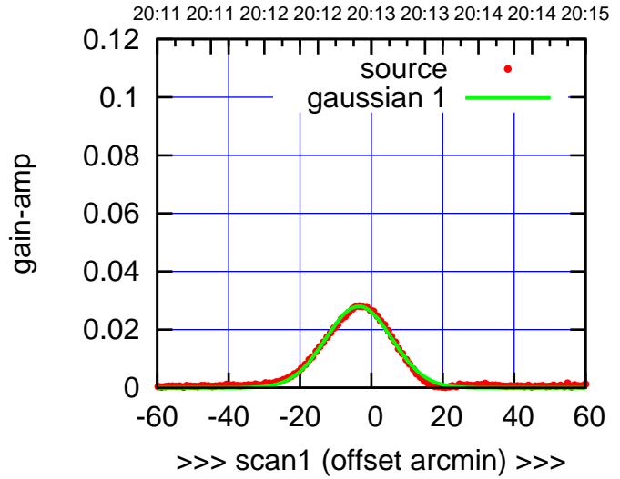
C14-175-EL OFF= -1.5' ( 21.9')
