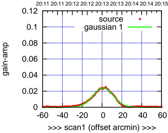
E03-130-EL OFF= 1.5' (24.2')
