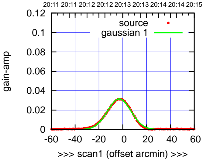
W02-130-EL OFF= -2.6' ( 23.0')
