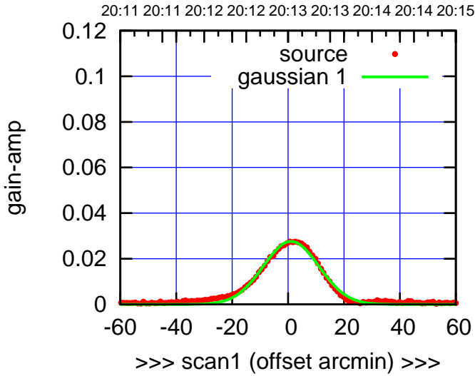
C06-130-EL OFF= 0.6' ( 23.4')
