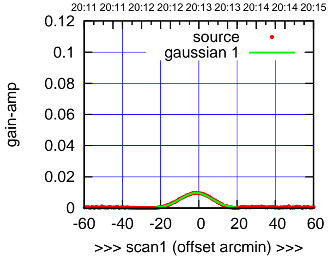
E04-175-EL OFF= 0.3' ( 19.0')
