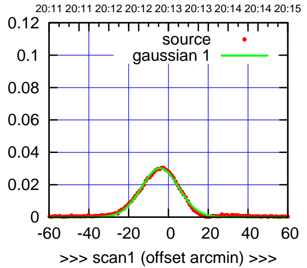
W06-175-EL OFF= -4.6' ( 22.2')
