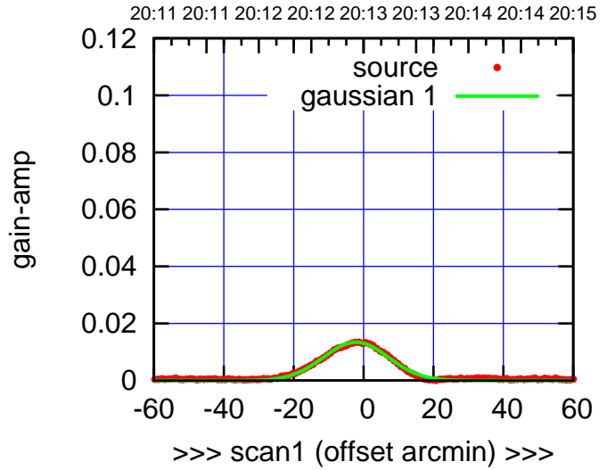
C01-175-EL OFF= 0.9' ( 21.0')
