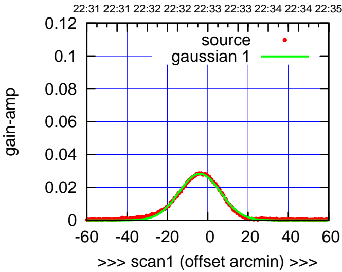
C14-130-EL OFF= -1.9' ( 24.6')
