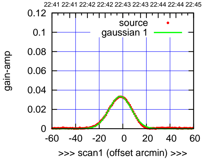
W02-175-EL OFF= -1.9' ( 22.4')
