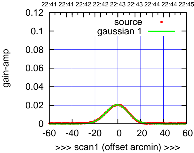
E04-130-EL OFF= 0.4' ( 22.5')
