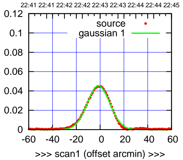
E05-175-EL OFF= -1.7' ( 21.9')
