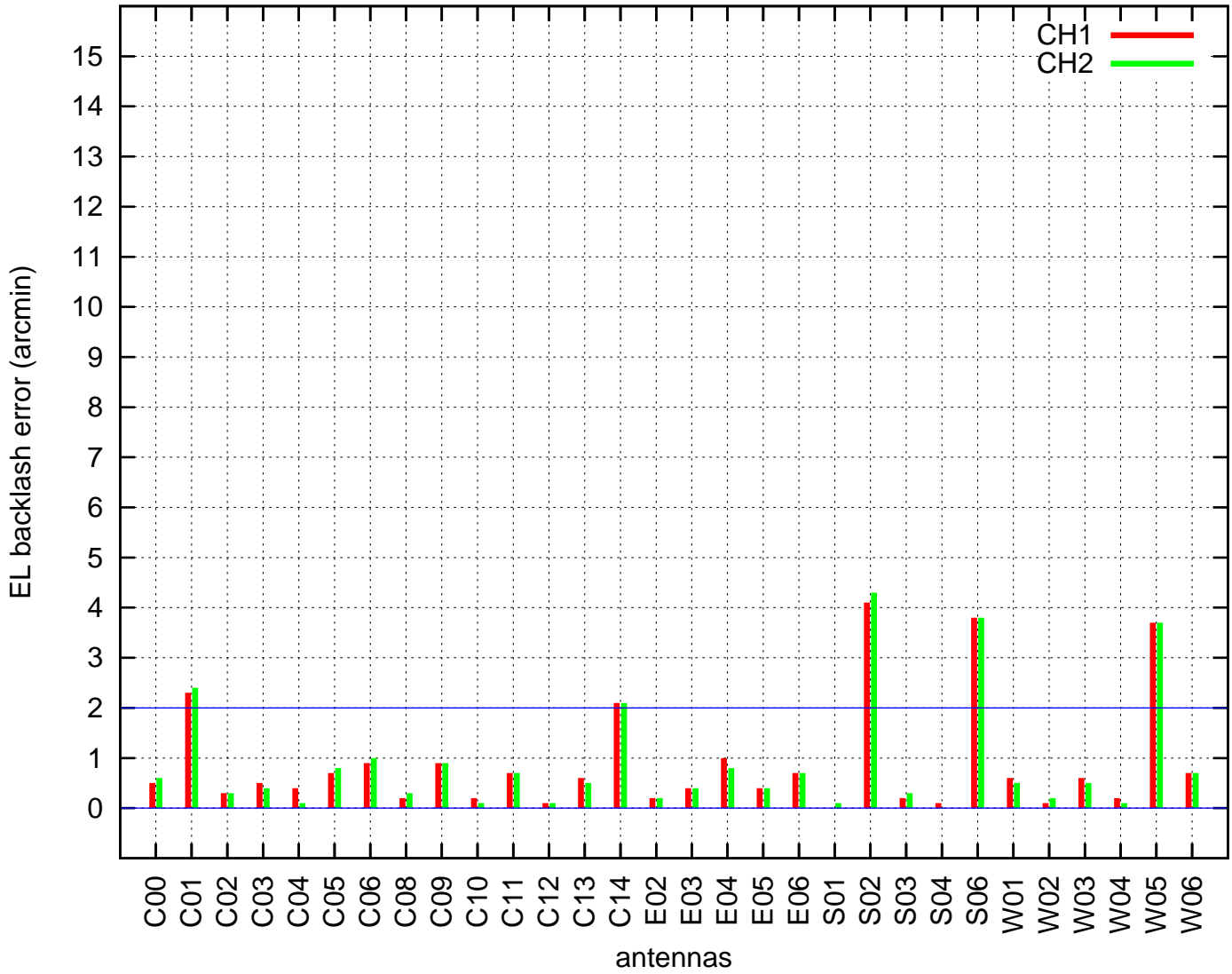
EL backlash test (17Jan2019 22:43:00)
