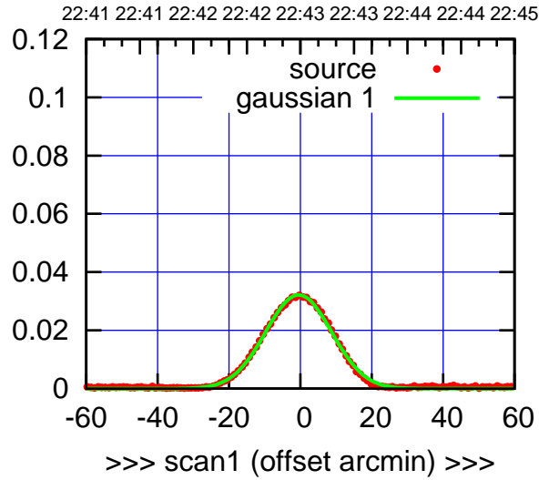
S04-175-EL OFF= -0.5' ( 21.5')
