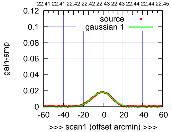
C11-175-EL OFF= -0.5' ( 23.0')
