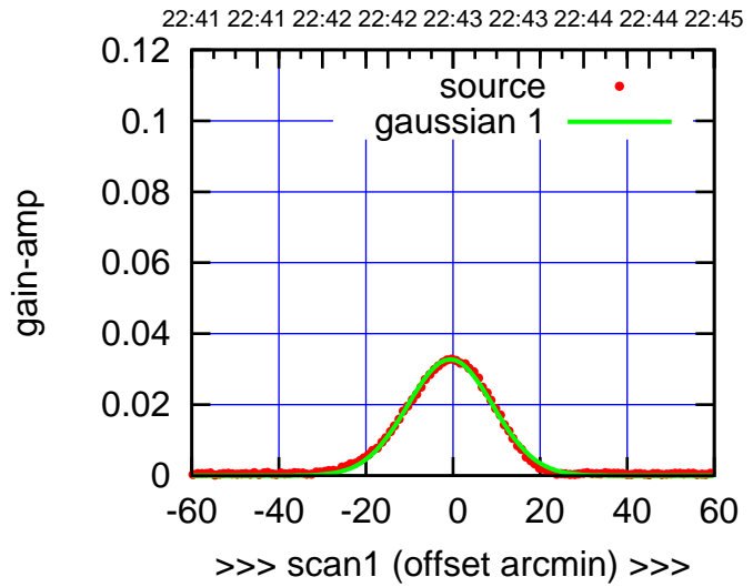
W04-175-EL OFF= -0.7' ( 22.9')
