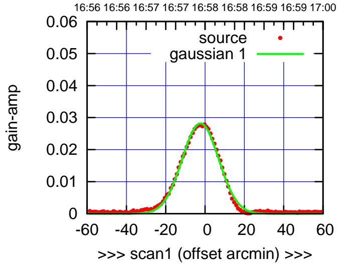
C14-175-EL OFF= -1.2'
