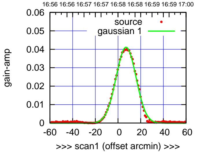
C08-175-EL OFF= 6.9'
