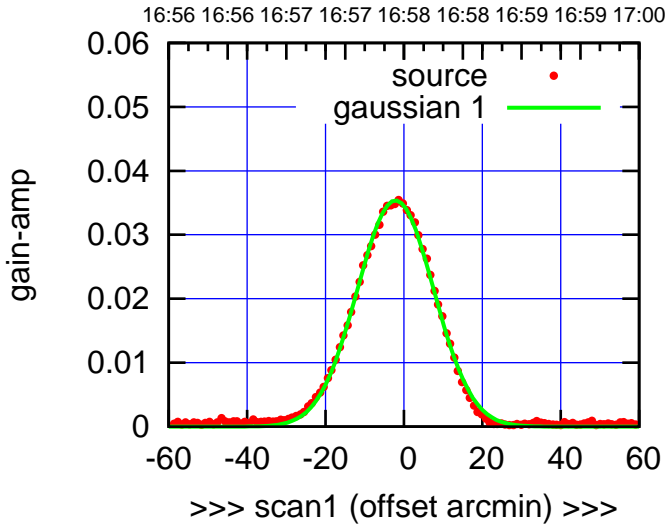
W03-130-EL OFF= -1.1'
