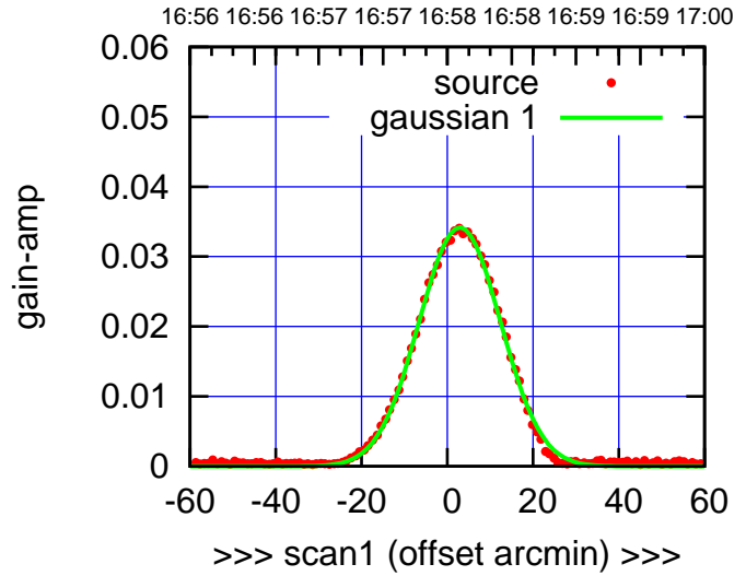
W02-175-EL OFF= 2.9'
