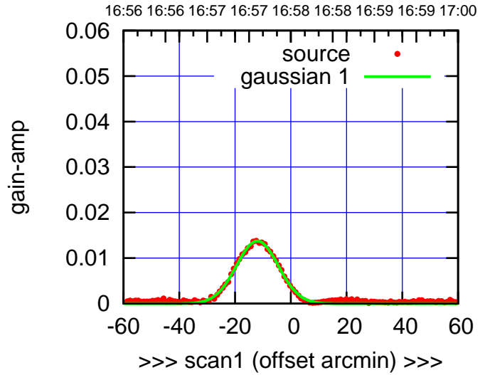
E06-175-EL OFF= -2.8'
