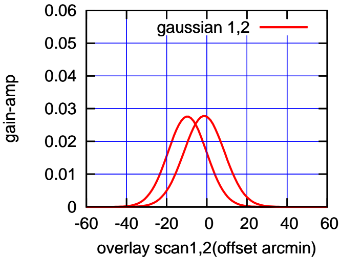
BACKLASH ERROR= 8.4'
