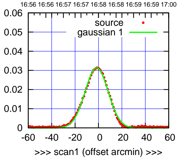
E03-175-EL OFF= -1.4'
