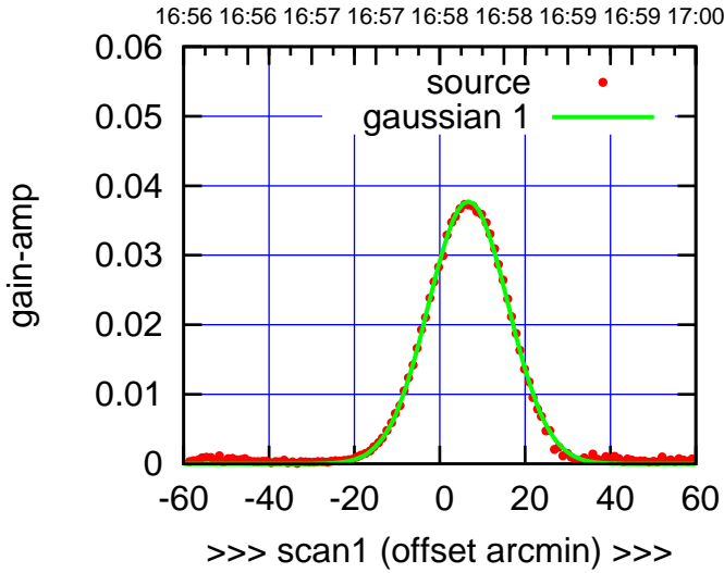
C08-130-EL OFF= 6.8'
