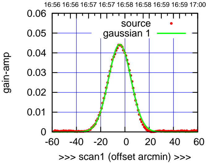
W05-130-EL OFF= -2.4'
