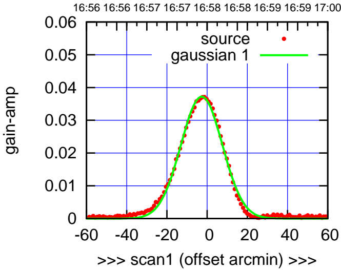
C13-130-EL OFF= -2.2'
