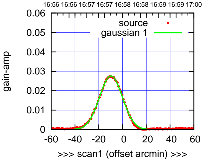
S04-130-EL OFF= -1.3'
