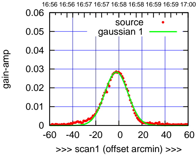
C14-130-EL OFF= -1.2'
