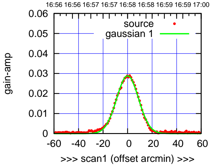
C03-175-EL OFF= -0.9'
