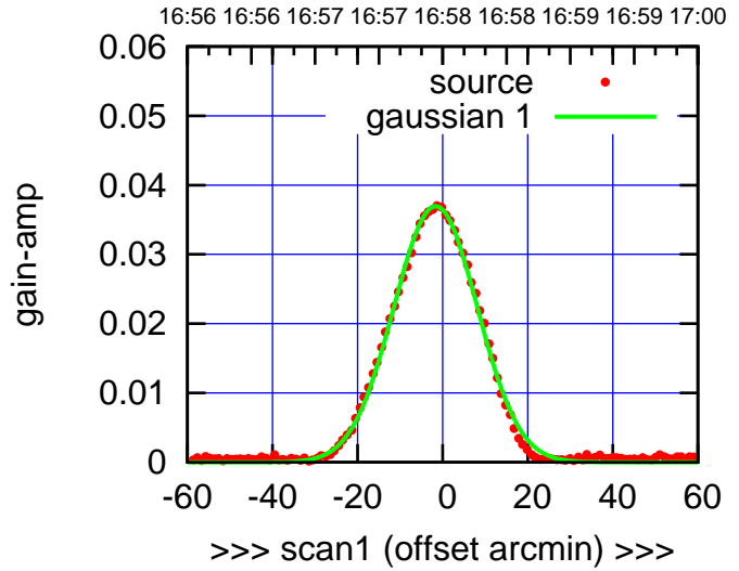
C00-175-EL OFF= 2.5'
