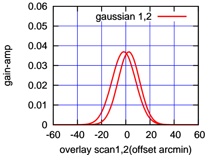
BACKLASH ERROR= 4.2'
