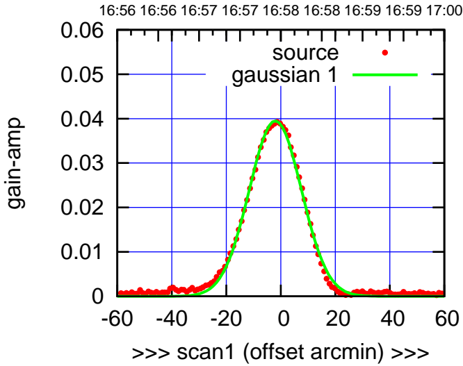
C10-130-EL OFF= -1.6'
