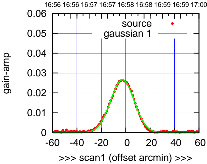
C01-130-EL OFF= -0.2'
