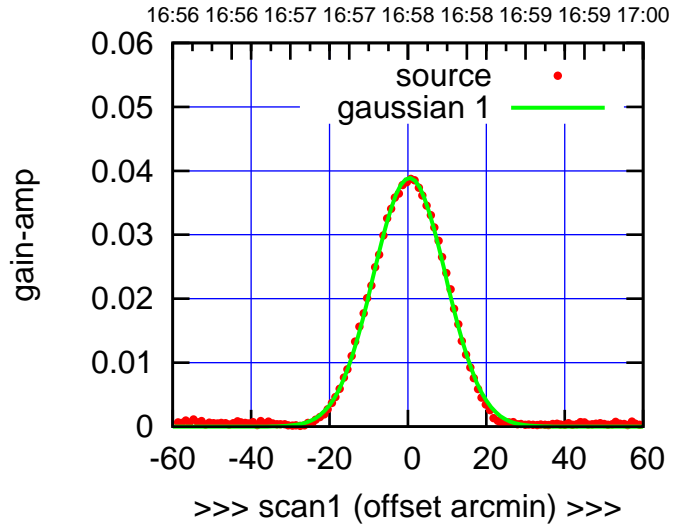
C04-175-EL OFF= 0.7'
