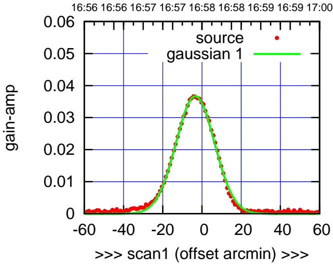
C06-130-EL OFF= -3.8'
