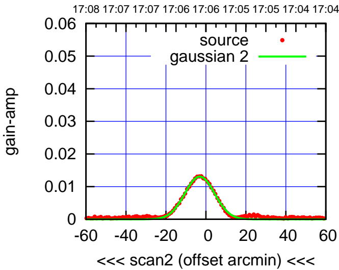
BACKLASH ERROR= 9.2'
