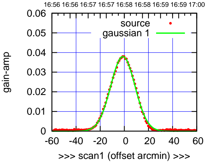
C00-130-EL OFF= 2.9'
