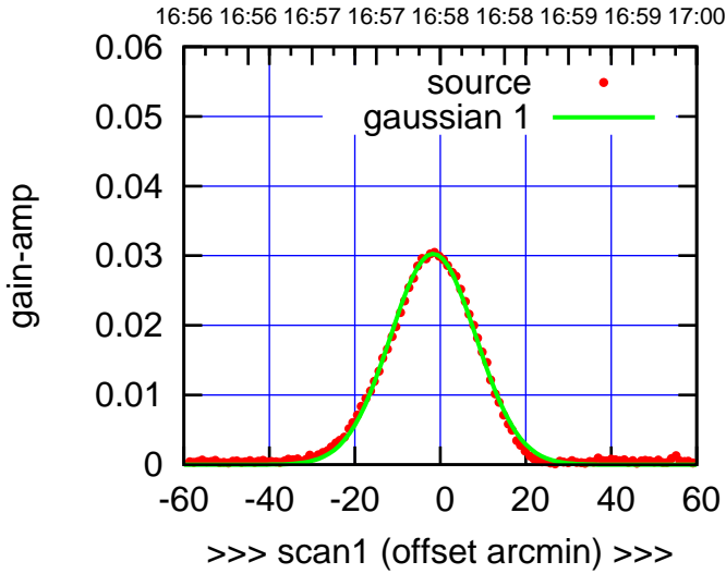
E03-130-EL OFF= -1.6'
