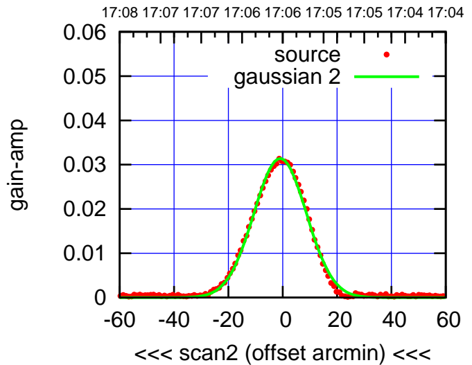
BACKLASH ERROR= 8.5'
