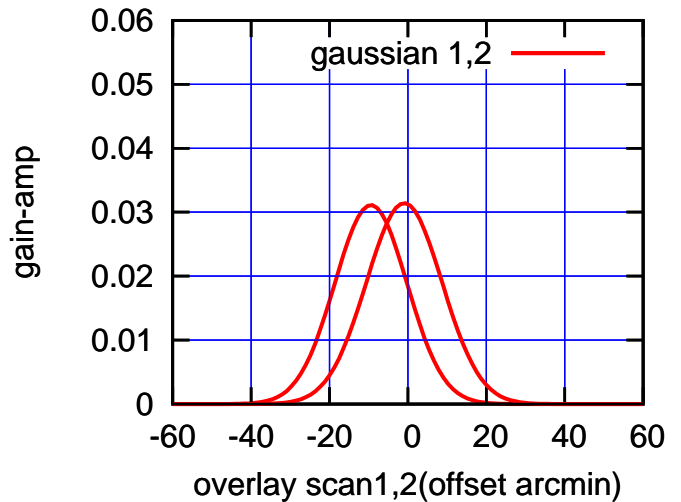
BACKLASH ERROR= 8.5'
