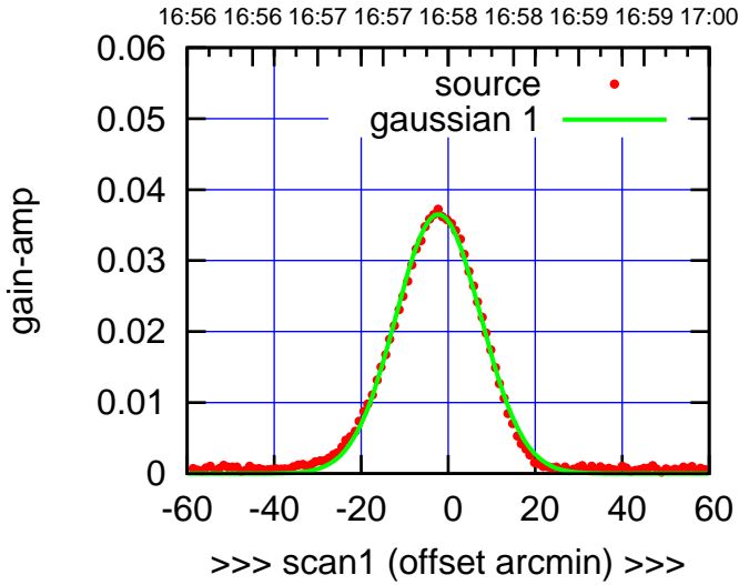
C09-130-EL OFF= -1.7'
