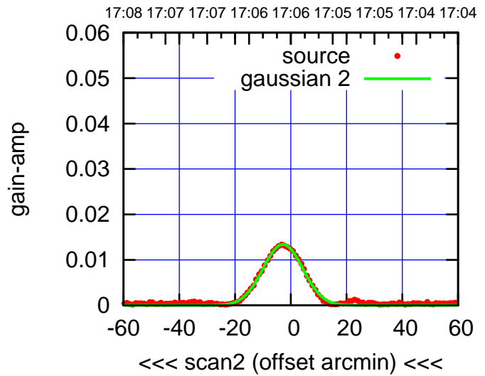
BACKLASH ERROR= 9.2'
