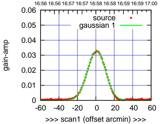
C11-175-EL OFF= 0.9'
