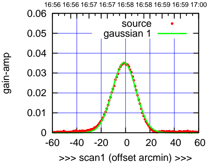
E02-130-EL OFF= -1.3'
