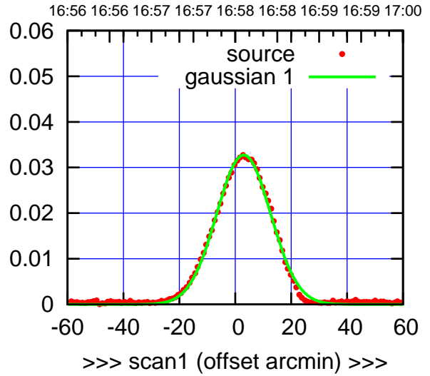
W06-175-EL OFF= 2.0'
