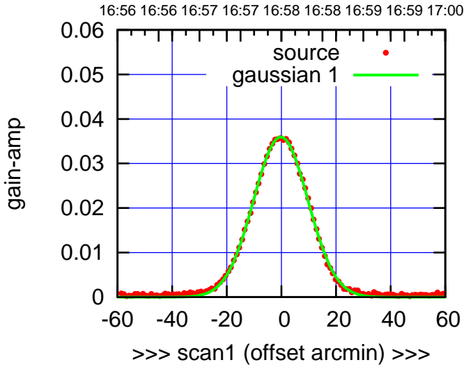
S01-130-EL OFF= -0.3'
