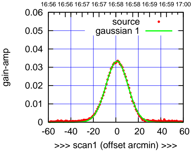
C02-130-EL OFF= 0.6'
