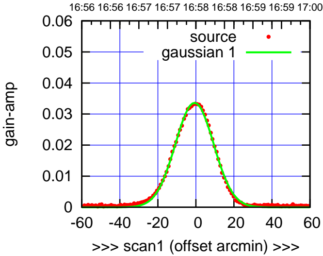
S03-130-EL OFF= -0.7'
