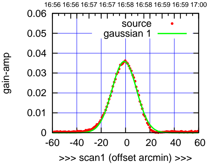
E05-130-EL OFF= -1.7'
