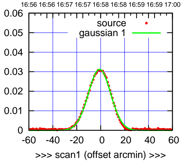
E02-175-EL OFF= -1.3'
