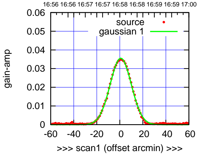
C02-175-EL OFF= 0.5'
