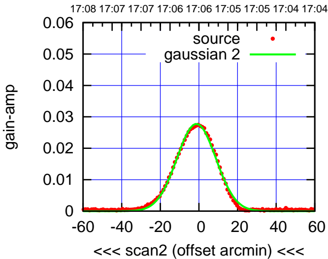
BACKLASH ERROR= 8.4'
