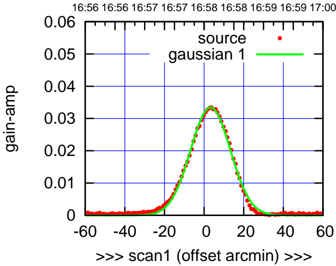
W06-130-EL OFF= 2.2'
