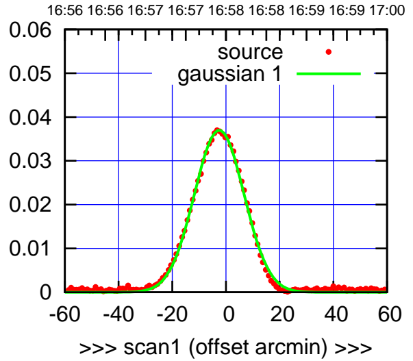
C09-175-EL OFF= -1.9'
