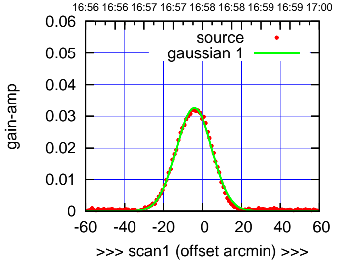
W05-175-EL OFF= -2.4'
