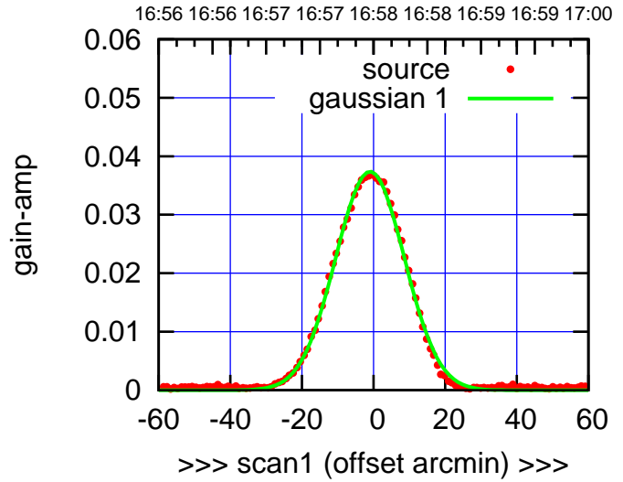
S03-175-EL OFF= -0.9'
