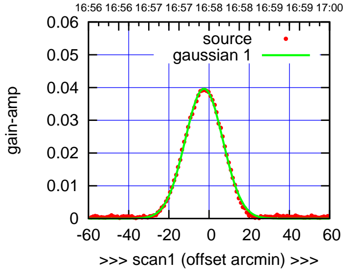
W03-175-EL OFF= -1.5'
