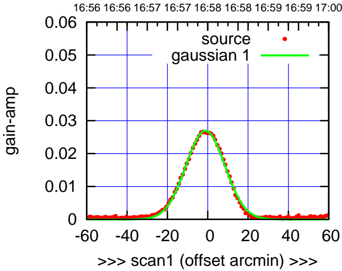
C12-130-EL OFF= -1.3'
