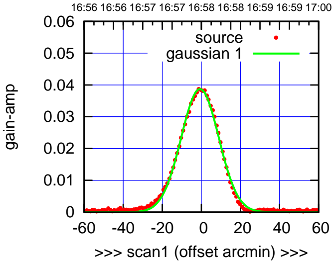
W01-130-EL OFF= -0.4'
