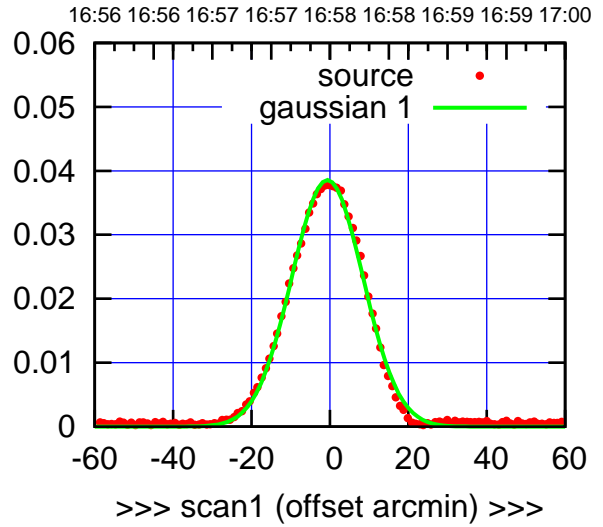
W01-175-EL OFF= -0.4'
