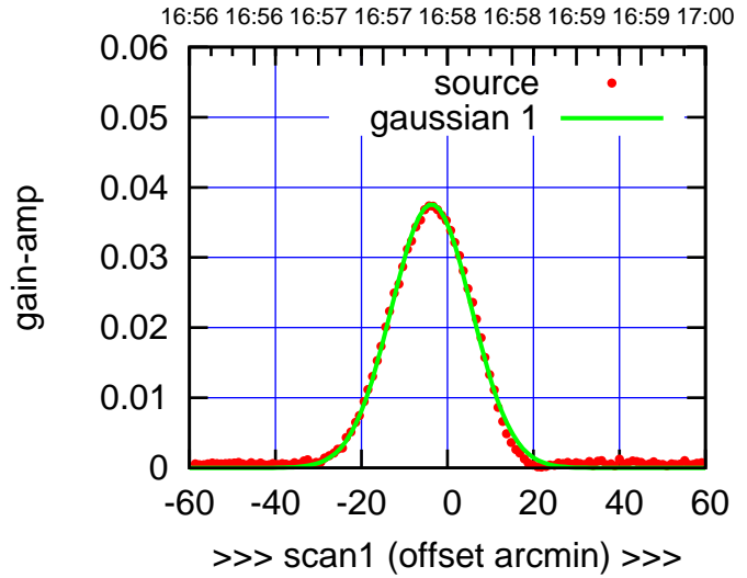
C06-175-EL OFF= -4.1'
