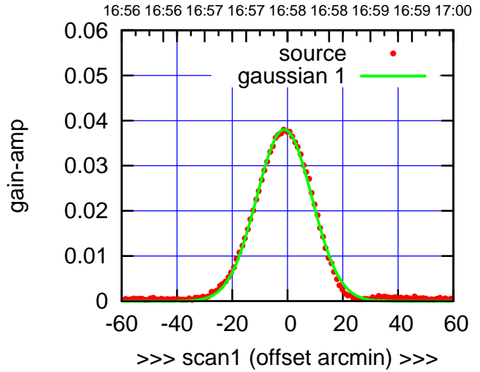
E05-175-EL OFF= -1.8'
