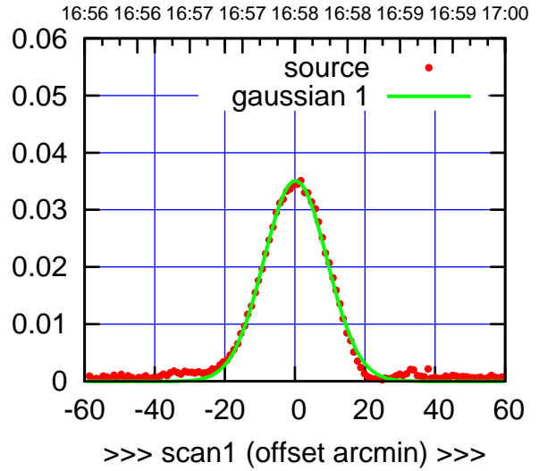
C05-175-EL OFF= -1.0'
