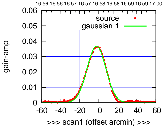
C13-175-EL OFF= -1.9'
