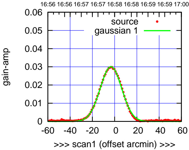
E04-130-EL OFF= -3.0'
