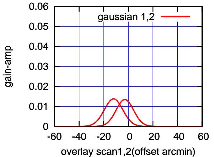
BACKLASH ERROR= 9.2'
