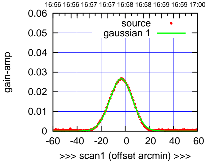
E04-175-EL OFF= -3.0'
