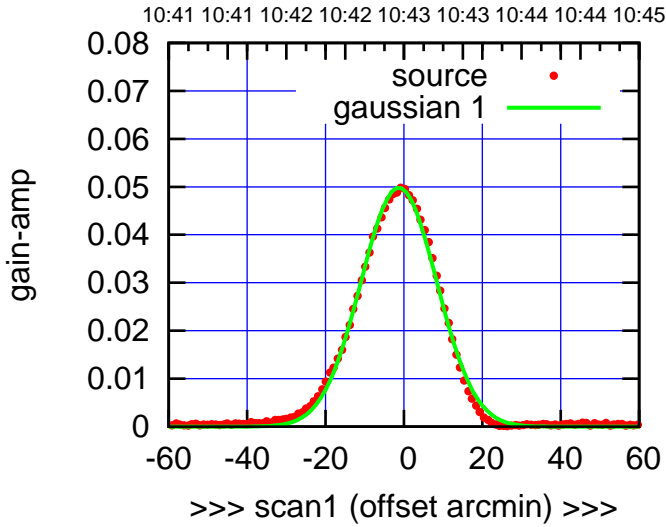
W04-130-EL OFF= -0.9' ( 22.8')
