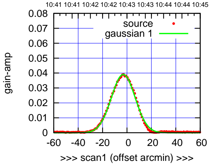
E04-175-EL OFF= -3.1' ( 22.3')
