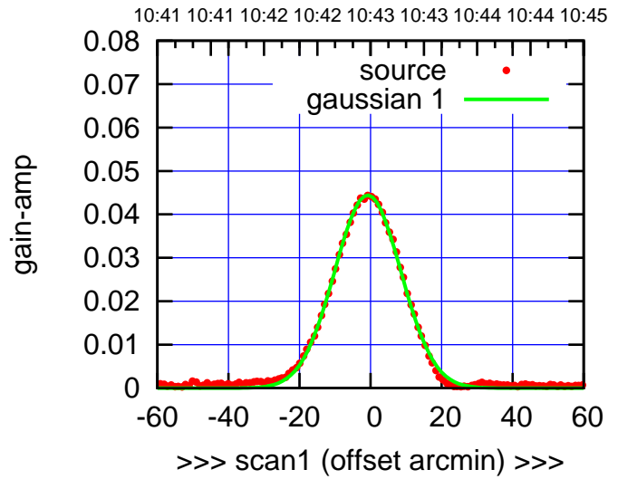
C06-175-EL OFF= -1.4' ( 21.9')
