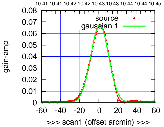
E05-175-EL OFF= 1.4' (22.5')
