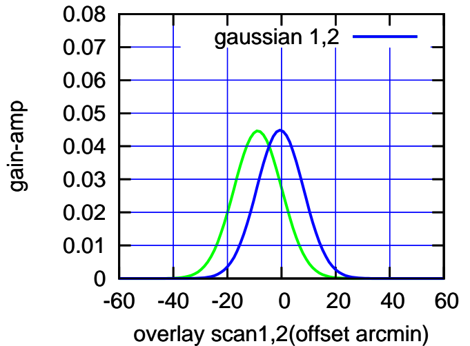
BACKLASH ERROR= 8.2'
