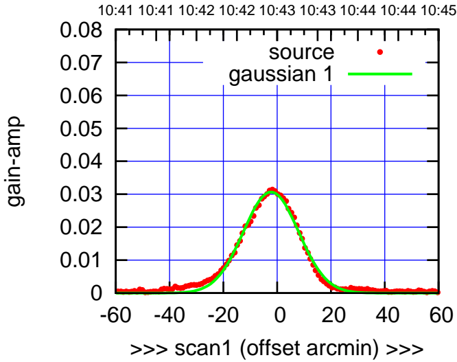
S06-130-EL OFF= -2.0' ( 24.3')
