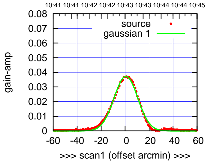
W06-175-EL OFF= 0.5' ( 22.7')
