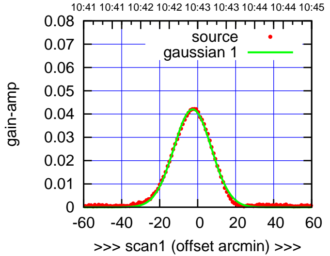
C11-175-EL OFF= -1.8' ( 23.1')
