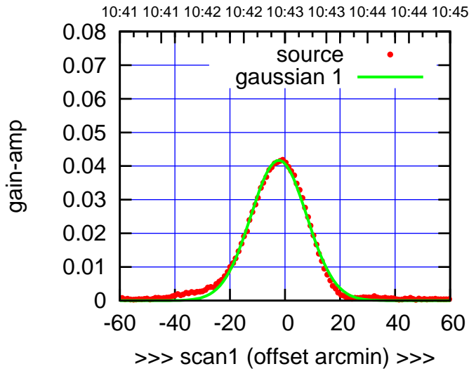
E02-130-EL OFF= -1.7' ( 23.6')
