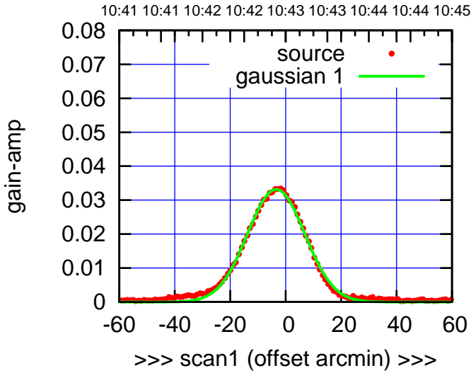
S03-130-EL OFF= -3.4' ( 24.0')
