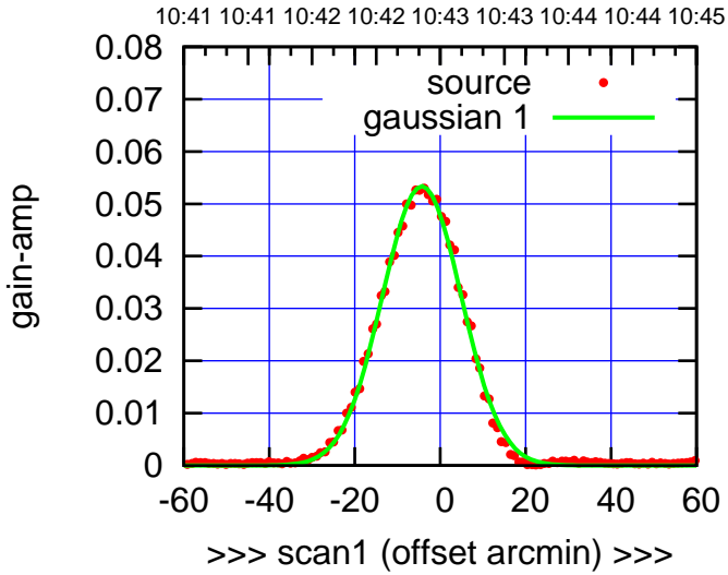
W05-130-EL OFF= -1.5' ( 22.4')
