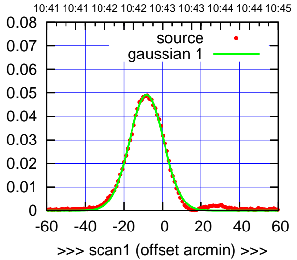
C00-175-EL OFF= -5.5' ( 22.9')
