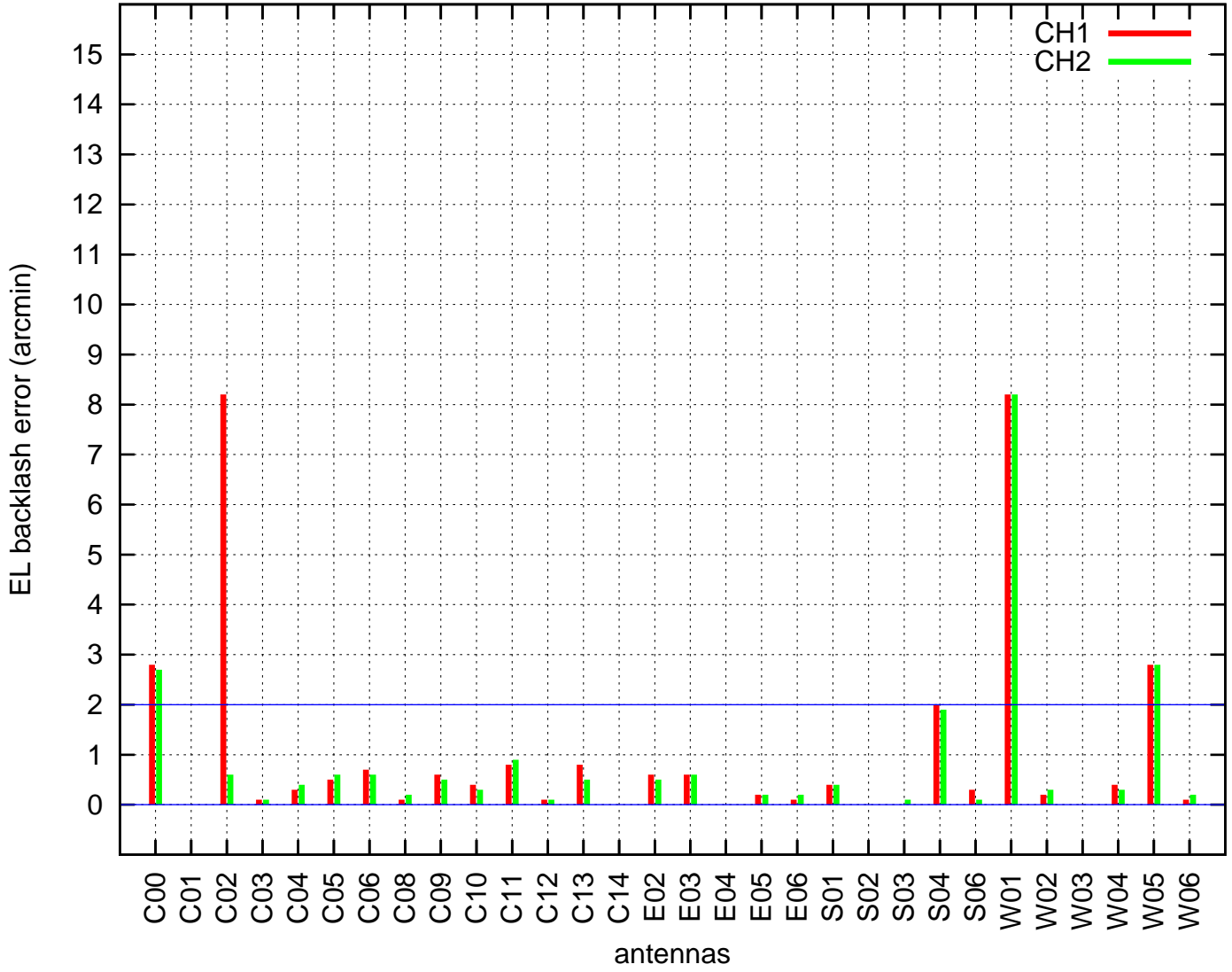
EL backlash test (18May2017 10:43:00)
