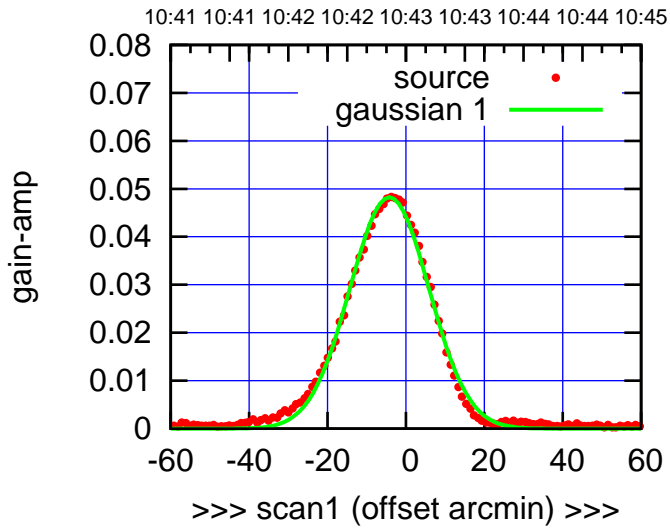
C09-130-EL OFF= -3.6' ( 23.7')
