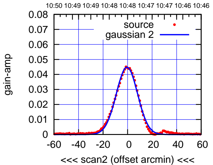
BACKLASH ERROR= 8.2'
