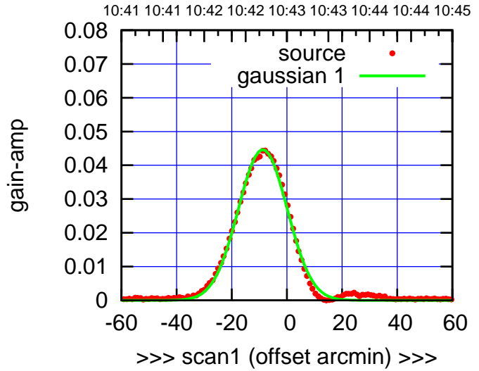
W01-175-EL OFF= -0.5' ( 20.4')
