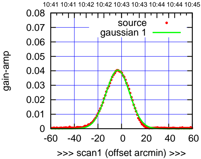
E04-130-EL OFF= -3.1' ( 23.1')
