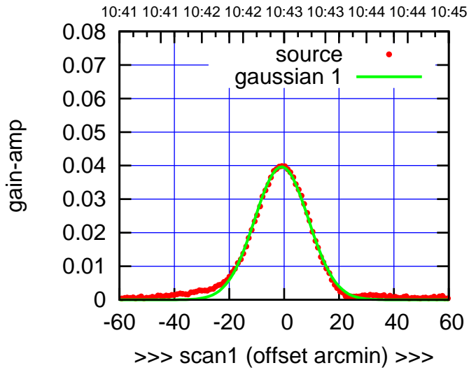
C06-130-EL OFF= -1.6' ( 23.3')
