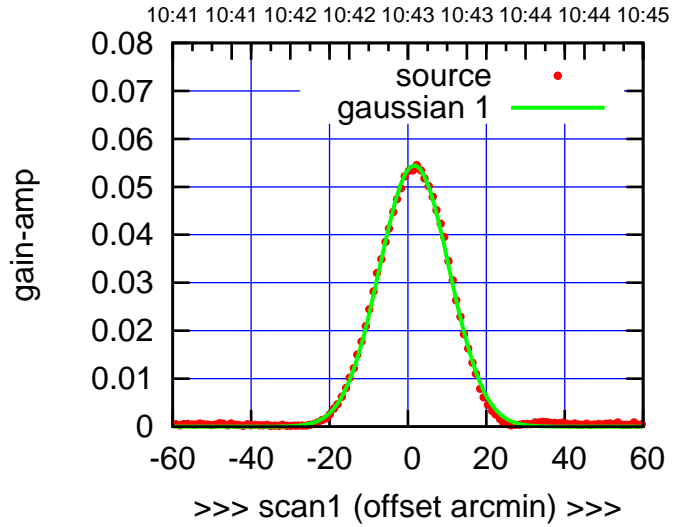
C08-175-EL OFF= 1.8' ( 20.8')
