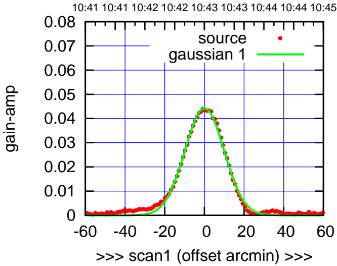
C10-130-EL OFF= -0.4' ( 23.8')
