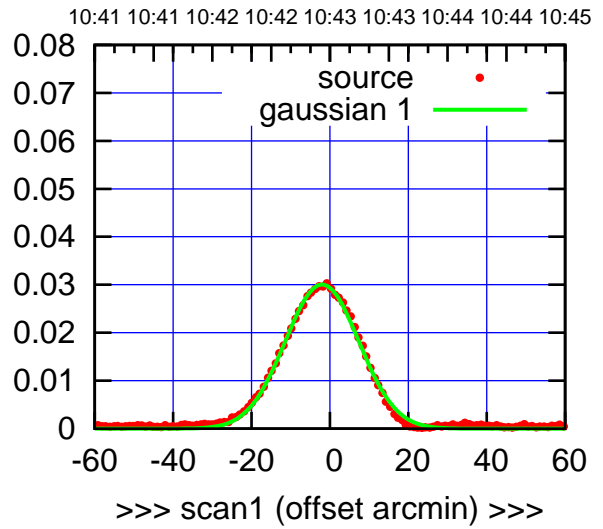
E02-175-EL OFF= -1.5' ( 22.0')
