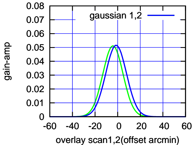
BACKLASH ERROR= 2.8'
