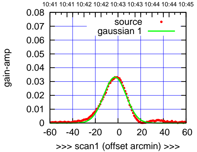
C13-175-EL OFF= -2.2' ( 23.5')
