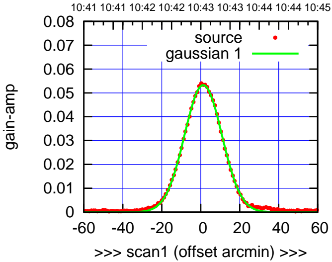
C08-130-EL OFF= 1.4' ( 22.4')
