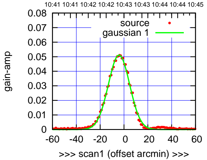
W05-175-EL OFF= -1.4' ( 21.6')
