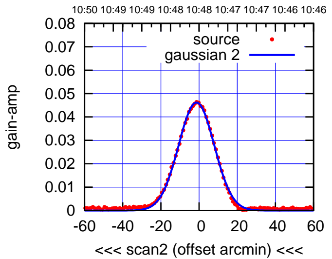
BACKLASH ERROR= 0.6'
