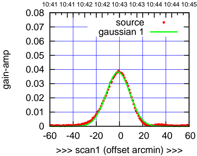
E03-130-EL OFF= -0.6' ( 24.2')
