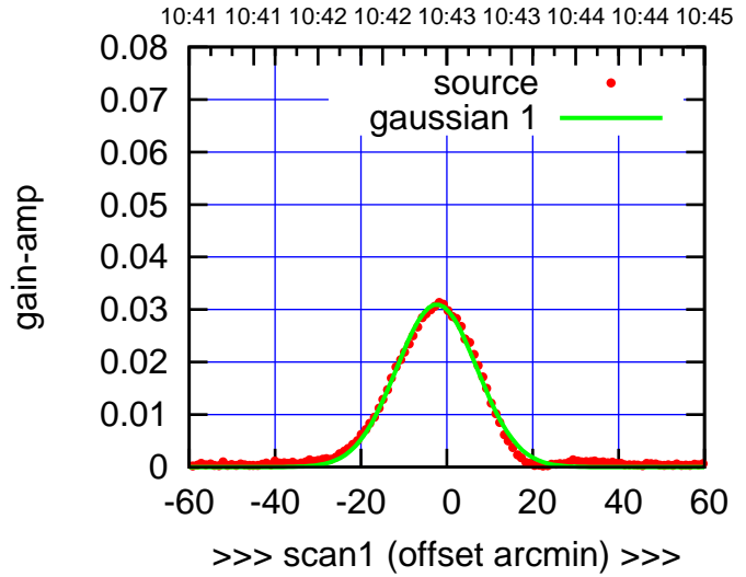
S06-175-EL OFF= -2.2' ( 22.3')
