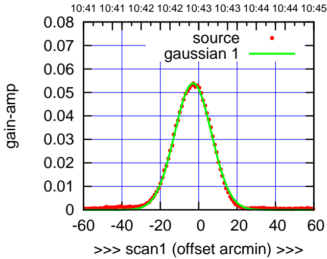
C04-130-EL OFF= -2.6' ( 22.6')
