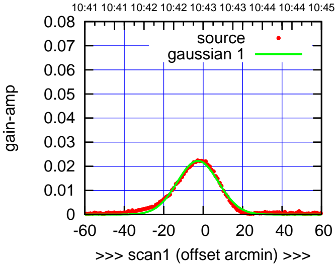
C13-130-EL OFF= -1.9' ( 24.5')
