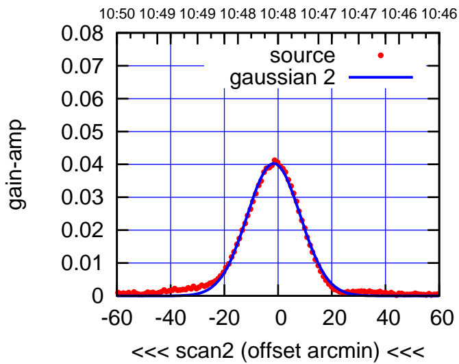
BACKLASH ERROR= 0.7'
