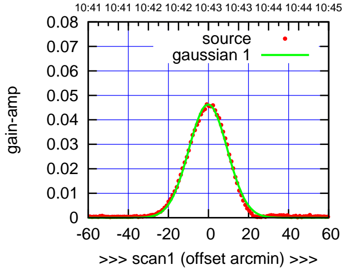
W02-175-EL OFF= 0.1' ( 22.2')
