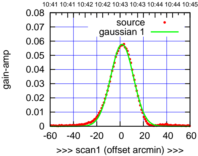
E05-130-EL OFF= 1.5' (23.0')
