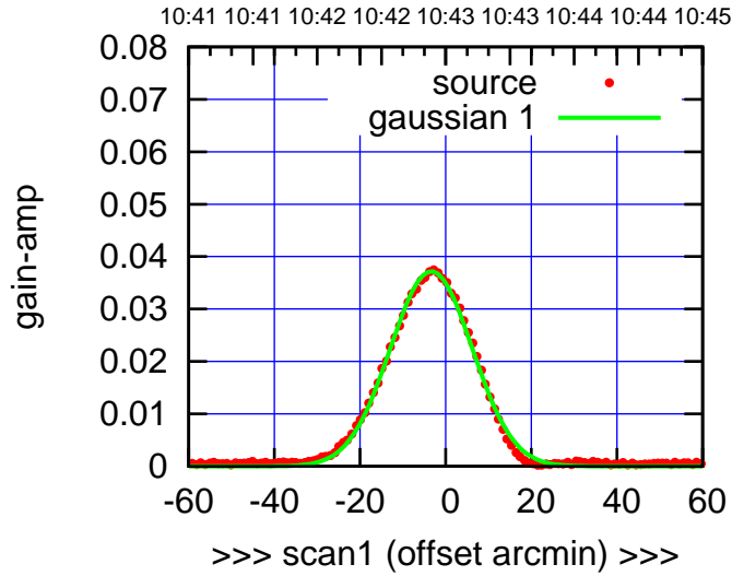
S03-175-EL OFF= -3.4' ( 22.4')
