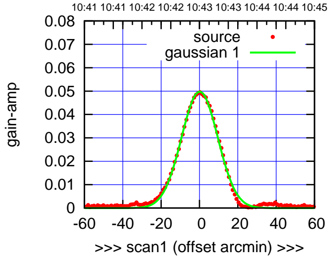
C10-175-EL OFF= -0.2' ( 22.7')
