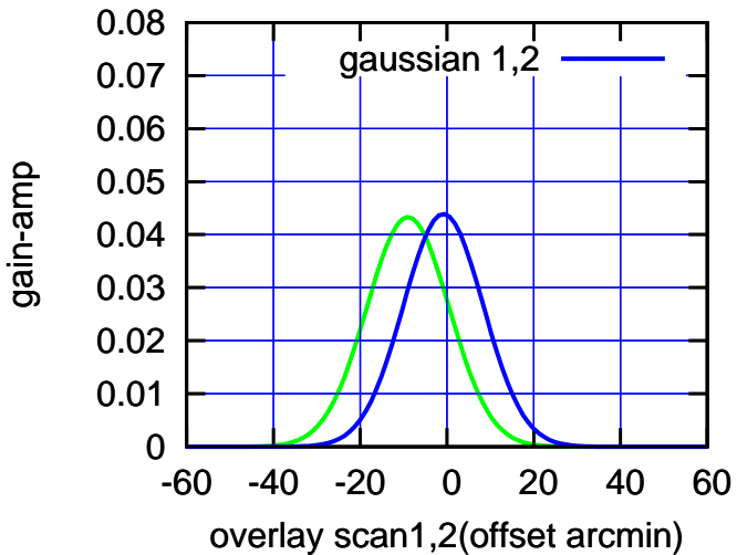
BACKLASH ERROR= 8.2'
