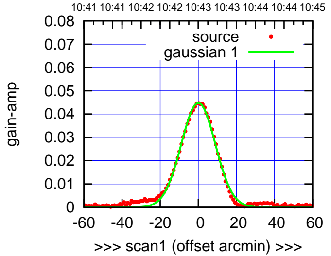
C05-175-EL OFF= -0.6' ( 21.0')
