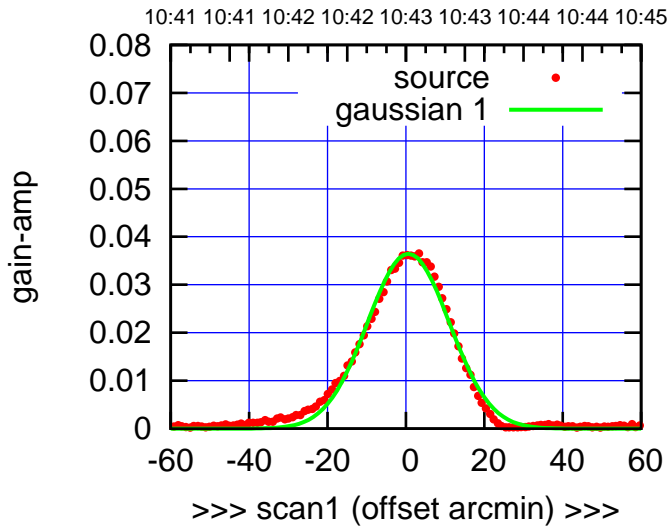
W06-130-EL OFF= 0.5' ( 24.2')
