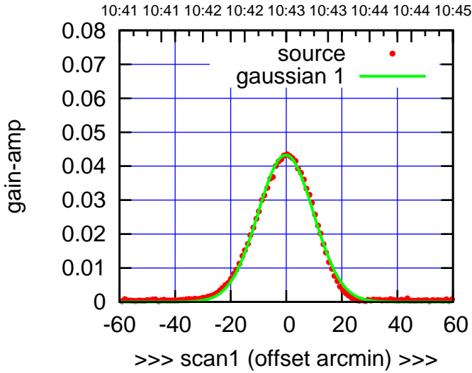
W02-130-EL OFF= -0.0' ( 23.1')
