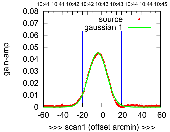
C09-175-EL OFF= -3.6' ( 21.8')
