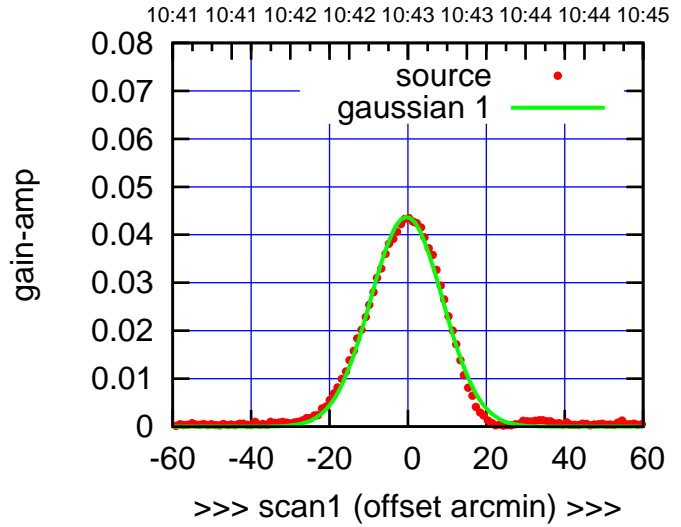
C12-175-EL OFF= -0.4' ( 21.5')
