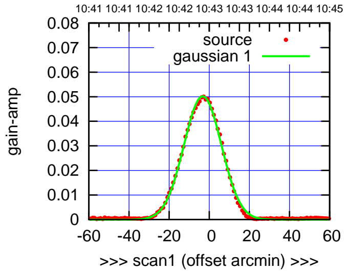
C04-175-EL OFF= -2.9' ( 21.9')
