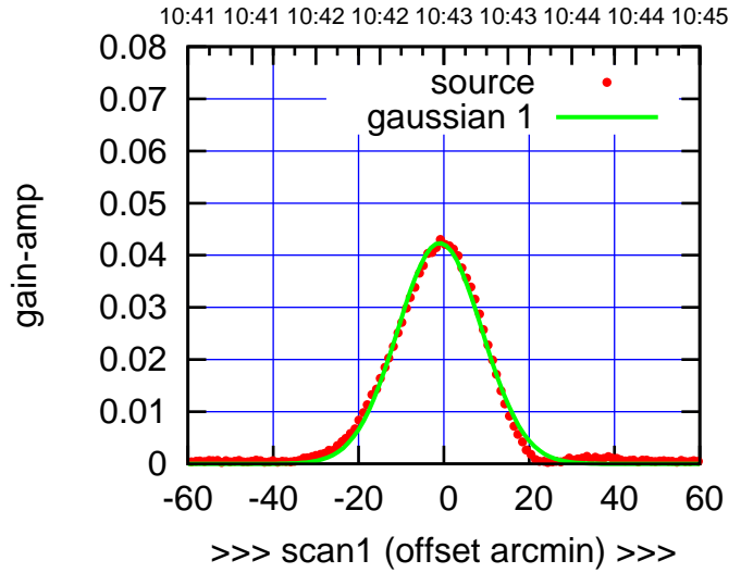
E03-175-EL OFF= -0.4' ( 23.3')
