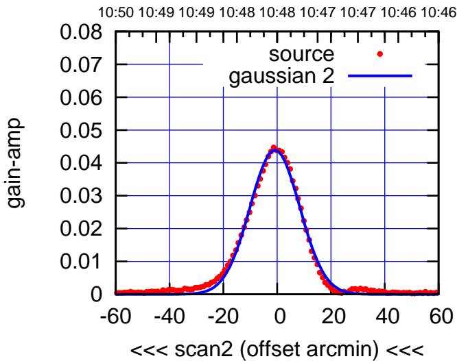
BACKLASH ERROR= 8.2'
