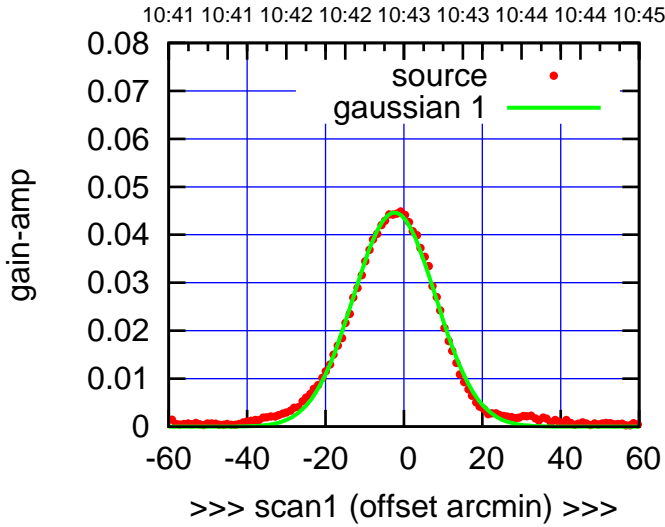
C11-130-EL OFF= -1.6' ( 24.5')
