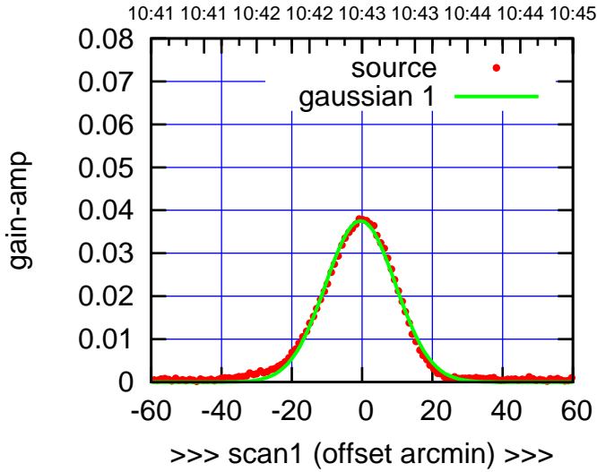
C12-130-EL OFF= -0.5' ( 23.3')
