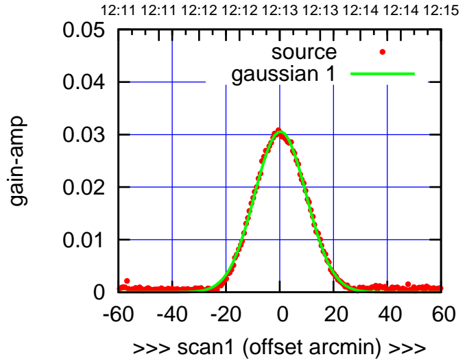
W04-175-AZ OFF= -0.4' ( 22.5')
