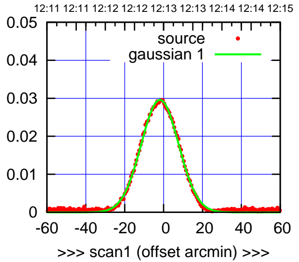
S02-175-AZ OFF= -2.2' ( 22.2')
