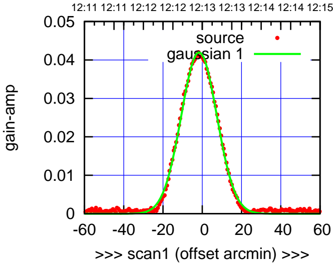
C02-130-AZ OFF= -2.2' ( 20.9')
