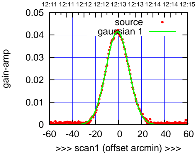
C11-130-AZ OFF= -2.0' ( 23.2')
