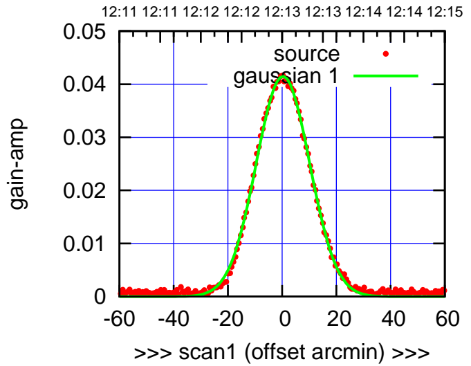
C10-175-AZ OFF= -0.5' ( 23.1')
