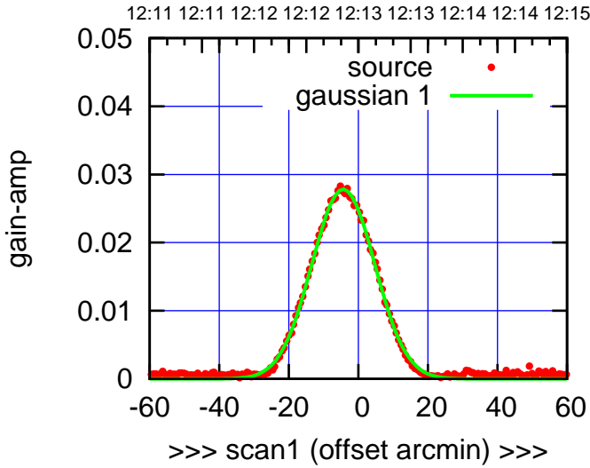
W02-130-AZ OFF= -4.1' ( 21.2')
