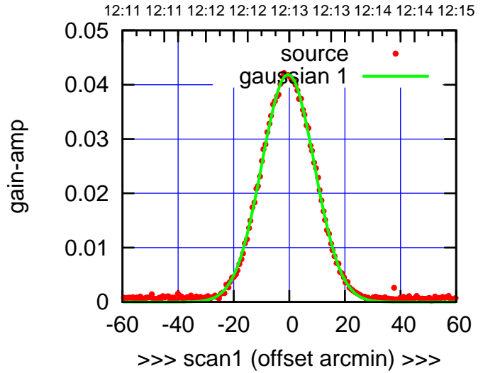
W01-175-AZ OFF= -1.6' ( 22.1')
