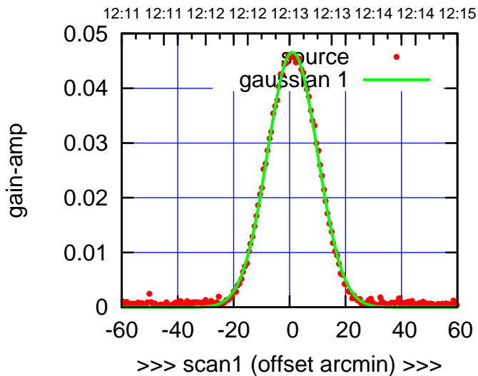
W05-130-AZ OFF= 0.4' ( 20.9')
