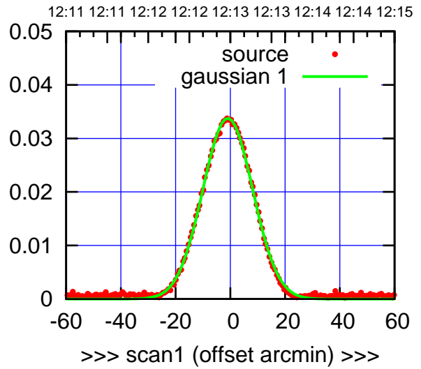
E05-175-AZ OFF= -1.7' ( 21.5')
