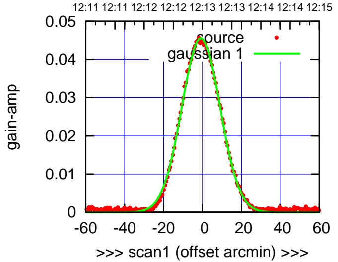
C11-175-AZ OFF= -2.0' ( 23.1')
