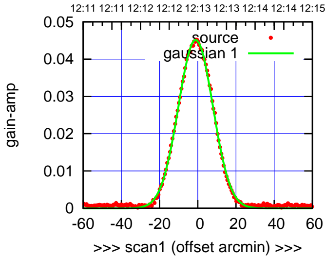
E05-130-AZ OFF= -1.8' ( 21.5')
