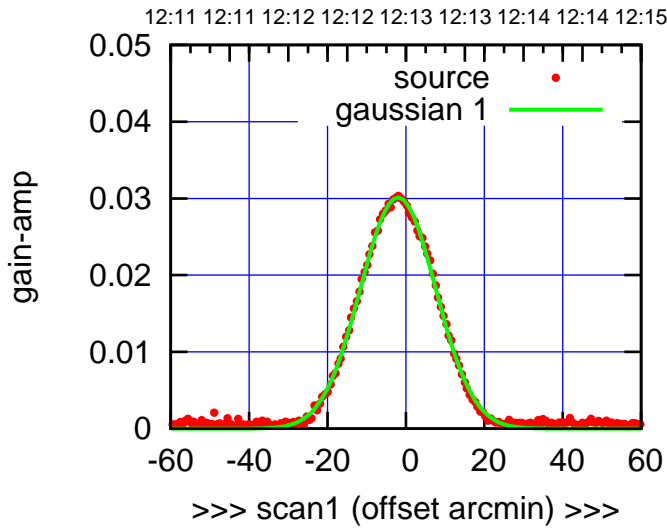
S02-130-AZ OFF= -2.3' ( 22.2')
