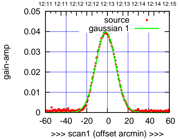
C02-175-AZ OFF= -2.1' ( 21.8')
