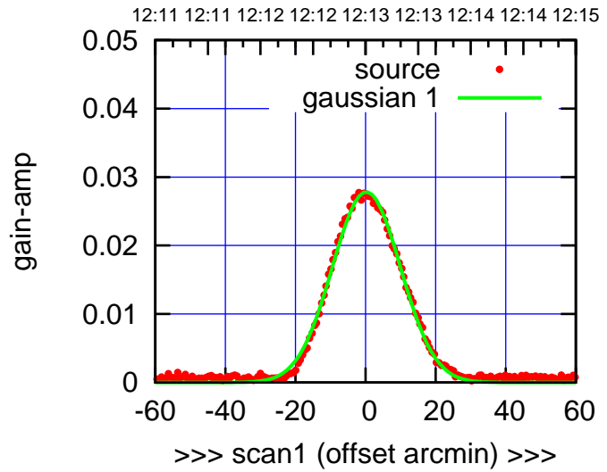
C14-175-AZ OFF= -0.6' ( 22.9')
