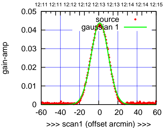
W05-175-AZ OFF= 0.5' ( 21.0')
