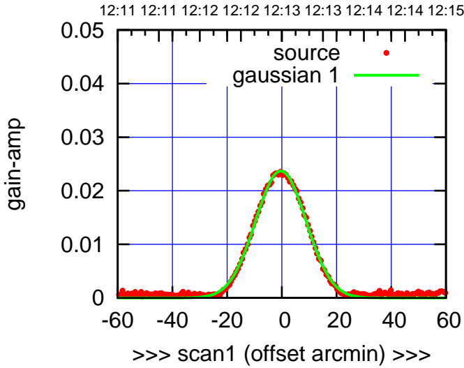
W01-130-AZ OFF= -1.5' ( 21.6')
