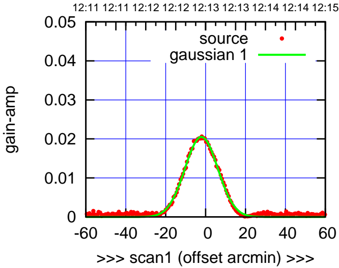
W06-130-AZ OFF= -2.7' ( 19.2')
