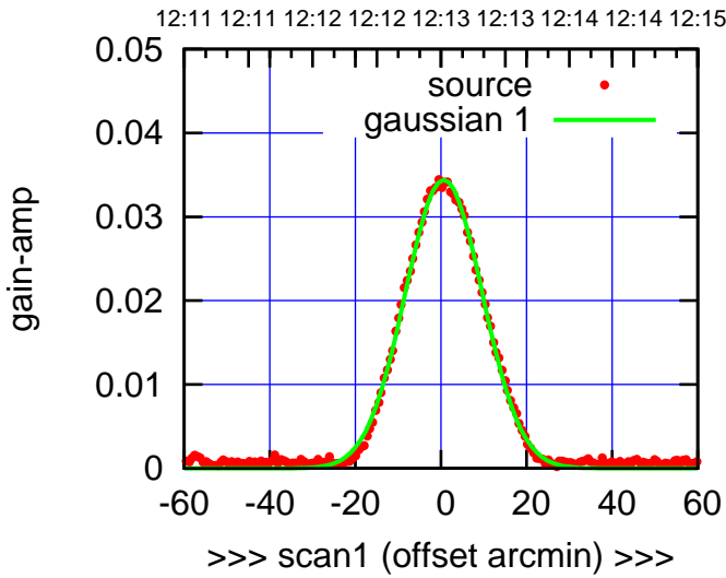
C12-130-AZ OFF= -0.3' ( 21.2')
