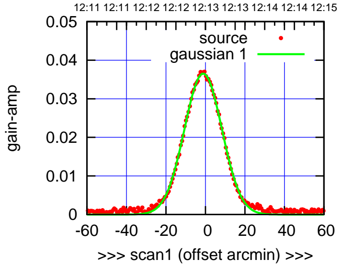
C05-175-AZ OFF= -2.0' ( 22.2')
