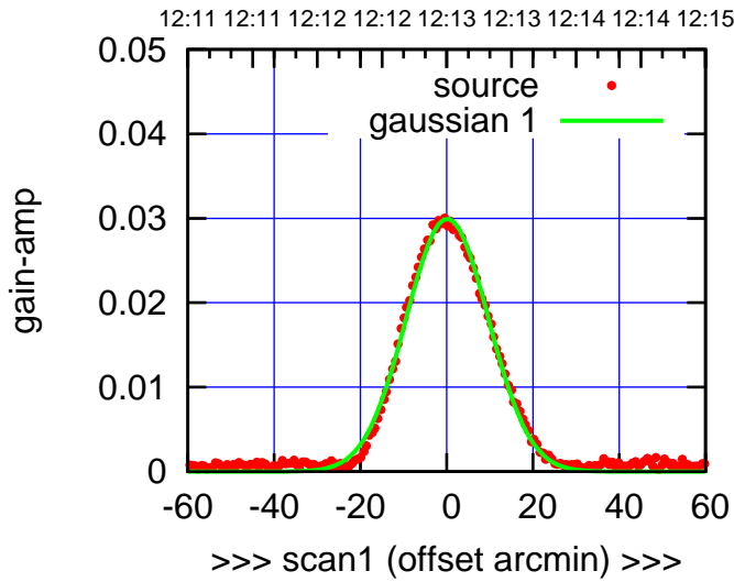
C14-130-AZ OFF= -0.5' ( 22.7')
