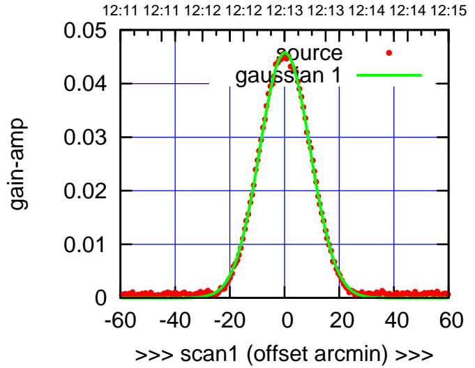
W03-175-AZ OFF= -0.5' ( 21.8')
