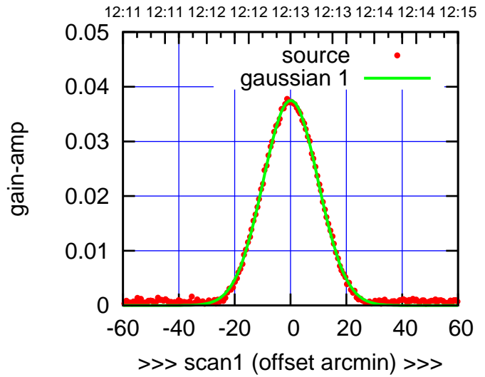
C13-175-AZ OFF= -1.2' ( 23.1')
