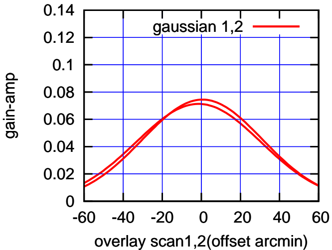
BACKLASH ERROR= 3.4'
