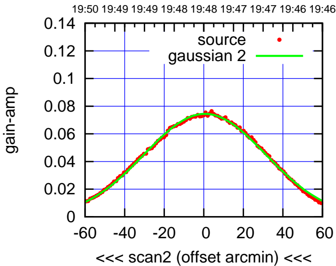
BACKLASH ERROR= 3.4'
