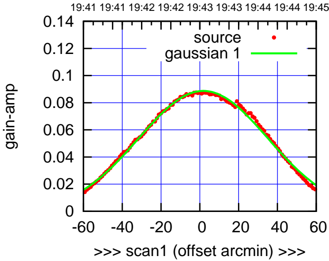
W02-130-AZ OFF= 0.8'
