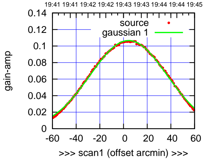
W06-175-AZ OFF= 3.3'
