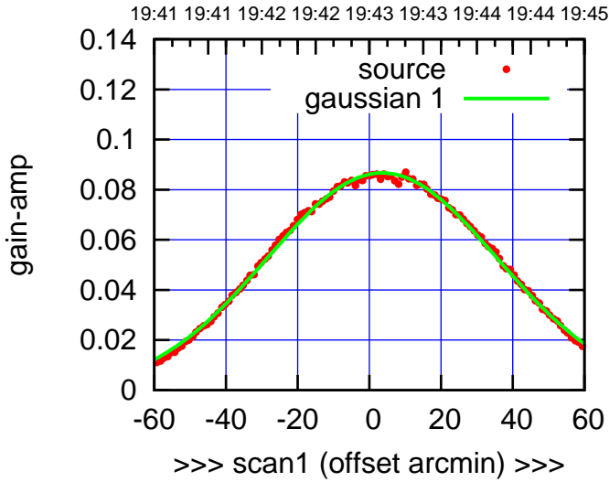
C02-130-AZ OFF= 3.4'
