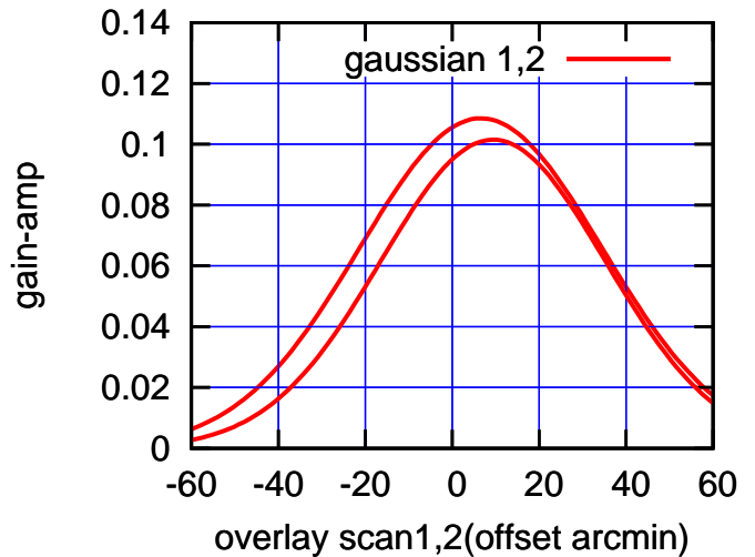
BACKLASH ERROR= 4.8'
