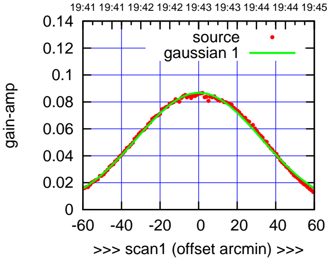
C00-130-AZ OFF= -1.6'
