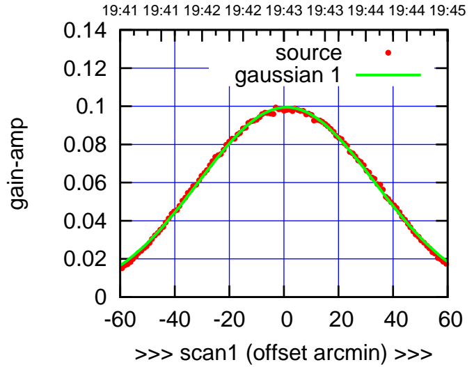
C11-175-AZ OFF= 0.3'
