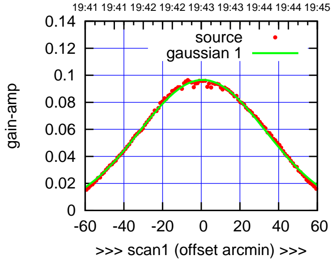
C12-175-AZ OFF= -0.2'
