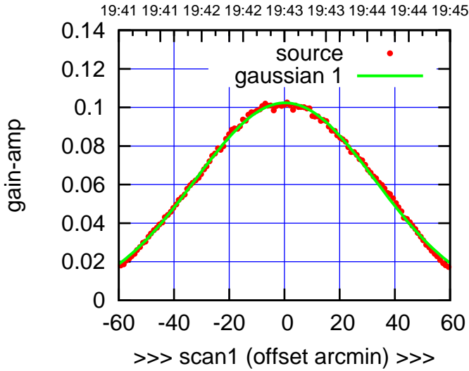
C12-130-AZ OFF= -0.7'
