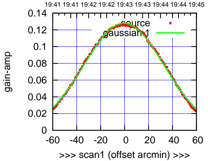
W01-175-AZ OFF= -1.5'
