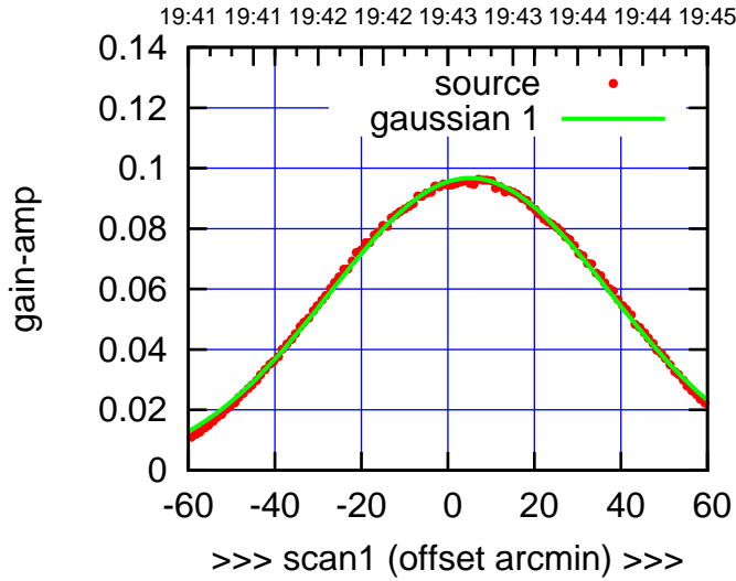
W06-130-AZ OFF= 4.3'
