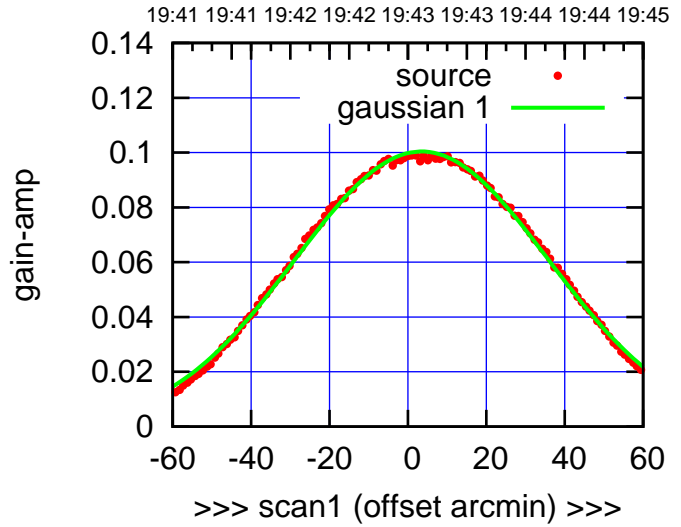
C02-175-AZ OFF= 3.3'
