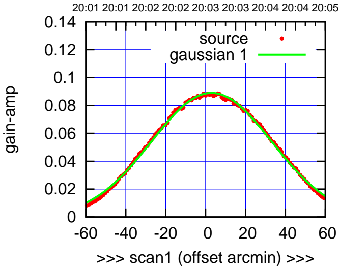
C02-130-AZ OFF= 2.6'
