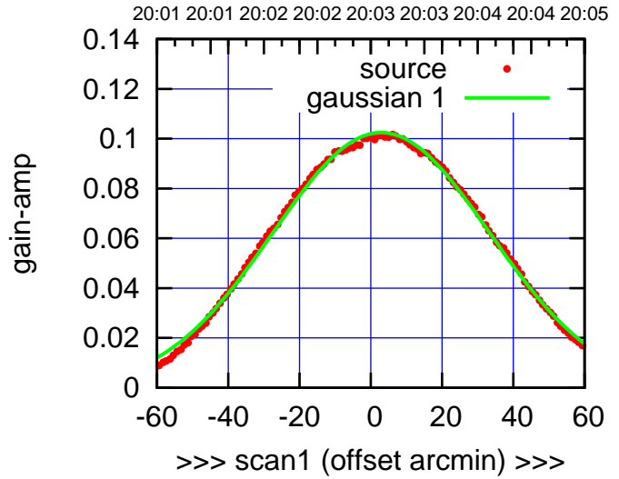
C02-175-AZ OFF= 2.5'
