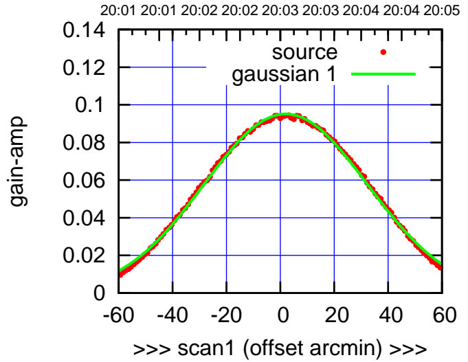
W02-175-AZ OFF= 2.4'
