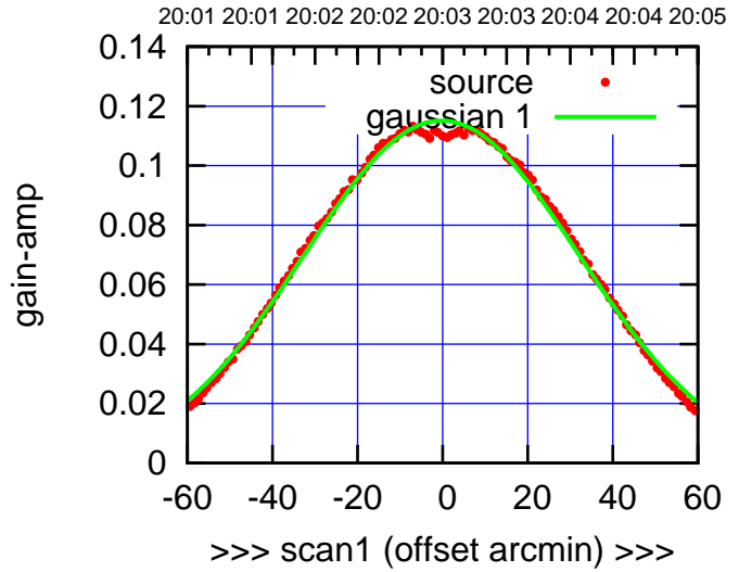
S03-175-AZ OFF= -0.6'
