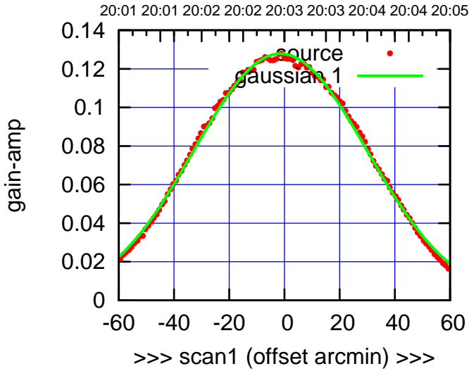
C10-130-AZ OFF= -1.7'
