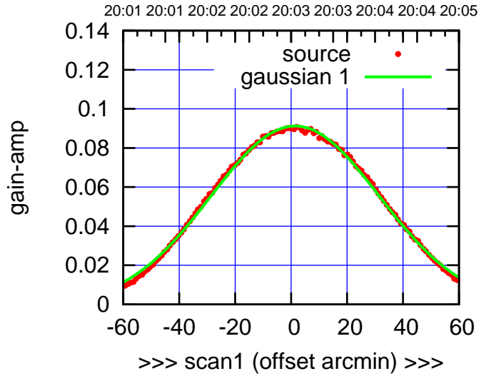
C00-175-AZ OFF= 0.5'
