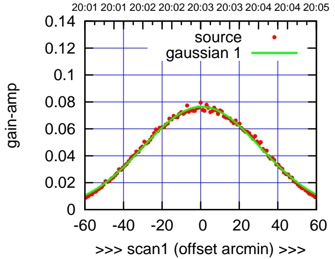
W05-175-AZ OFF= 0.4'
