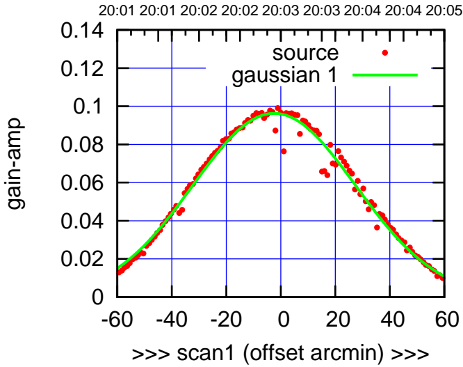
C14-130-AZ OFF= -2.1'
