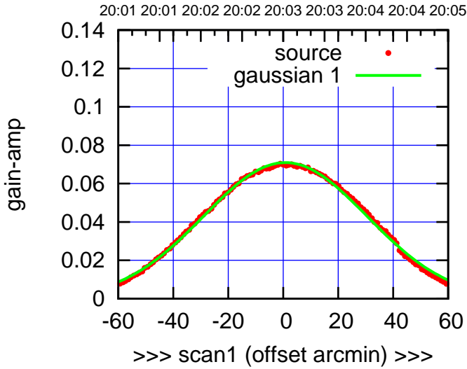
E05-130-AZ OFF= 0.6'
