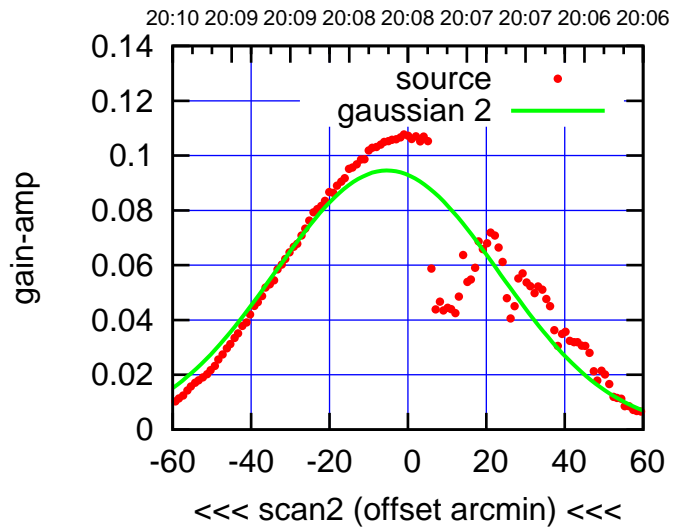
BACKLASH ERROR= 8.9'
