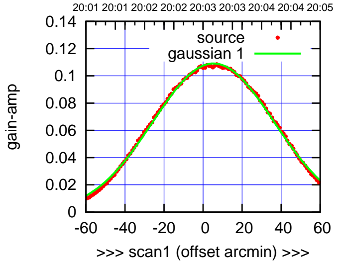
S01-175-AZ OFF= 4.5'
