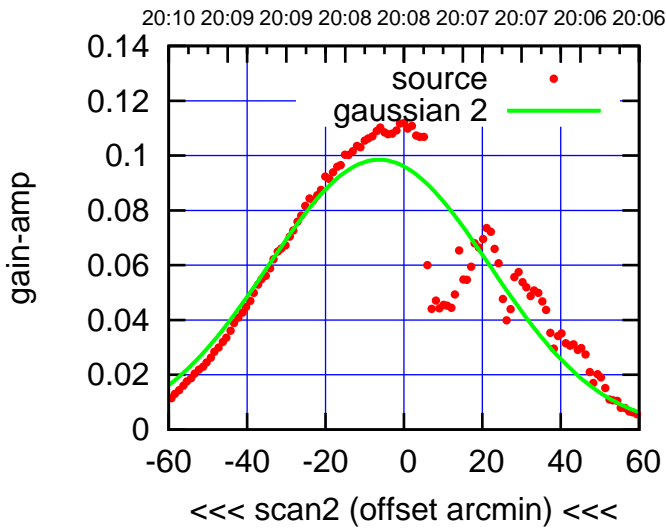
BACKLASH ERROR= 8.1'
