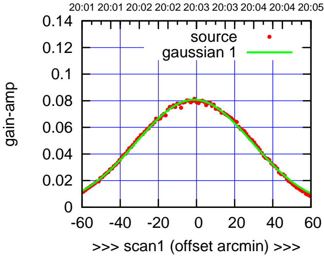
C00-130-AZ OFF= -2.2'
