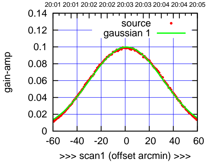
C11-175-AZ OFF= 0.9'
