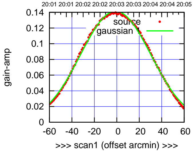
C10-175-AZ OFF= -1.4'
