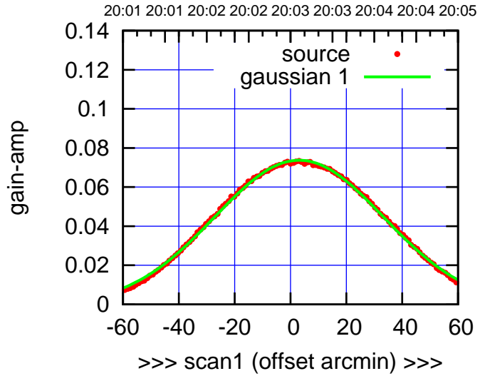
S04-175-AZ OFF= 2.7'
