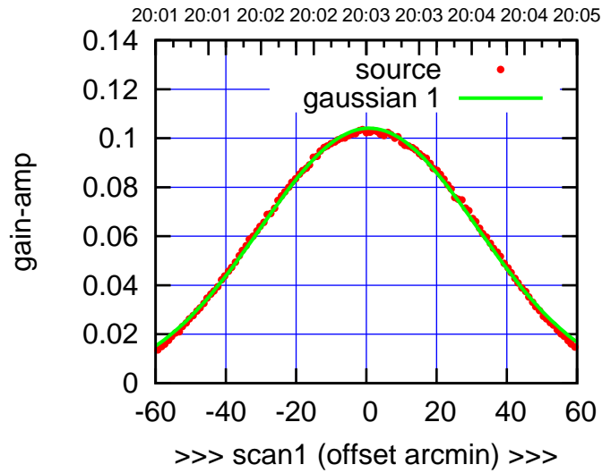
W03-175-AZ OFF= 0.3'
