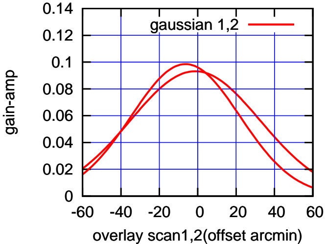
BACKLASH ERROR= 8.1'
