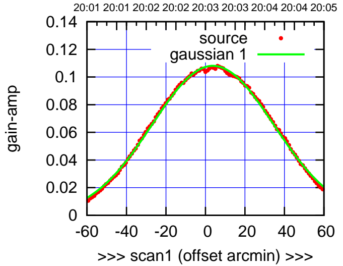
W06-175-AZ OFF= 3.5'
