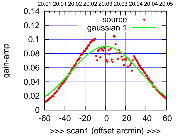
C06-175-AZ OFF= -5.3'
