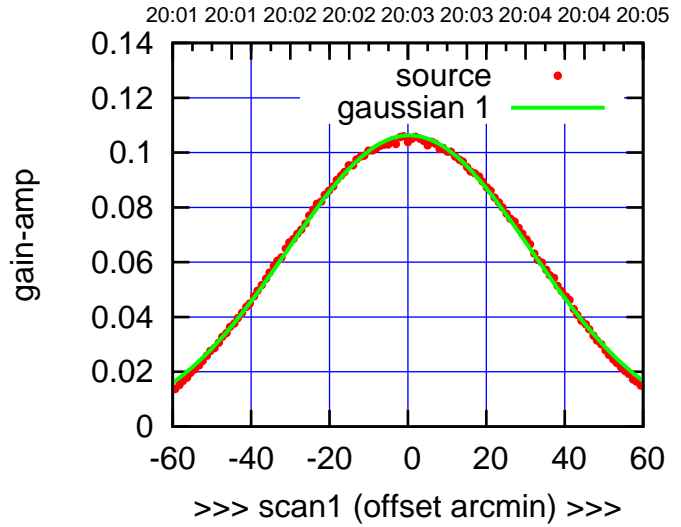
S02-175-AZ OFF= 0.3'
