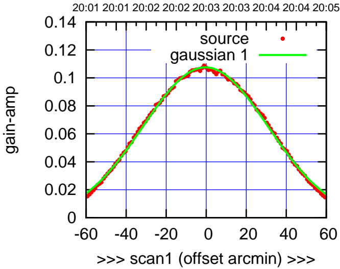
S02-130-AZ OFF= -0.4'
