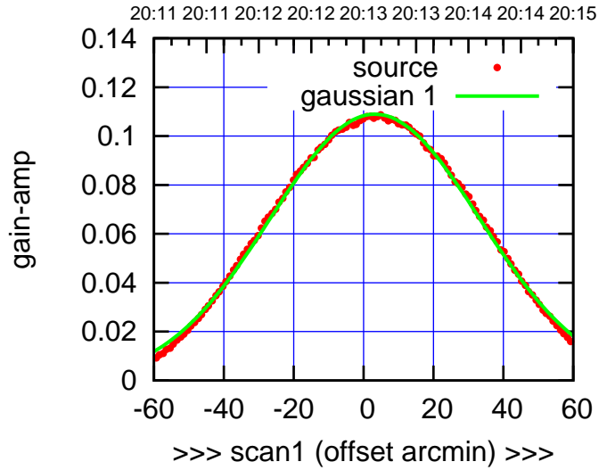
W06-175-AZ OFF= 3.0'
