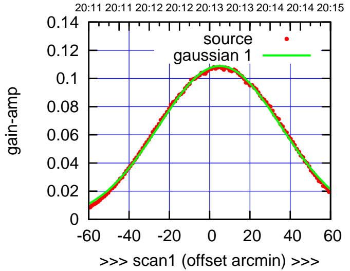
S01-175-AZ OFF= 3.9'
