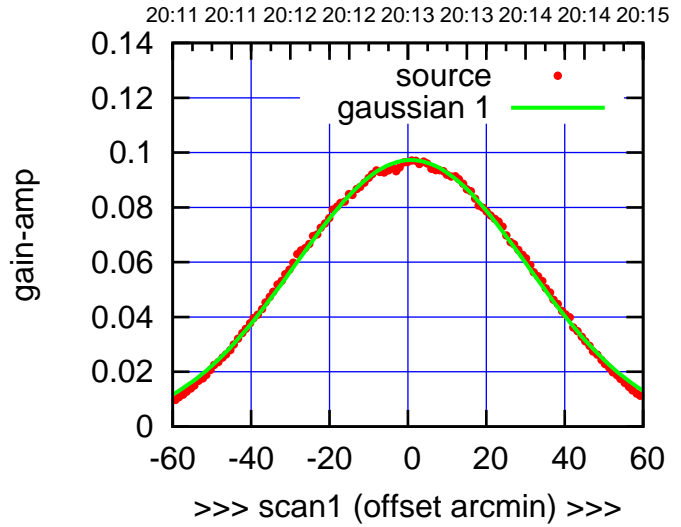
E05-175-AZ OFF= 0.4'
