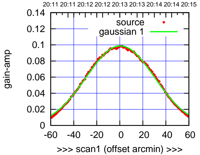
C12-175-AZ OFF= 0.0'
