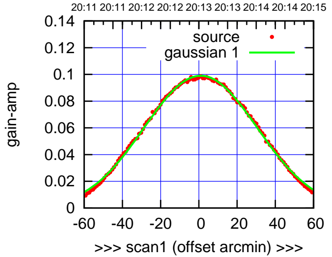
C11-175-AZ OFF= 0.8'
