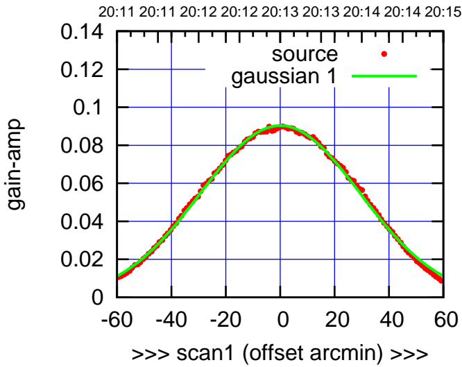
W05-130-AZ OFF= -0.1'
