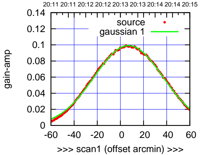
C04-175-AZ OFF= 6.4'
