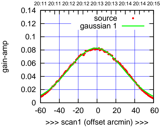
C00-130-AZ OFF= -2.3'
