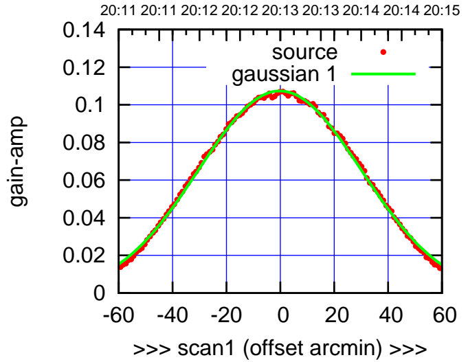
S02-175-AZ OFF= -0.2'
