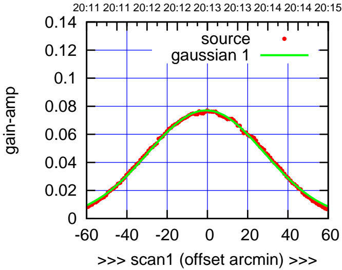
C08-130-AZ OFF= -0.4'
