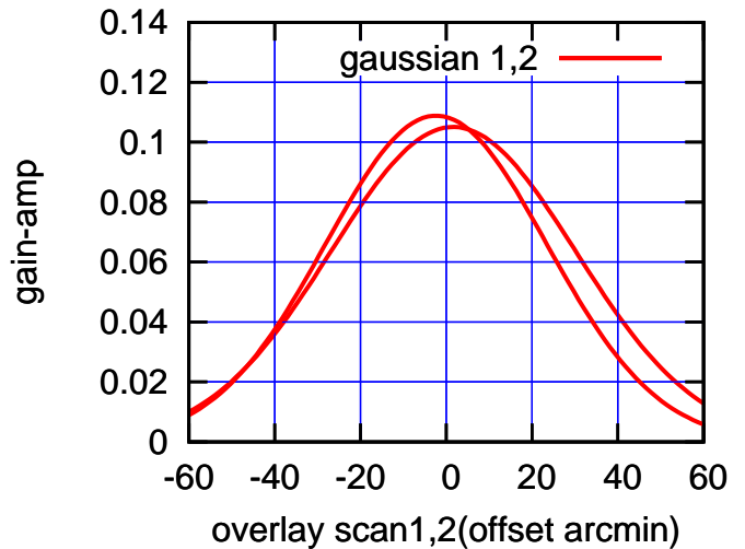
BACKLASH ERROR= 6.3'
