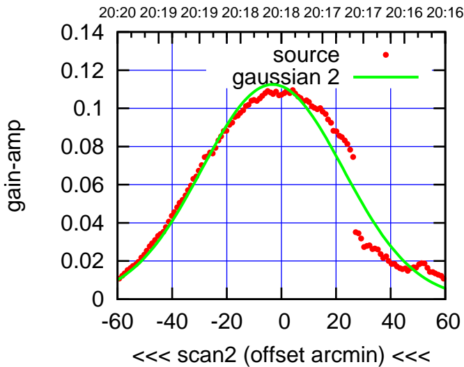
BACKLASH ERROR= 6.0'
