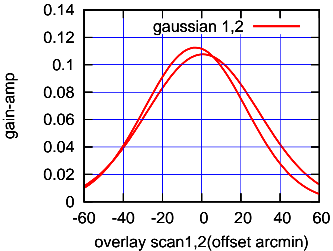
BACKLASH ERROR= 6.0'
