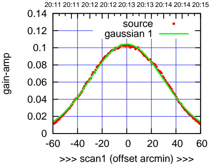
C12-130-AZ OFF= -0.5'
