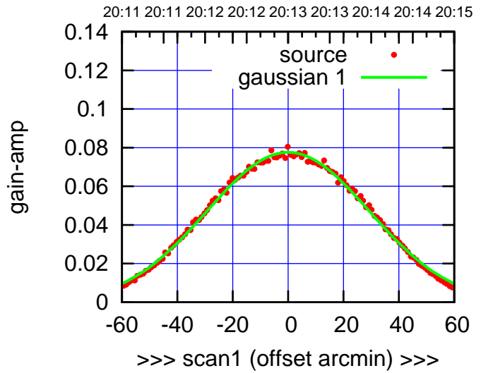
W05-175-AZ OFF= -0.0'
