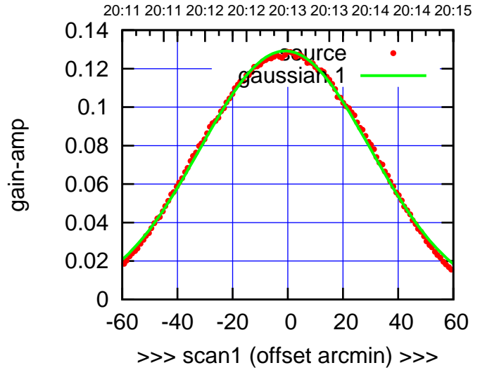
W01-175-AZ OFF= -1.3'
