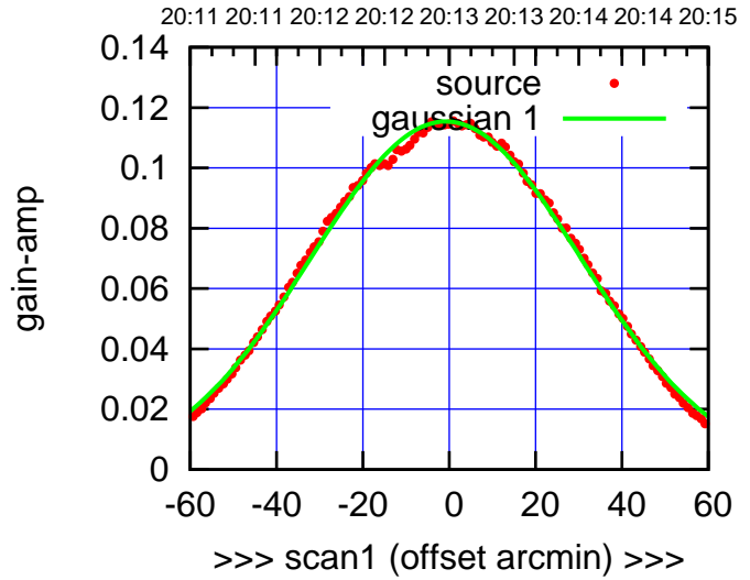
S03-175-AZ OFF= -1.1'
