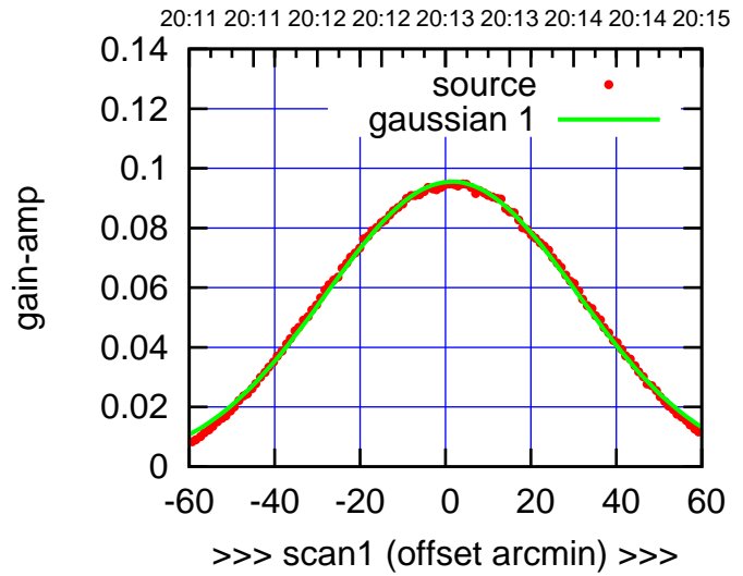
W02-175-AZ OFF= 1.7'
