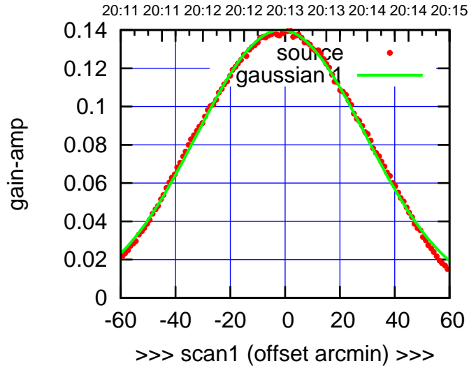
C10-175-AZ OFF= -1.6'
