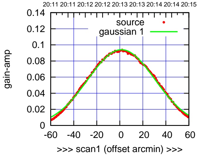
C00-175-AZ OFF= 0.2'
