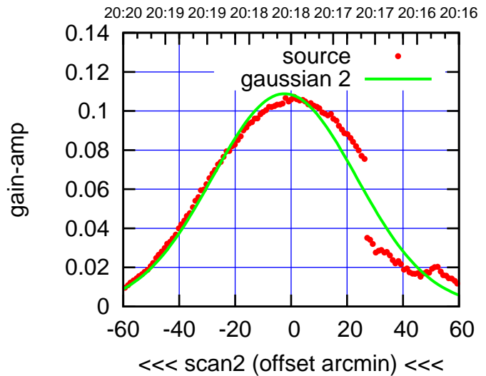
BACKLASH ERROR= 6.3'
