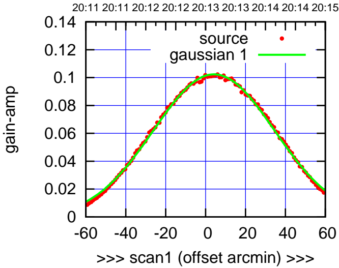
S01-130-AZ OFF= 2.9'
