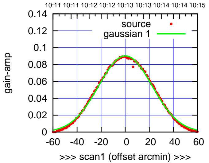
E04-175-AZ OFF= -0.4' ( 52.0')
