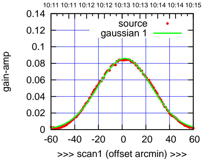
C12-130-AZ OFF= 1.4' ( 53.2')
