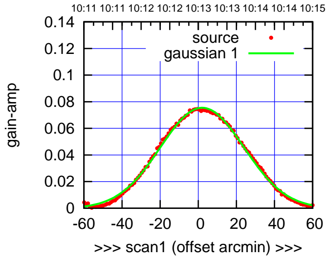
C14-175-AZ OFF= 1.6' ( 51.4')
