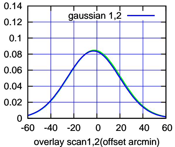
BACKLASH ERROR= 0.7'
