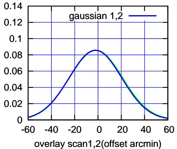
BACKLASH ERROR= 0.5'
