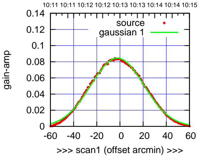
S03-130-AZ OFF= -2.9' ( 53.4')
