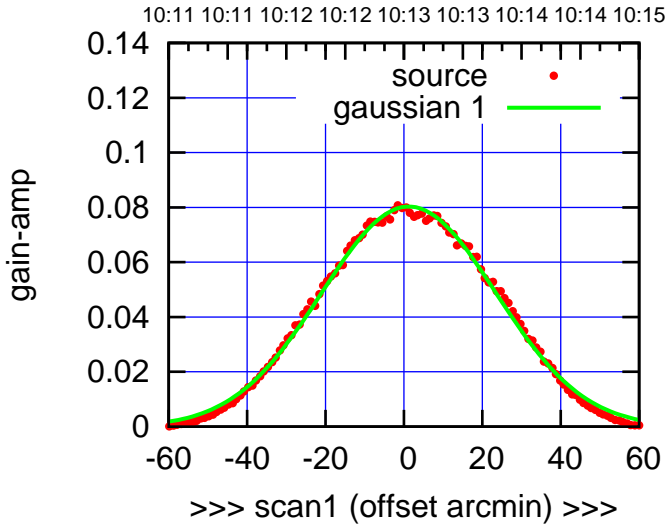
W02-130-AZ OFF= 1.8' ( 51.7')
