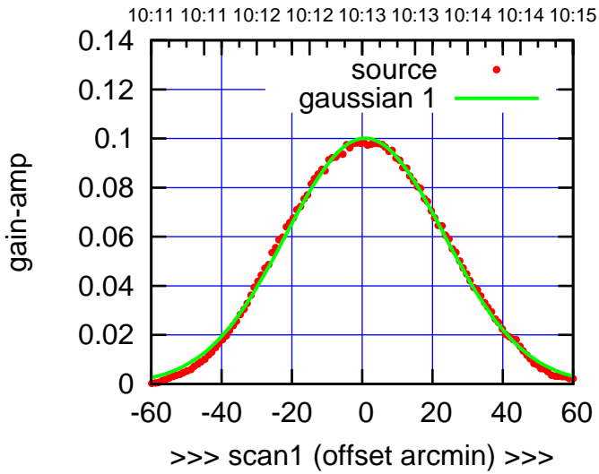
C10-130-AZ OFF= 0.3' (53.0')
