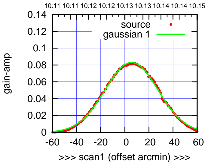
W06-130-AZ OFF= 4.9' ( 51.8')
