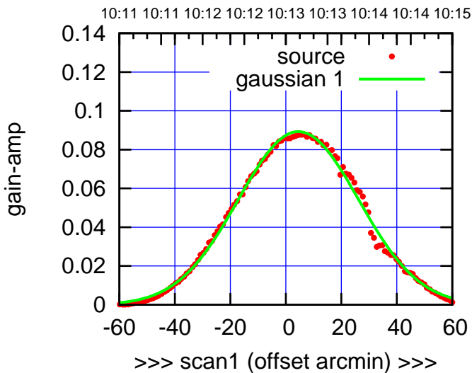
W06-175-AZ OFF= 4.3' ( 52.2')
