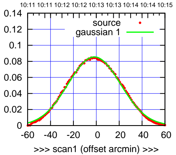
S06-175-AZ OFF= -2.2' ( 53.0')
