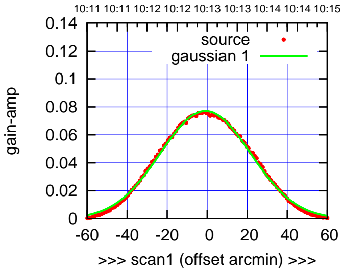
S06-130-AZ OFF= -1.3' ( 52.6')
