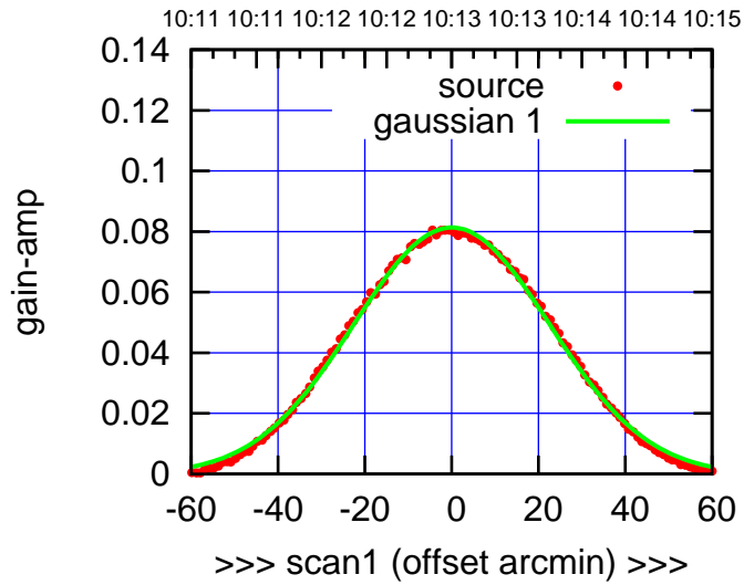
S02-175-AZ OFF= 0.5' ( 52.6')
