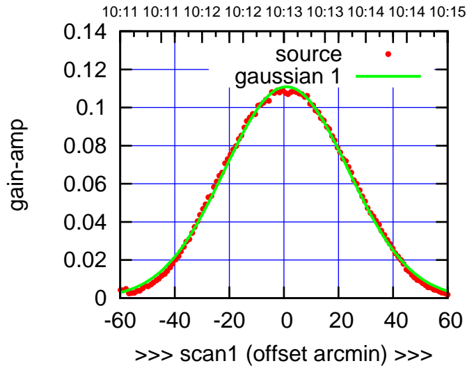
C10-175-AZ OFF= 0.6' (53.3')
