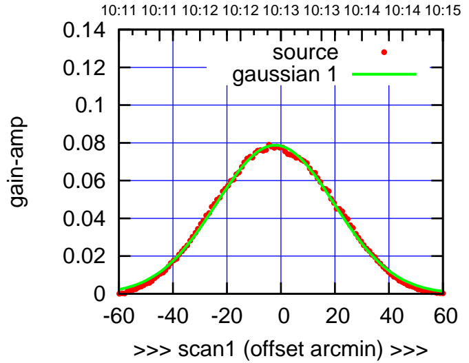
W05-175-AZ OFF= -1.8' ( 51.1')
