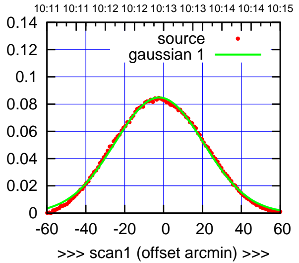
S03-175-AZ OFF= -2.9' ( 53.6')
