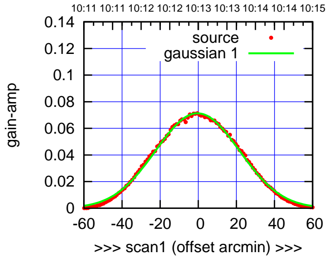
E05-175-AZ OFF= -1.1' ( 51.6')
