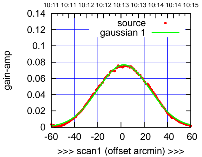
C12-175-AZ OFF= 2.0' ( 52.2')
