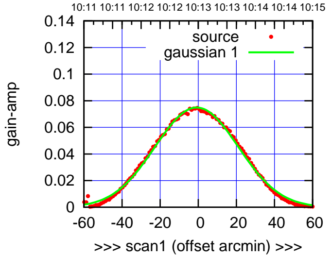
C00-175-AZ OFF= -1.6' ( 50.6')
