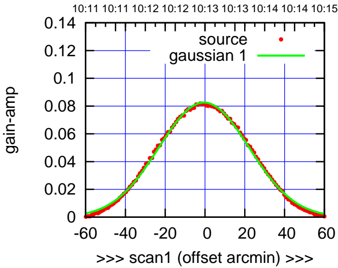
S02-130-AZ OFF= -0.0' ( 52.9')
