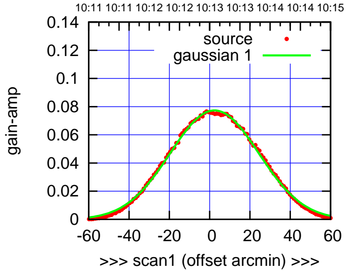
W02-175-AZ OFF= 2.9' ( 51.3')
