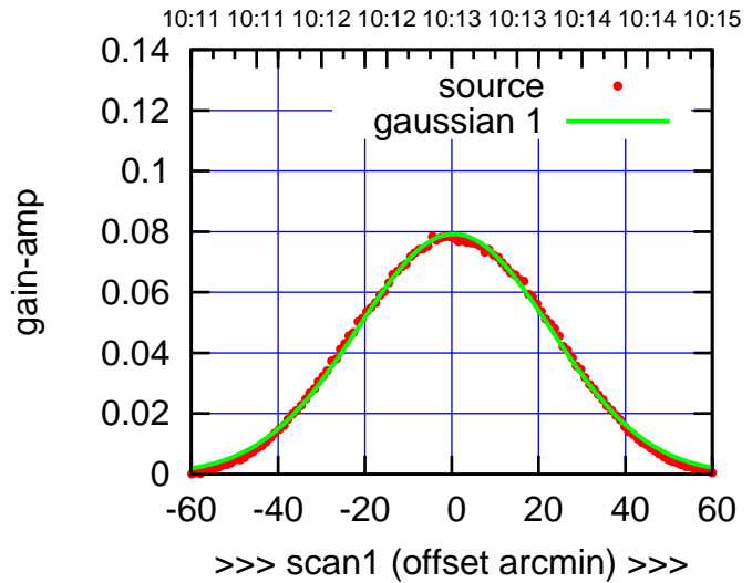
W03-175-AZ OFF= 0.2' ( 52.0')
