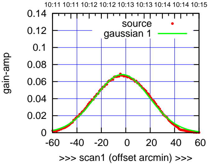
C00-130-AZ OFF= -3.7' ( 51.8')
