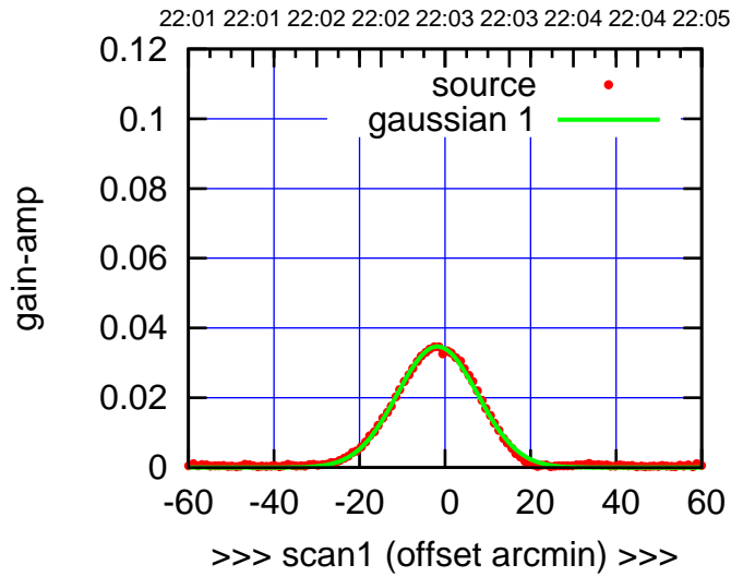
S01-175-EL OFF= -1.6' ( 22.2')
