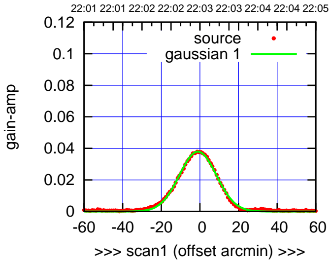
C08-130-EL OFF= -0.5' ( 23.1')
