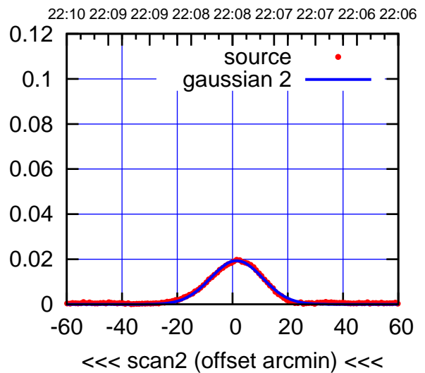
BACKLASH ERROR= 2.6'
