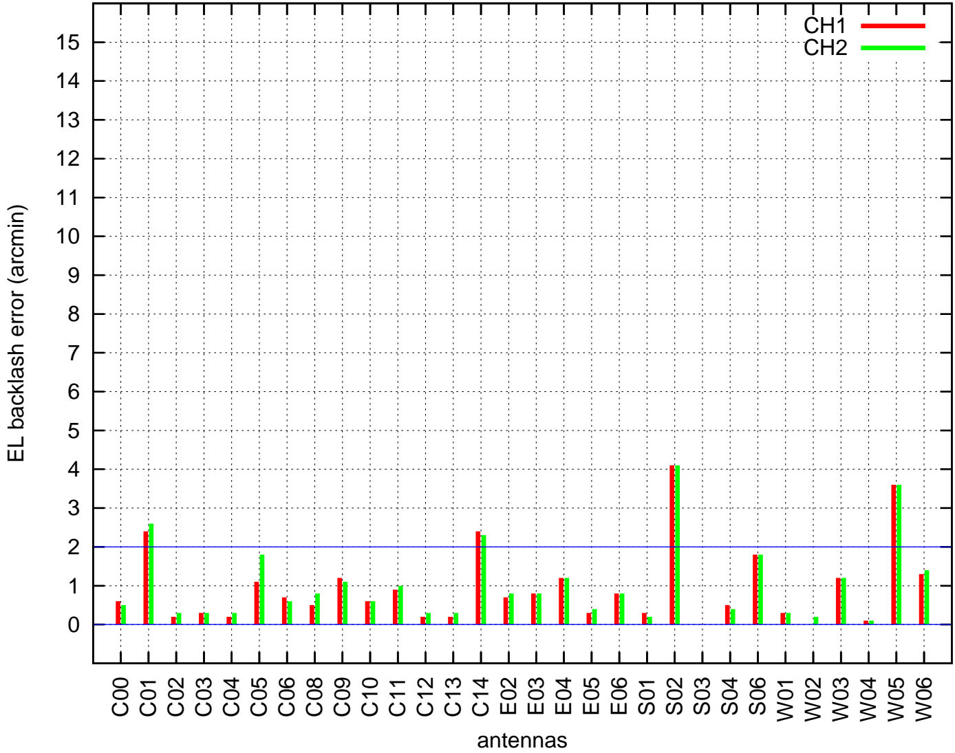
EL backlash test (25Jul2018 22:03:00)
