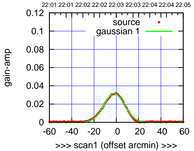
C12-175-EL OFF= -2.1' ( 21.6')
