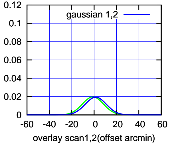
BACKLASH ERROR= 2.6'
