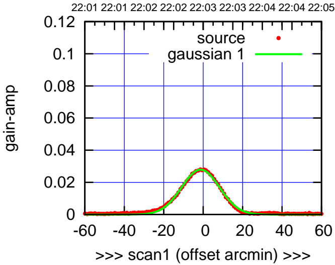
E04-130-EL OFF= -0.1' ( 22.9')
