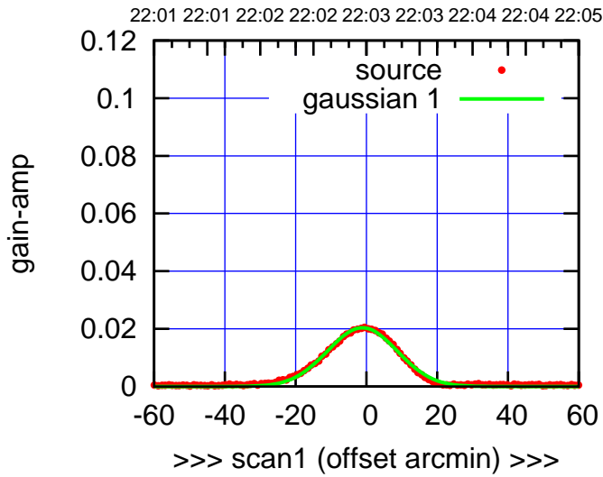
C01-130-EL OFF= 1.3' ( 22.9')
