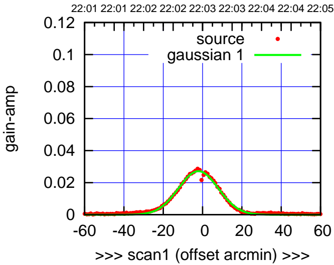
S01-130-EL OFF= -1.8' ( 23.6')
