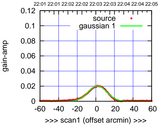
C10-130-EL OFF= 1.3' ( 23.5')
