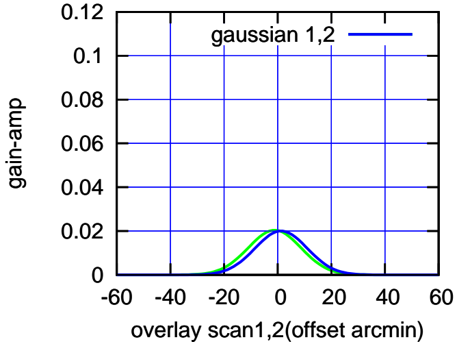
BACKLASH ERROR= 2.4'
