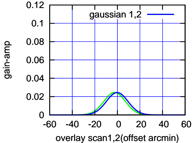
BACKLASH ERROR= 2.3'
