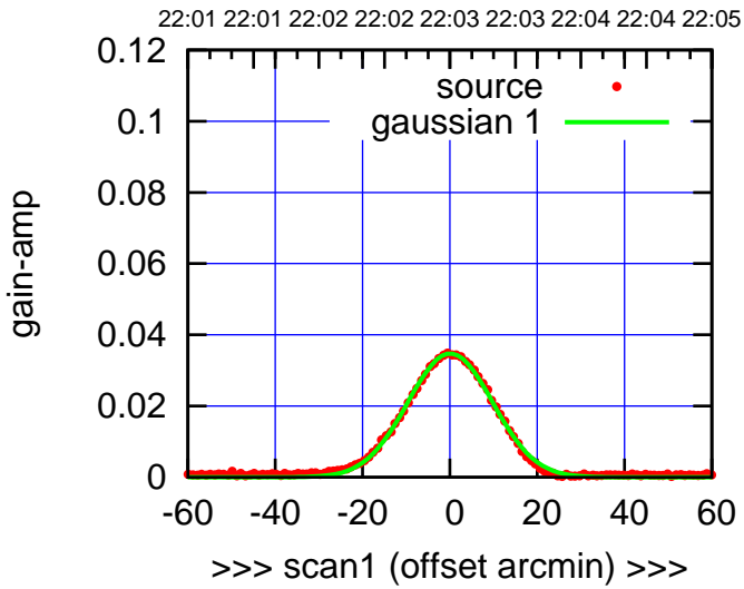
C04-130-EL OFF= 0.3' ( 22.6')
