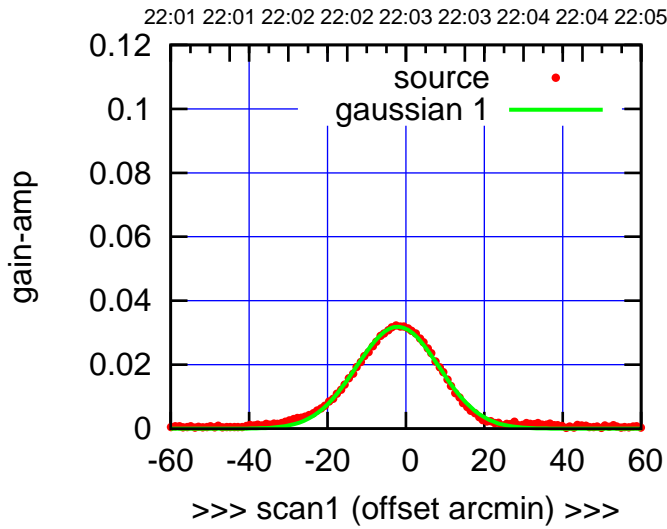
C11-130-EL OFF= -1.2' ( 25.0')
