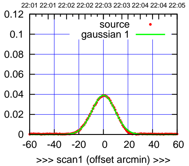
C04-175-EL OFF= 0.4' ( 21.9')
