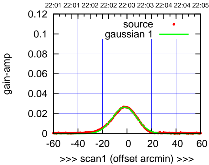
C12-130-EL OFF= -2.1' ( 23.4')
