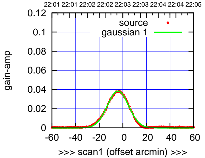
W05-175-EL OFF= -0.5' ( 21.2')
