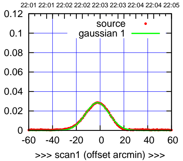
C11-175-EL OFF= -1.3' ( 23.2')
