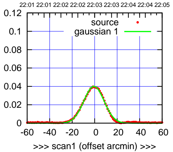
C08-175-EL OFF= 0.2' ( 21.3')
