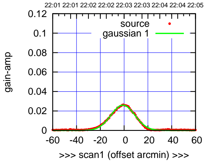
E03-175-EL OFF= -0.2' ( 23.5')
