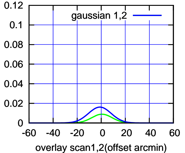
BACKLASH ERROR= 1.8'
