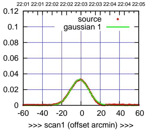
S04-175-EL OFF= -1.8' ( 22.2')
