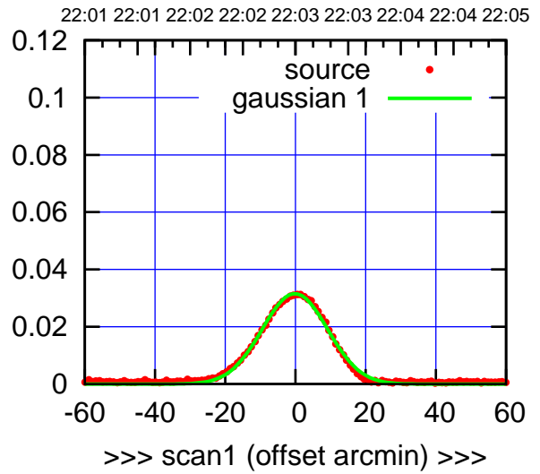
C06-175-EL OFF= -0.8' ( 21.9')
