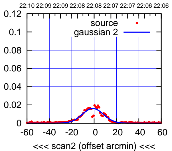
BACKLASH ERROR= 1.8'
