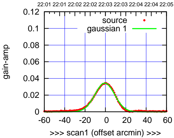
W01-130-EL OFF= -0.3' ( 22.5')
