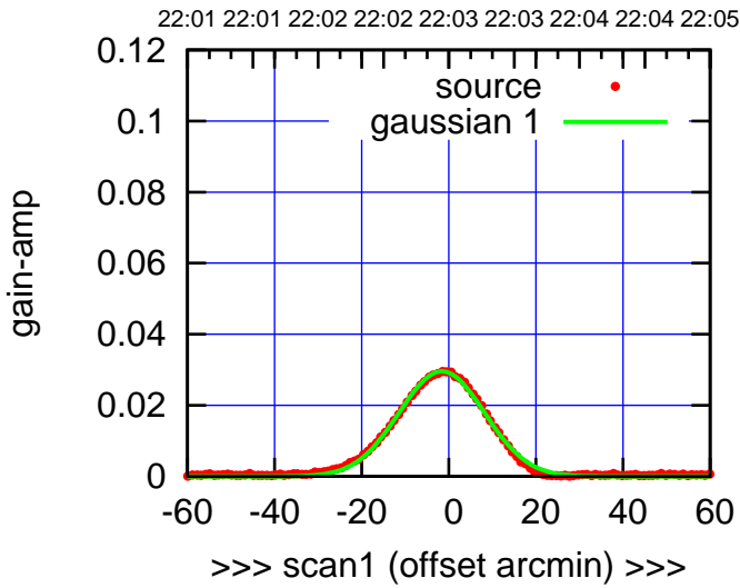
S04-130-EL OFF= -2.1' ( 23.3')
