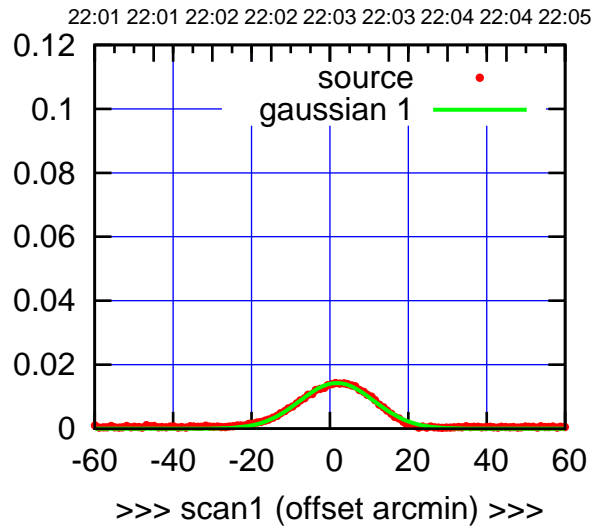
C10-175-EL OFF= 1.2' ( 22.8')
