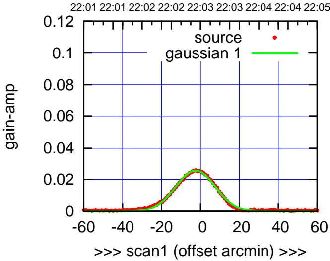
C14-130-EL OFF= -0.1' ( 24.2')
