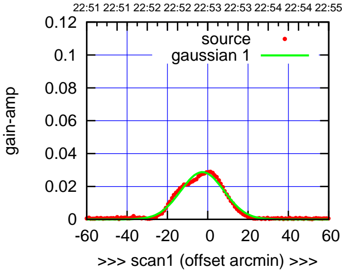
C00-130-AZ OFF= -2.9' ( 20.1')
