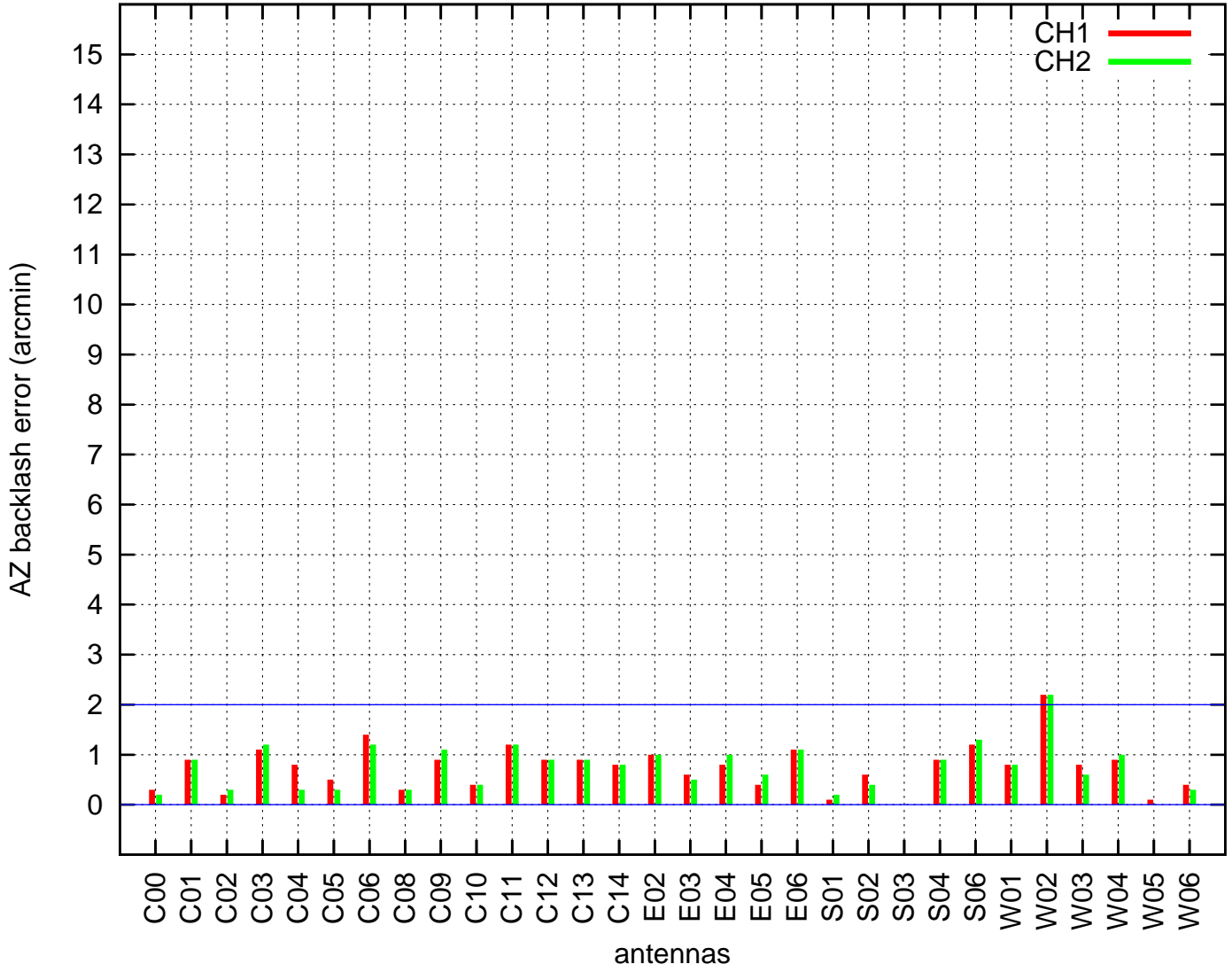
AZ backlash test (25Jul2018 22:53:00)
