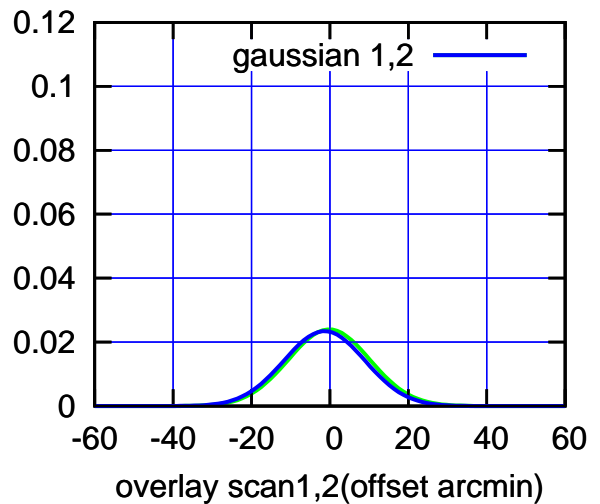
BACKLASH ERROR= 1.3'
