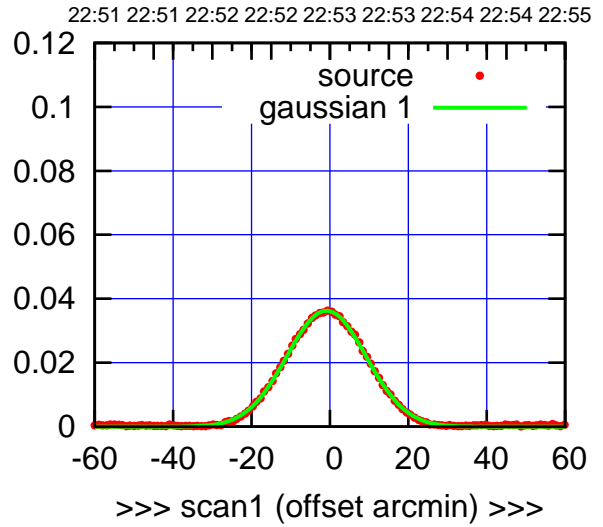
W05-175-AZ OFF= -0.9' ( 24.0')
