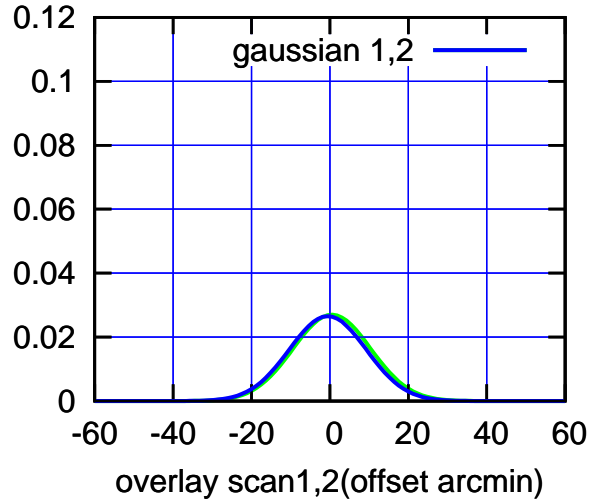
BACKLASH ERROR= 1.2'
