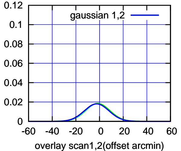
BACKLASH ERROR= 1.0'
