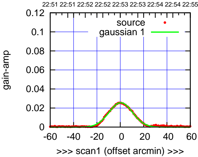
C12-130-AZ OFF= -0.4' ( 22.7')
