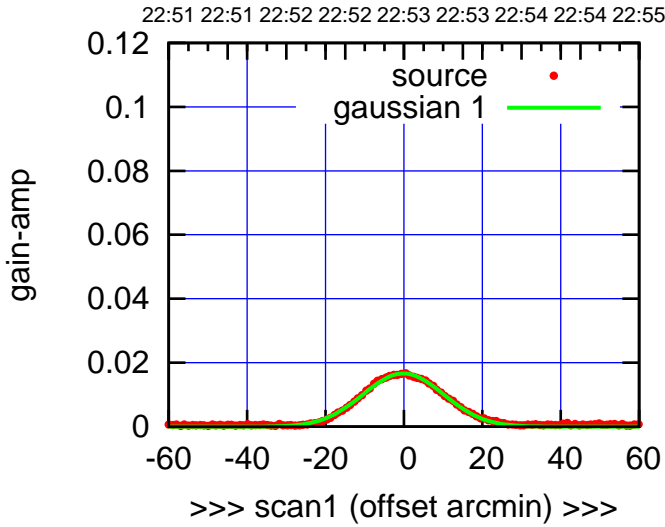
C10-130-AZ OFF= -0.5' ( 24.9')
