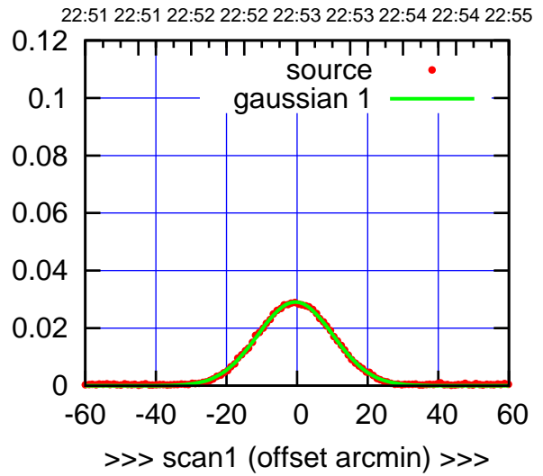
S02-175-AZ OFF= -0.9' ( 24.9')
