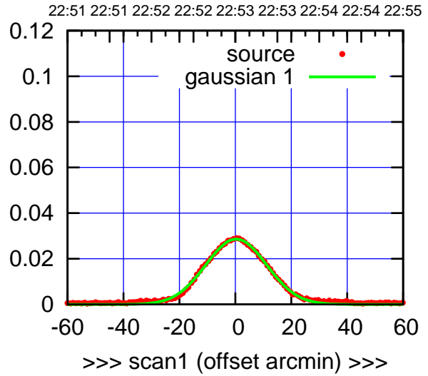
C12-175-AZ OFF= -0.5' ( 24.6')
