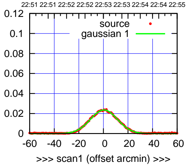
E03-175-AZ OFF= -0.1' ( 25.3')
