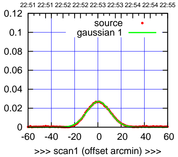
C11-175-AZ OFF= -0.6' ( 23.2')
