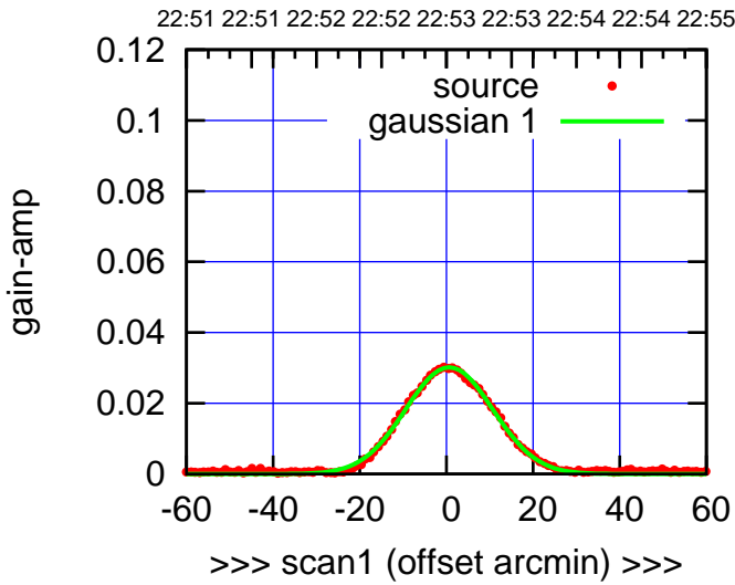
C11-130-AZ OFF= -0.4' ( 23.4')
