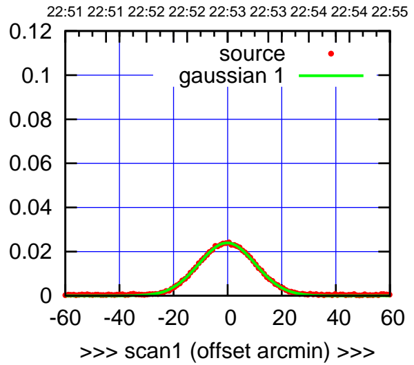
S06-175-AZ OFF= -1.4' ( 24.4')
