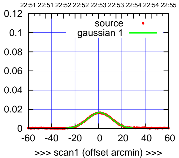
W06-175-AZ OFF= 0.7' ( 24.5')
