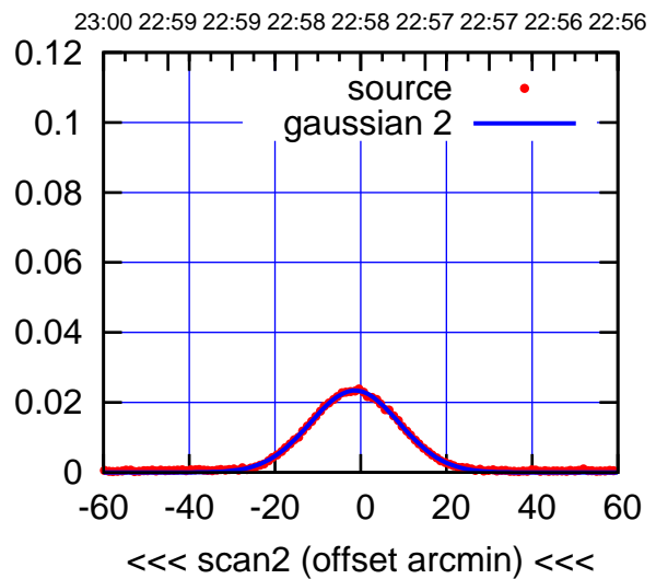
BACKLASH ERROR= 1.3'
