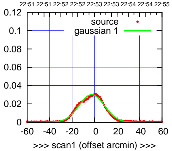
C00-175-AZ OFF= -2.8' ( 21.7')
