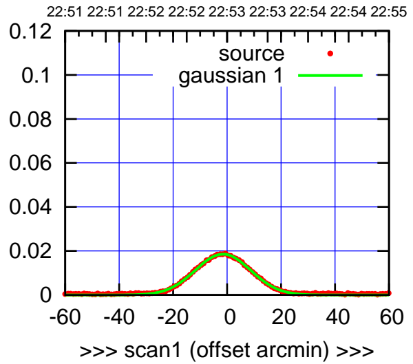
E02-175-AZ OFF= -2.4' ( 24.3')
