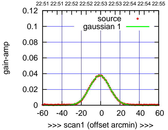
W03-175-AZ OFF= -1.6' ( 24.1')
