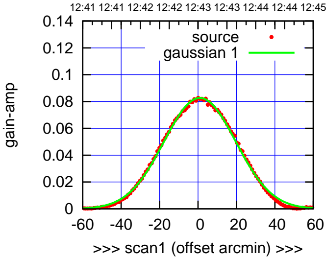
W05-130-EL OFF= 4.7'
