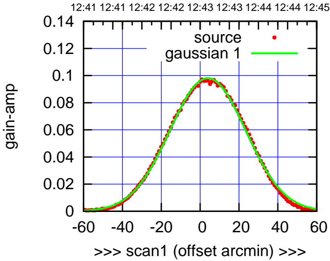
S03-130-EL OFF= 3.3'
