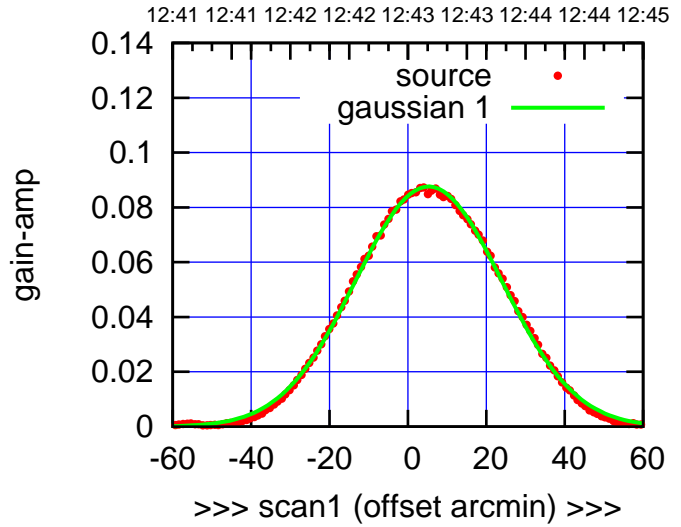
C04-175-EL OFF= 5.3'
