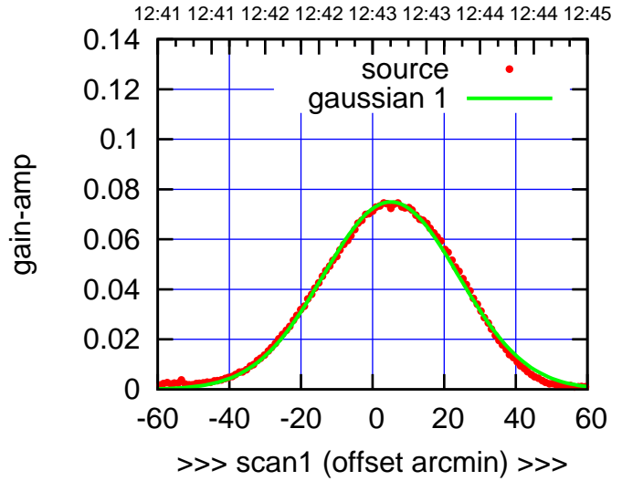
C05-175-EL OFF= 4.4'
