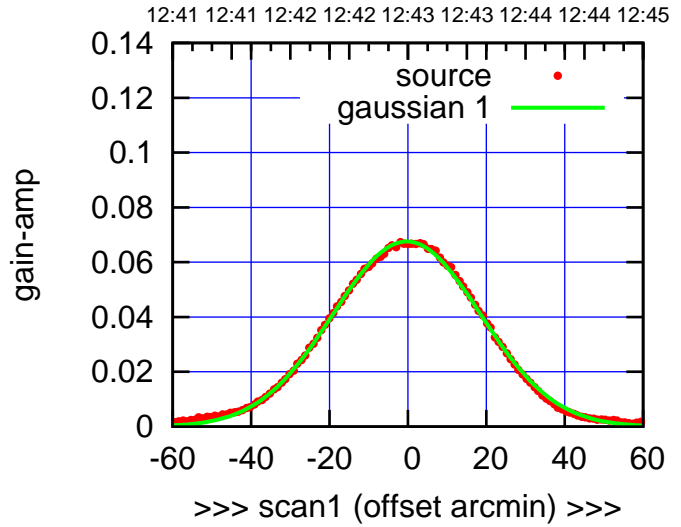
C03-175-EL OFF= -0.6'
