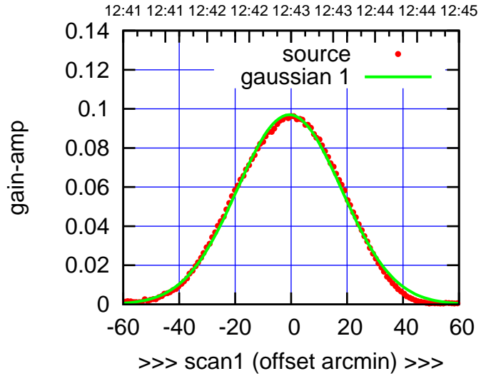
C02-175-EL OFF= 0.4'
