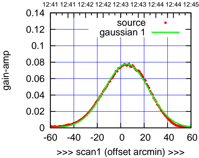
C05-130-EL OFF= 4.3'
