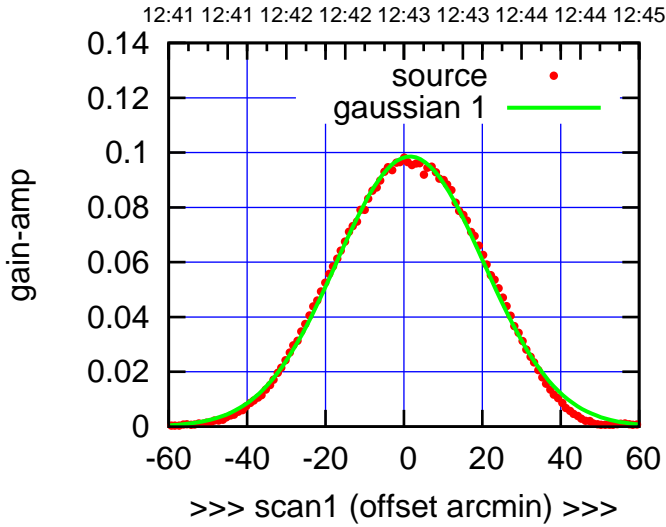
E04-130-EL OFF= 2.5'
