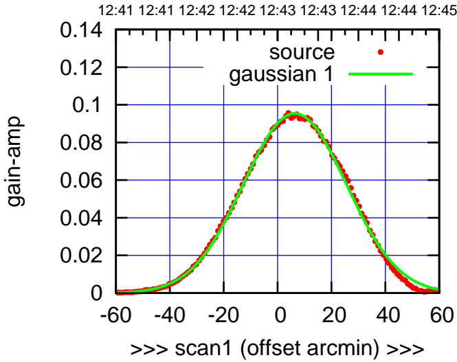
W02-130-EL OFF= 6.6'
