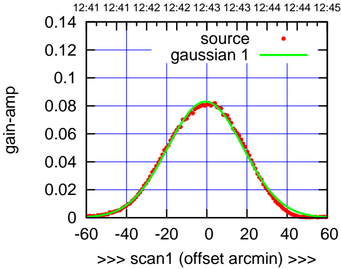
C02-130-EL OFF= 0.3'
