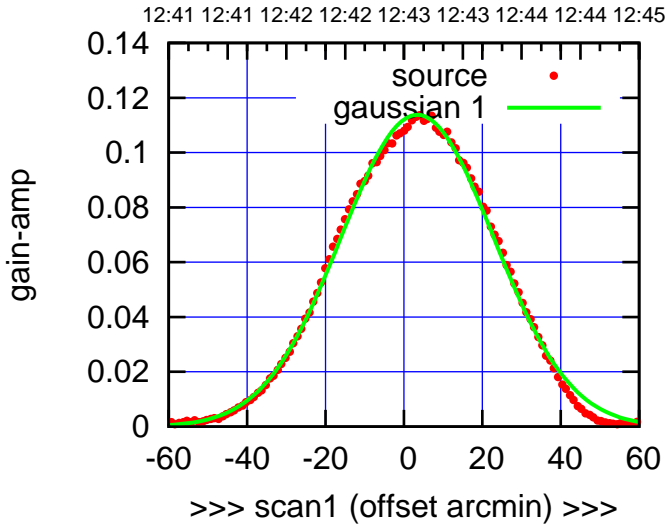
C10-130-EL OFF= 4.7'
