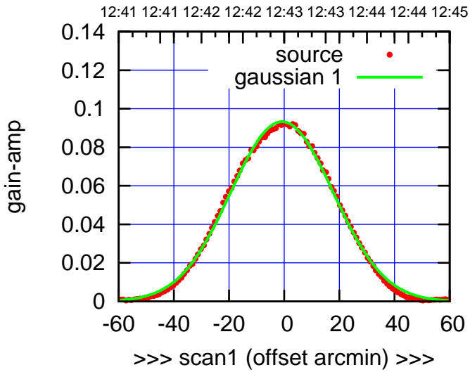
W03-130-EL OFF= 0.6'
