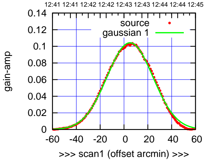
C13-175-EL OFF= 5.3'
