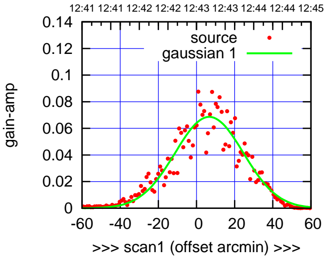
C14-130-EL OFF= 7.0'
