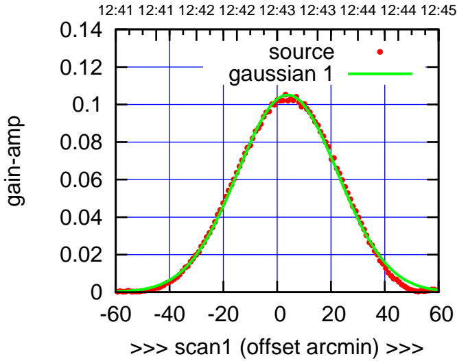
S02-130-EL OFF= 7.6'
