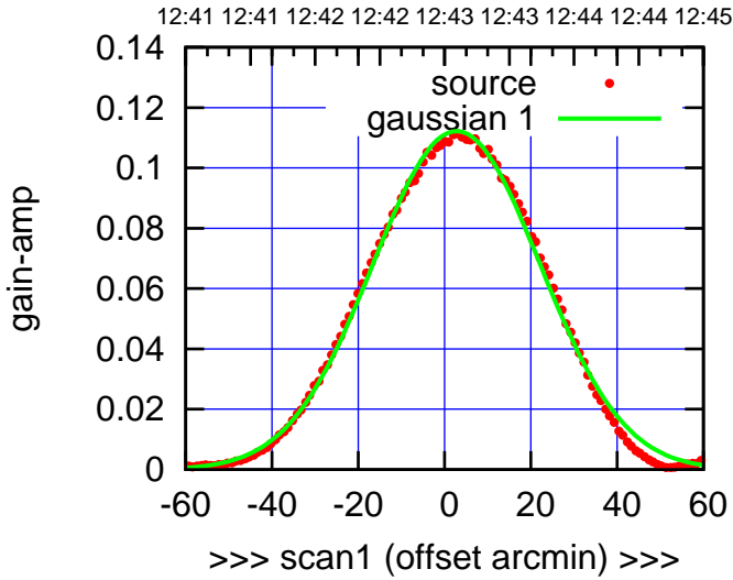
W01-130-EL OFF= 3.7'
