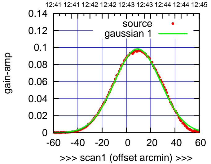
E05-175-EL OFF= 9.5'
