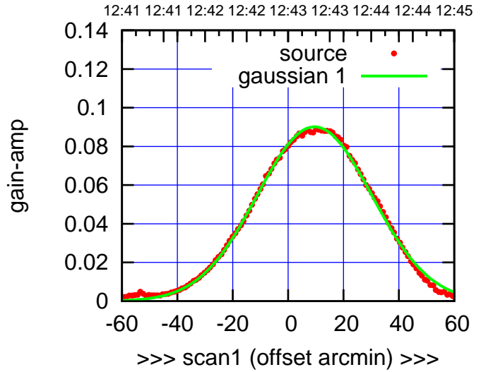
C06-175-EL OFF= 8.9'
