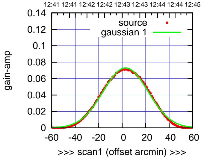
S04-175-EL OFF= 11.5'
