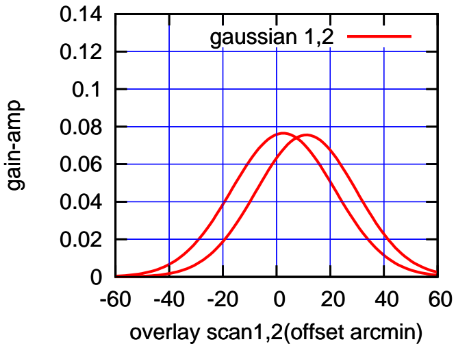
BACKLASH ERROR= 8.6'
