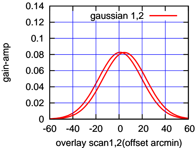
BACKLASH ERROR= 3.7'
