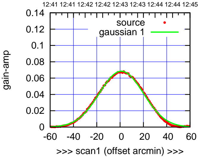
S06-130-EL OFF= 2.2'
