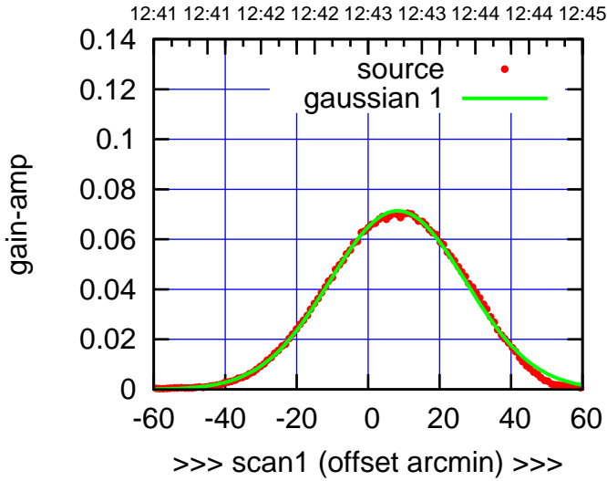
E05-130-EL OFF= 8.6'
